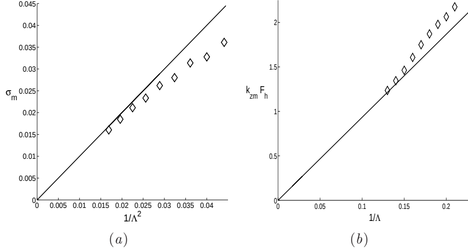
FIG. 4.6 – Comparison of (a) the maximum growth rate against 1/\Lambda^2 and (b) of the most amplified wavenumber against 1/\Lambda obtained numerically (diamonds) for F_h = 1 and Re = 16000 and asymptotically (plain line).
