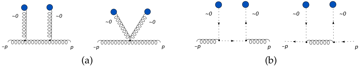
Figure 3.1: (a) Contribution of the gluon A^2 -condensate (represented as soft external gluons) to the gluon two-point function (b) Contribution of the ghost \bar{c}c condensate (represented as soft external ghosts) to the gluon and ghost two-point functions. These contributions vanish because they are proportional to ( \sim zero) momentum of the outgoing ghost is the ghost-gluon vertex.
