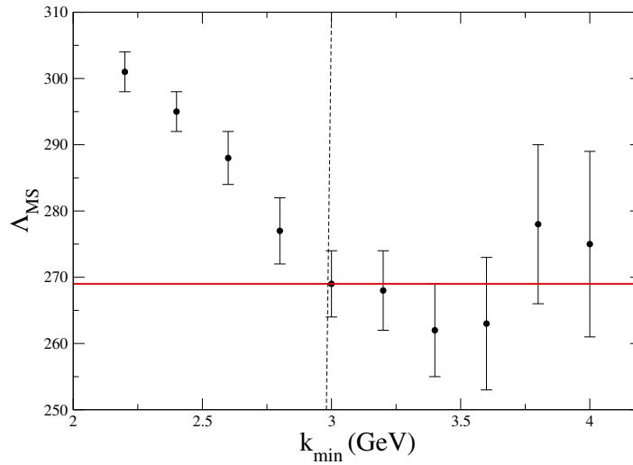
Figure 3.8: The determination of the optimal window fit (from 3 GeV to k_{\max} a \leq \pi/2 ) results from the search for some “plateau” of \Lambda_{\overline{MS}} when one changes the low bound of the fit window. Fits are done in the \widetilde{MOM} scheme.
