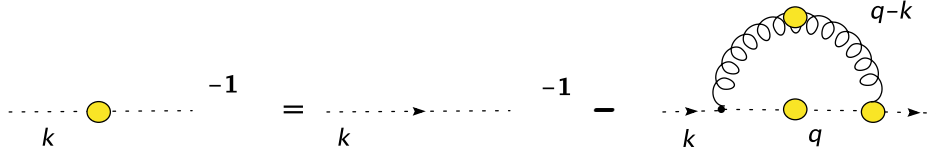
Figure 1.3: Schwinger-Dyson equation for the ghost propagator in a pure gauge theory, diagrammatically.
