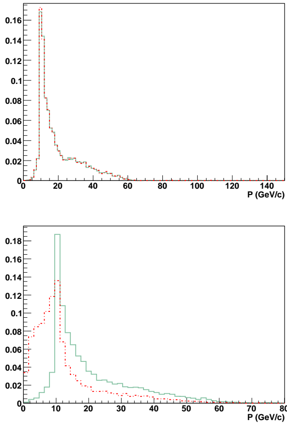
Figure 5.19: Comparison between the track momentum at the vertex (green, solid histogram) and at the outermost hit (red, dashed-dotted) for 10 GeV/c p_T electrons. Top) E_{\gamma} tracks: the two distributions are very similar. Bottom) GSF tracks: a large difference is visible.
