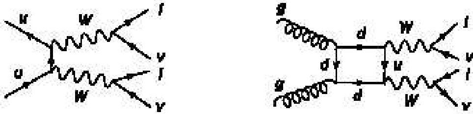
Figure 6.2: Tree level diagrams for the q\bar{q} \rightarrow WW^{(*)} and the gg \rightarrow WW^{(*)} processes with two charged leptons and two neutrinos in the final state.
