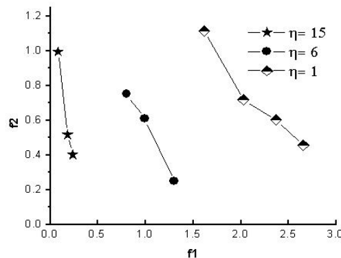
Figure 4.5 Influence of the distribution index \eta of SBX crossover on the results (results of 12 runs). Higher value of distribution index \eta seems more efficient for foothill inversion.
