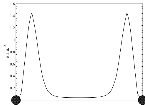
Figure 12.13: LDA density cuts in e \text{ a.u.}^{-3} along a line between two neighboring copper atoms. The large dark circles represent copper atoms.
