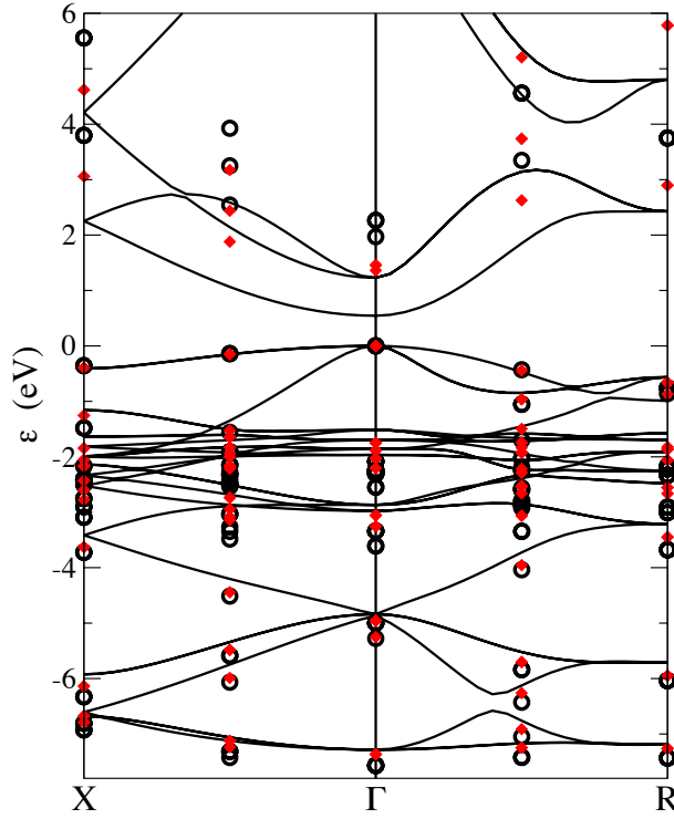
Figure 14.3: Band structure of \text{Cu}_2\text{O} within LDA (solid line) and one shoot GW (closed diamonds) given as a reference and within self-consistent GW (open circles) along X- \Gamma -R direction.
