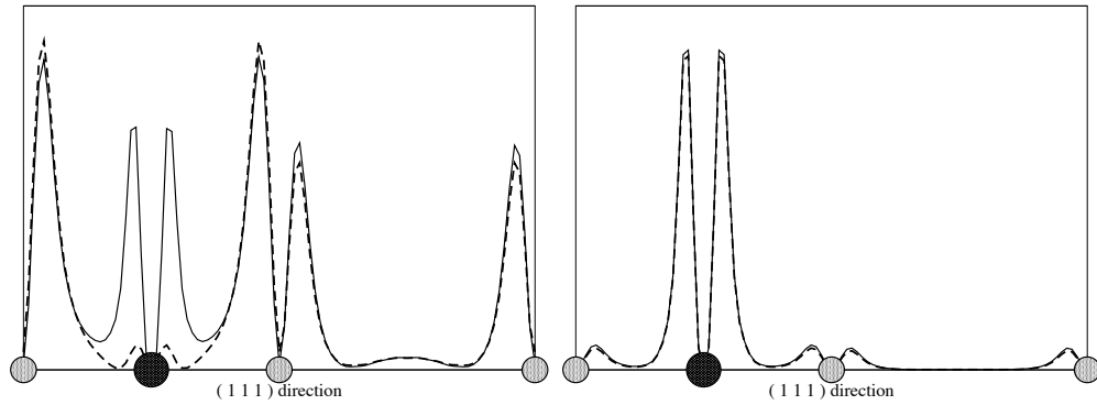
Figure 14.5: Squared modulus of the valence band number 30 wavefunction (Cu 3d region) (left panel) and sum of all squared moduli of Cu 3d valence wavefunctions (right panel) at \mathbf{k} -point (1/4, 1/4, 0) in \text{Cu}_2\text{O} along (1\ 1\ 1) direction. The small light grey circles symbolize the oxygen atoms. The large dark grey circle symbolizes the copper atom. The wavefunctions within LDA are displayed with the dashed line, the wavefunctions within GW with the solid line.
