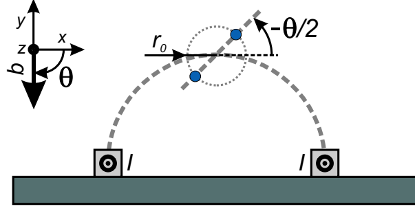
Figure 4.4: Tilting the double well: a small magnetic field \mathbf{b} splits the double to a radius r_0 = \sqrt{A/b} , rotating this field by \theta rotates the double well by -\theta/2 . A field \mathbf{b} orthogonal to the chip surface rotates the double well to 45^\circ which allows for horizontal splitting, when the chip is mounted under the same angle as in the Orsay setup.
