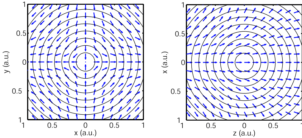
Figure 7.1: Normalized field vectors and equipotential lines of an isotropic Ioffe-Pritchard trap in the (x, y, 0) plane (left) and the (x, 0, z) plane (right).
