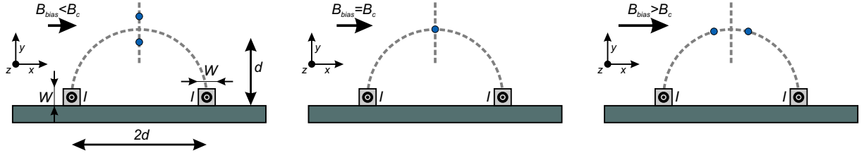
Figure 4.3: Schematic representation of the two wire beamsplitter/double well scheme proposed by [96]: for a small external bias field, two trap minima form an a vertical line (left). They merge at the coalescence point located at a distance d from the surface for B_{\text{bias}} = B_c (center) and horizontally split for larger bias field (right).
