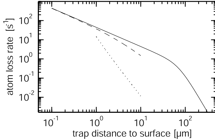
Figure 3.6: Atom loss rate due to thermally excited current in the atom chip. The solid line indicates the loss rate for a gold half space. The dotted line corresponds to a thin gold layer of 5\mu\text{m} , the dotted line is for a square cross section gold wire of 700\text{ nm} width. The atoms are assumed at rest at the bottom of a magnetic trap of B_0 = 1\text{ G} .
