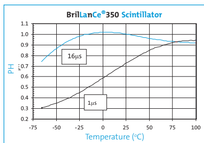
Figure 3. Temperature response
