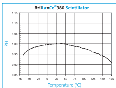
Figure 3. Temperature response. (The curve is for 12\mu\text{s} . The curve for 1\mu\text{s} is identical.)
