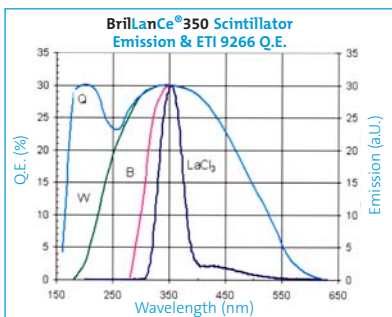
Figure 2. Scintillation emission spectrum of the BrillanCe®350 crystal and Quantum Efficiency of a bi-alkali ETI9266 PMT with (B) Borosilicate, (W) UV glass, and (Q) Quartz face plates (Q.E. data courtesy of Electron Tubes, Inc.)
