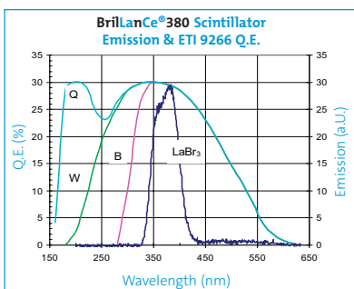
Figure 2. Scintillation emission spectrum of the BrilLanCe380 crystal and Quantum Efficiency of a bialkali ETI9266 PMT with (B) Borosilicate, (W) UV glass, and (Q) Quartz face plates (Q.E. data courtesy of Electron Tubes, Inc.)
