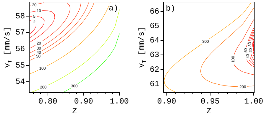
Figure D.3: Two \chi^2 - maps for TOFs of clouds with fugacities, a ) much smaller and, b ) much bigger than one. Clearly, in both graph, the real \chi^2 minima falls out of the shown maps . For the first case, however, this is just because the map was computed for values bigger than Z = 0.75 . An eye guided extrapolation of the ellipses for the region Z < 0.75 makes us almost guess what should be the fugacity. This is not case in the right hand side where the ellipses are too much deformed close to Z = 1 .
