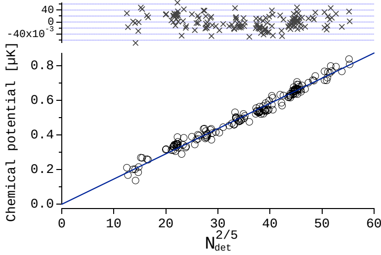
Figure B.2: Chemical potential for the pure condensates (see text) plotted in function of the number of detected atoms to the power of 2/5 . The curve is very well fitted by a straight line, which passes at zero even if no constraints are imposed in the fit. In the upper part of graph we also present the residuals of the fit: there is no tendency for the data to deviate from the linear fit. This result is compatible with a ballistic free expansion of the condensate. This could not be the case if it existed a lens effect due to the cloud of polarized atoms in the magnetic sub-level m_J = 1 (see also the text).
