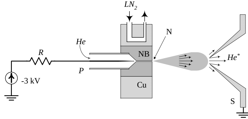
Figure 1.10: The \text{He}^* source setup. Helium in its fundamental state and at a pressure of several bars undergoes a relaxation between a nozzle (N) with a tiny diameter of 0.25 mm and length of 1 cm and a skimmer (S) located approximately 2.5 cm further and with a diameter of 1 mm. An electric discharge of -3 kV, established between the pin P and the grounded skimmer, produces some metastable helium atoms (the resistance R stabilizes the discharge at an operating current of about 13 mA). The efficiency of the process is of only 10^{-4} and, starting from a total helium flow of 5 \times 10^{15} at/s, the metastable jet flux is around 10^{12} at/s. The nozzle is manufactured out of boron nitride (electrical insulator but good thermal conductor), assembled inside a block of copper through which circulates liquid nitrogen at 77 K. The jet longitudinal velocity is of about 1200 m/s with a divergence around 40 mrad. At the level of the skimmer, the collisions between atoms become negligible and the atomic jet is supersonic[73].
