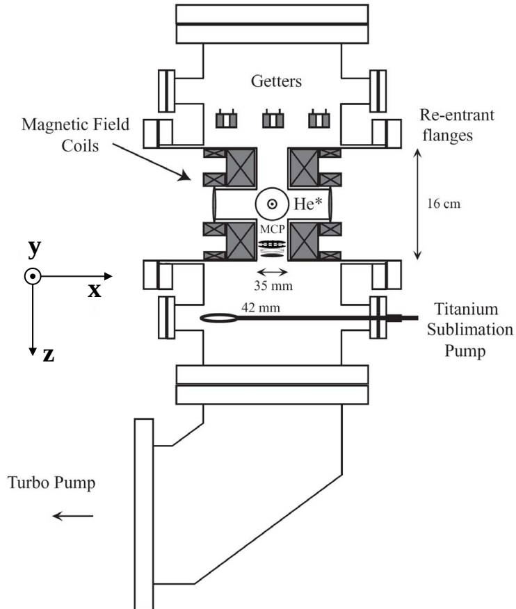
Figure 1.8: The ultra-high vacuum science chamber (UHV-Ch), where \text{He}^* condensation takes place. To help preserving the vacuum conditions, the magnetic field coils (dark gray in the Figure) are assembled outside the chamber in re-entrant flanges, as shown in the Figure. This allows positioning the coils closer together, increasing the trapping field gradients. As before, gravity acts in the Oz direction. See further details in §1.2.3.
