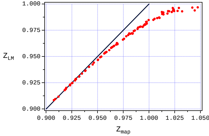
Figure D.2: Comparison between the values found by a LM routine and the \chi^2 - map 's method for the fugacity of several TOFs of clouds close to the critical phase transition. This graphs shows a tendency to the LM routine to return a value for Z slightly smaller than the one obtained with the \chi^2 - maps .
