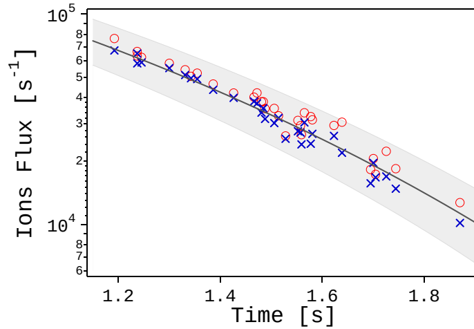
Figure 4.11: Same as in the preceding Figure but for fewer critical points , represented for both hyperbola-based (crosses) and the slope-break (circles) methods. The shadowed region corresponds, as before, to the \pm 25 kHz region around the critical curve .
