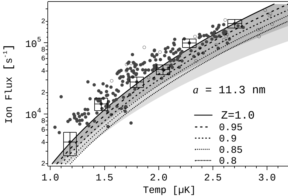
Figure 5.7: Similar graph as in Fig.5.5 with the ion flux in a log scale. The solid line is a theoretical curve for Z = 1 and a = 11.3 \text{ nm} . Boxes indicate typical error for the temperature (from the fit) and the critical ion flux. Dispersed points plotted in the right hand side of the Z = 1 line correspond to thermal cloud with Z < 1 . Shaded regions are computed using the results on Fig.4.6 and indicates dispersion regions for the entire bias fluctuation (lighter) or only half of it (darker). This latter seems to be sufficient to explain the data dispersion. The dashed and dotted lines correspond to theoretical curves for different Z . Those with Z = 0.95 and Z = 0.9 would limit the above dispersion regions if, disregarding the ion flux error, a proper value of the TOF 's fugacity is included in the determination of the temperature (see also text).
