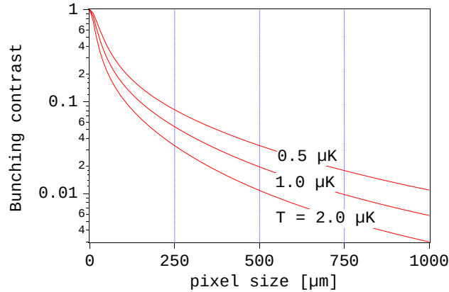
Figure 3.10: The bunching contrast in function of the pixel size, for three different temperatures.
