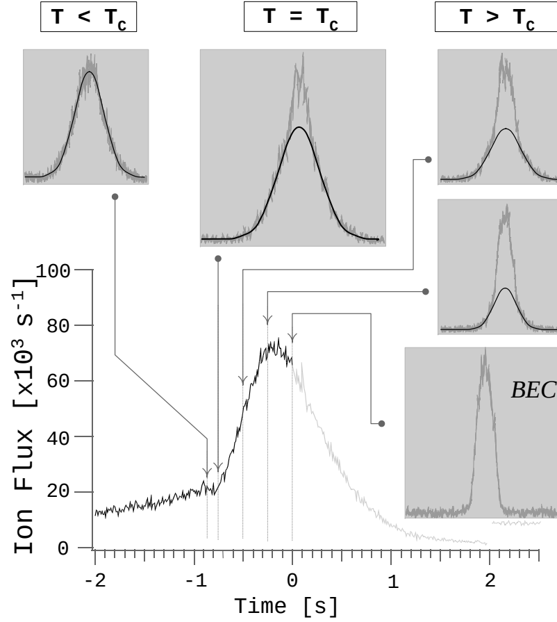
Figure 4.1: A single-shot measurement of the ions flux. The black part of the curve correspond to the last rf-ramp, where the rf -frequency ramps down from 1400 \text{ kHz} at t = -2 \text{ s} to 1000 \text{ kHz} when, at t = 0 , a pure BEC is formed. The five insets on this figure, represents typical TOF signals for some given time instants. Although these TOF curves does not correspond to the same experimental realization as the one shown in the main graph (recall that the TOF acquisition implies releasing the cloud and, consequently, interrupting the evaporative process) they were chosen among similar ions signal curves. In the column T \ll T_c , the presented TOF signal is well fitted by a Gaussian since its temperature is much higher than T_c . In the mid column a Gaussian is not sufficient to interpret the experimental curve, which starts to have a cusp shape at its center. The right hand side column represents different stages of the cloud in its evolution towards a BEC . The last frame corresponds to the pure BEC , characterized by an inverted parabolic shape (cf. A). The light gray curve in the ion signal, for t > 0 , corresponds to the evolution of the cloud after achieving BEC : the cloud start to heat with the decrease of its density and a consequent reduction of the ion flux signal.
