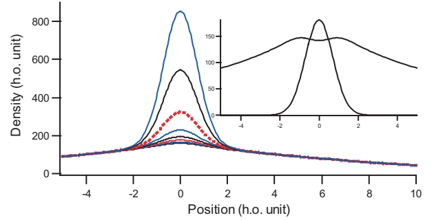
Fig. 6. Atomic density \rho_{ex} in function of r/\sigma where \sigma is the size of the harmonic oscillator ground-state. The temperature is T = 93.37\hbar\omega/k_B and the atom number N spans from 0.990 \times 10^6 to 1.004 \times 10^6 by step of 2000 atoms. The curve at threshold is in dotted line and corresponds to 10^6 atoms. The inset shows the excited states and ground state density profile at threshold. The dip around r = 0 is mainly due to the first excited state population.
