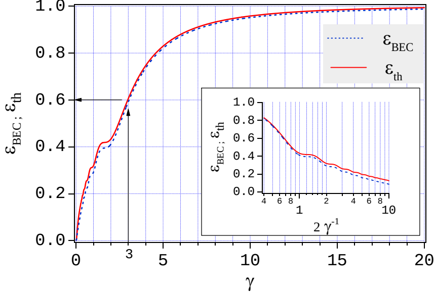
Figure 5.20: Dependence of \varepsilon_{\text{BEC}} and \varepsilon_{\text{th}} on the trapping potential relaxation constant \gamma . The inset graph shows the resonances that appears when the trapping relaxation time equals a semi-integer multiple of the time of an oscillation in the fast trapping axis.
