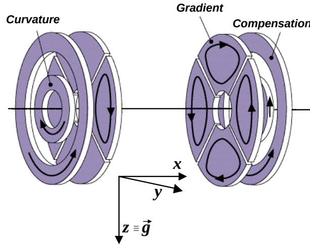
Figure 1.3: Clover-leaf magnetic trap schematic representation. The four inner coils, the gradient coils , create a gradient of the magnetic field in the transverse direction whereas the curvature coils are responsible for the axial confinement of the atoms. The compensation coils creates a magnetic field in the opposite direction of dipole field and are used to compress the trap (see also text). It is usual to refer to the axial direction as the bias field direction. The gravitational field direction coincides with the Oz direction. In our setup, the gradient coils are placed 44 mm apart (the shown Figure was taken from the Ketterle's group web site).
