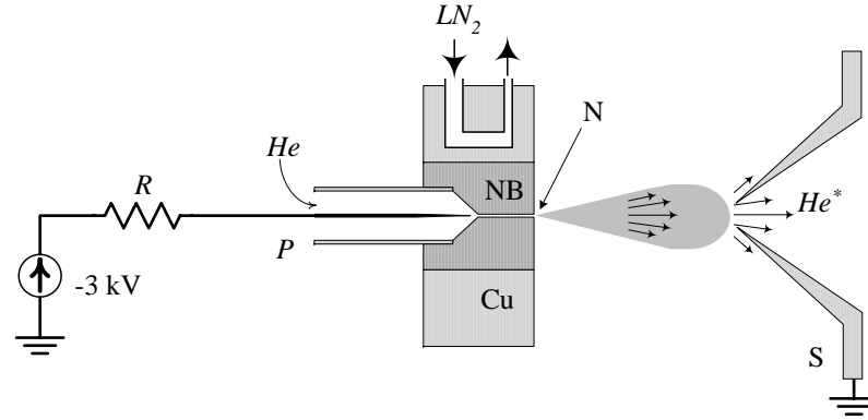
Figure 1.10: The \text{He}^* source setup. Helium in its fundamental state and at a pressure of several bars undergoes a relaxation between a nozzle ( N ) with a tiny diameter of 0.25 mm and length of 1 cm and a skimmer ( S ) located approximately 2.5 cm further and with a diameter of 1 mm. An electric discharge of -3 \text{ kV} , established between the pin P and the grounded skimmer, produces some metastable helium atoms (the resistance R stabilizes the discharge at an operating current of about 13 mA). The efficiency of the process is of only 10^{-4} and, starting from a total helium flow of 5 \times 10^{15} \text{ at/s} , the metastable jet flux is around 10^{12} \text{ at/s} . The nozzle is manufactured out of boron nitride (electrical insulator but good thermal conductor), assembled inside a block of copper through which circulates liquid nitrogen at 77 K. The jet longitudinal velocity is of about 1200 m/s with a divergence around 40 mrad. At the level of the skimmer, the collisions between atoms become negligible and the atomic jet is supersonic[73].
