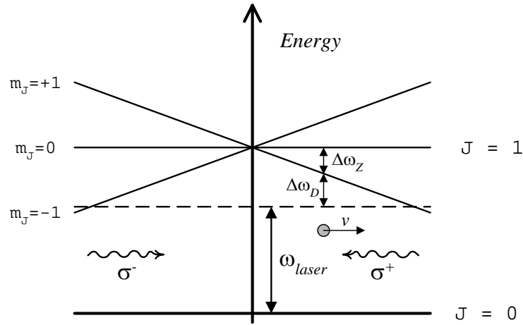
Figure 1.13: Working principle of a one dimensional Magneto-Optical trap (MOT) in a J = 0 to J = 1 atomic transition. Two contra-propagating laser beams, red detuned relatively to the atomic transition and polarizations \sigma^+ and \sigma^- are incident in a atomic cloud where a non-homogeneous magnetic field creates, from the center of the trap, a linear increase of the Zeeman shift of the atomic optic lines in that transition. The combination of the Doppler and of the Zeeman shifts makes fast out-coming atoms at the center of the trap to get in resonance with the laser and decelerate with the radiation pressure. This way, all the atoms with an initial velocity smaller than a critical capture velocity v_{cap} are confined at the center of the trap and cooled down. This critical velocity is proportional to the transverse size of region where the laser beams saturated the optical transition: the bigger this is, the bigger the number of optical cycles a given atom can make before escaping the trap
