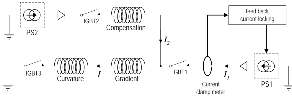
Figure 1.7: Electric circuit of the gradient, curvature and compensation coils, during the magnetic trap. Two power supplies, PS1 and PS2, are used to drive a current I_2 into the compensation coils and I = I_1 + I_2 into the gradient and the curvature coils, assembled in series. The high-bias field configuration ( B_0 = 190 G) is obtained closing the IGBTs 1 and 3, and adjusting PS1 so that I \equiv I_1 = 230 A. In the low-bias field case ( B_0 = 360 mG), all IGBTs are closed and the power supplies are adjusted as to deliver the currents I_1 = 10 A and I_2 = 220 A, keeping I = 230 A. In here, PS1 works in voltage control and a feed back locking circuit using a current clamp meter is used to stabilize I_1 (see also text). The bias field results from the difference between the fields produced by the compensation and gradient coils.
