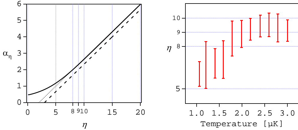
Figure 4.4: In the left hand side graph it is represented the dependence of \alpha_\eta in \eta . The dashed line corresponds to the value of \alpha_\eta obtained with the simple model presented in the beginning of this Section. The solid and dotted lines corresponds to the value of \alpha_\eta found with the model of Luiten et al. and an asymptotic approximation for this model respectively. In the right hand side graph, we plot experimental results obtained for \eta for different temperatures (see also the text). The error bars correspond to the standard deviations for many experimental runs.
