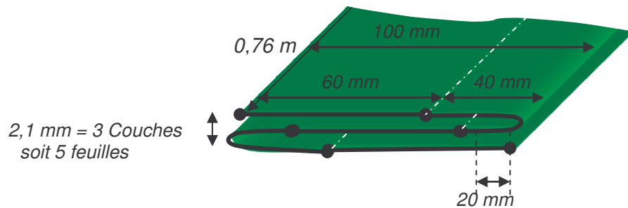
Figure III.6 : La disposition des bandes
