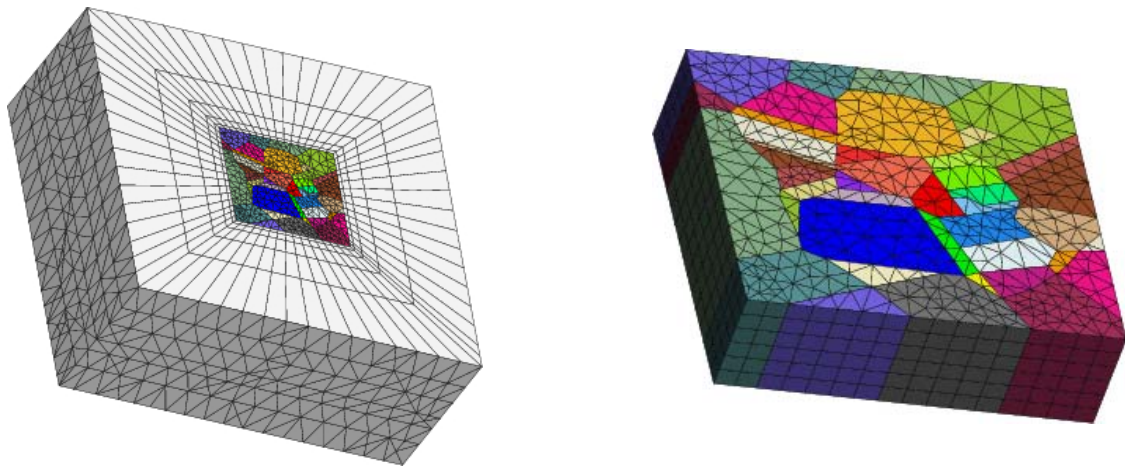
Figure VI.6 : "Modified small" and "extended small" finite element meshes
