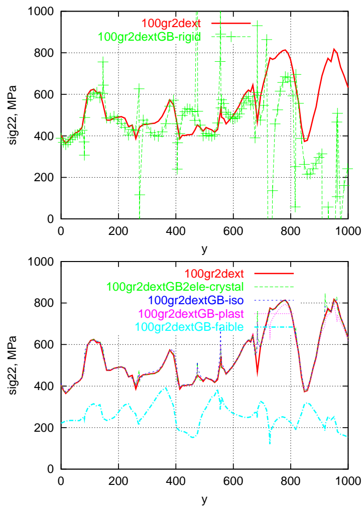
Figure VII.6 : sig22 dependence on Y coordinate for Y=0 line
