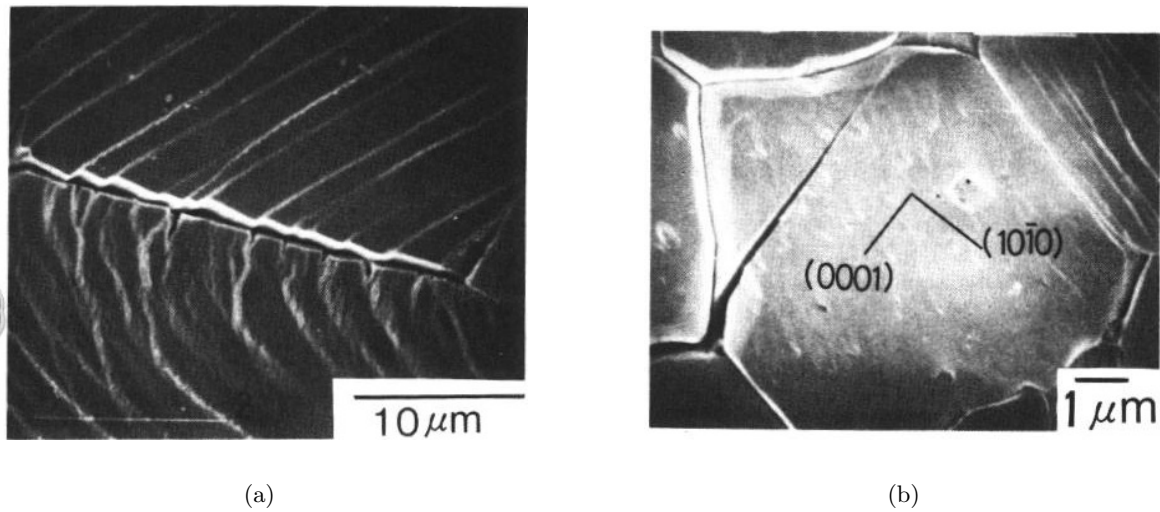
Figure II.5 : TG crack photos (Kubo et al., 1985) : (a) - Crack initiation, (b)- Crack propagation
