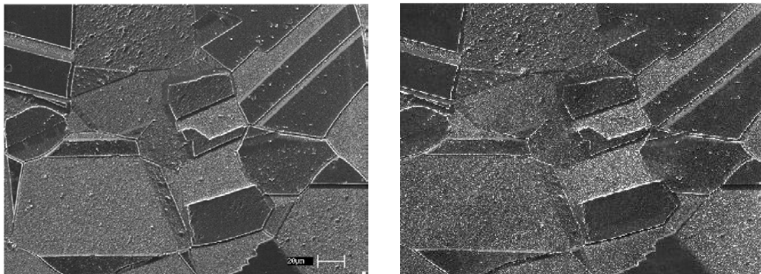
Figure VI.2 : SEM micrographs at 0% and 10% macrostrains
