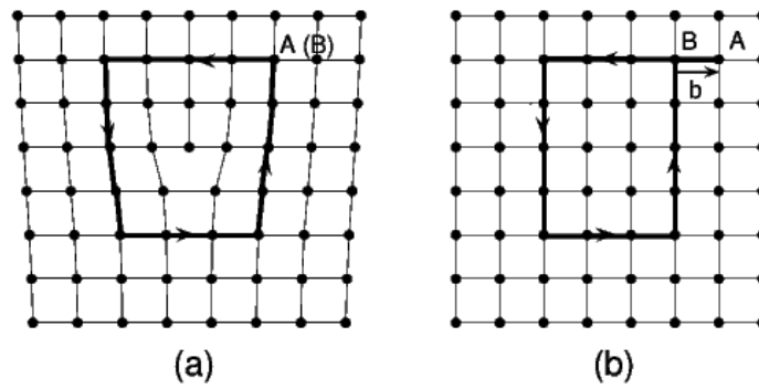
FIG. 1.4 – Circuit de Burgers
