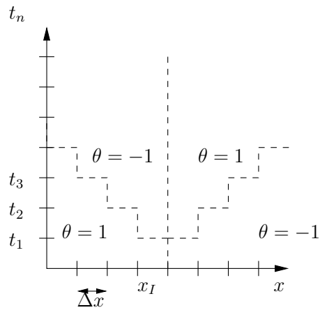
FIG. 6.3 – Evolution with the velocity c^n .
