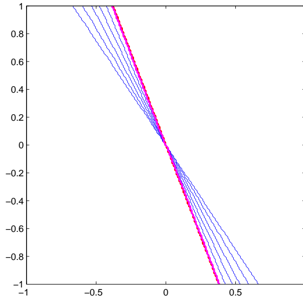
FIG. 6.15 – A rotating line
