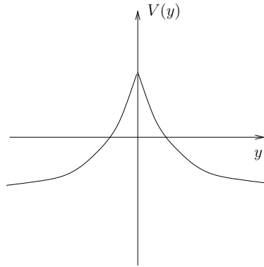
FIG. 8.2 – Typical profile for a potential V satisfying assumptions (H).
