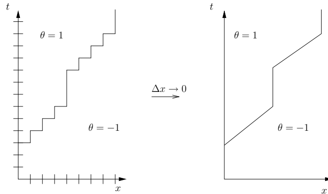
FIG. 6.10 – Correct evolution when the time is updated with t .
