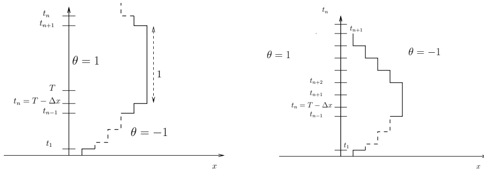
FIG. 6.7 – Front evolution without the threshold \Delta t FIG. 6.8 – Front evolution with the threshold \Delta t
