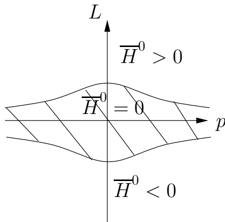
FIG. 8.1 – Schematic representation of the effective Hamiltonian
