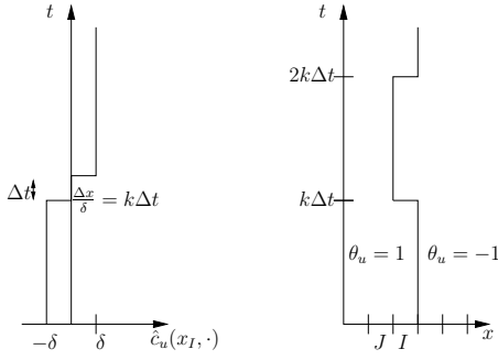
FIG. 6.11 – Velocity and evolution of the front for u .
