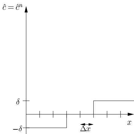
FIG. 6.4 – The velocity \hat{c}^n .
