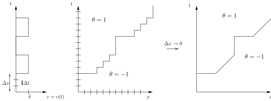
FIG. 6.9 – Wrong evolution when the time is updated with \hat{t} .
