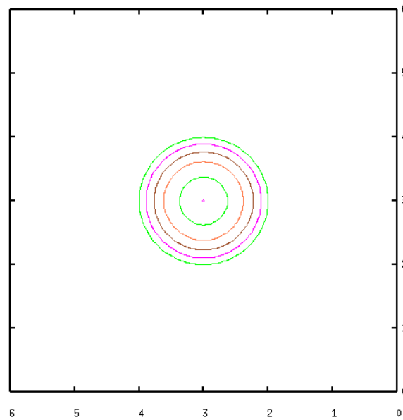
FIG. 5.2 – Evolution of a circle of radius 1 at time 0, 0.1, 0.2, 0.3, 0.4 and 0.49
