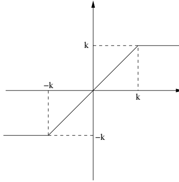
FIG. 2.2 – A truncature function T_k .
