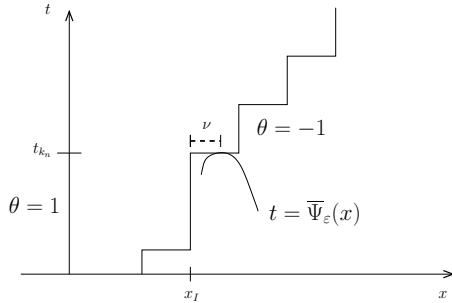
FIG. 6.13 – Test function from below FIG. 6.14 – Test function from above
