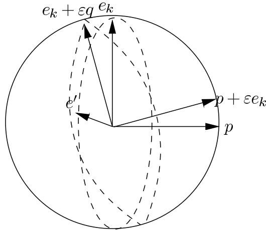
FIG. 4.1 – Computation at the first order of \partial_k A_{ij}(p) , case |p| = 1 .
