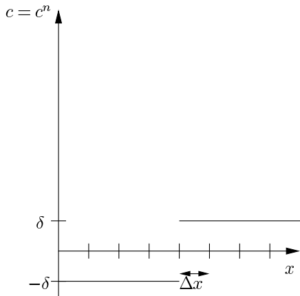
FIG. 6.2 – The velocity c^n .
