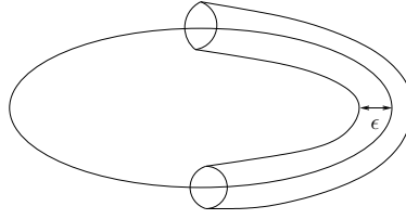
FIG. 2.1 – The cutoff tube of radius \epsilon .
