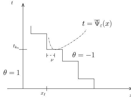
FIG. 6.13 – Test function from below FIG. 6.14 – Test function from above
