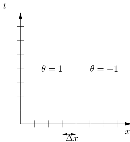
FIG. 6.5 – Evolution with the velocity \hat{c}^n .
