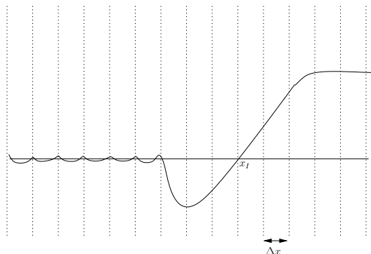
FIG. 5.1 – Graph of the function \varphi defined in \mathbb{R} .
