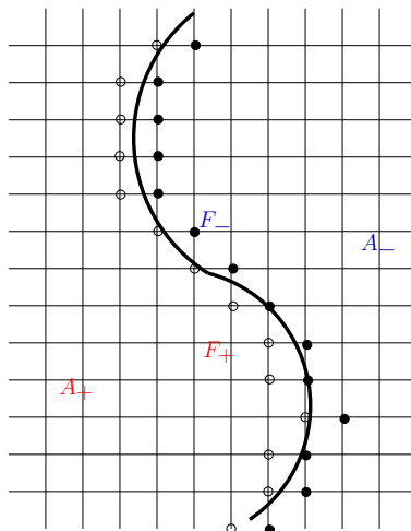
FIG. 6.1 – The narrow bands F_+ and F_- .
