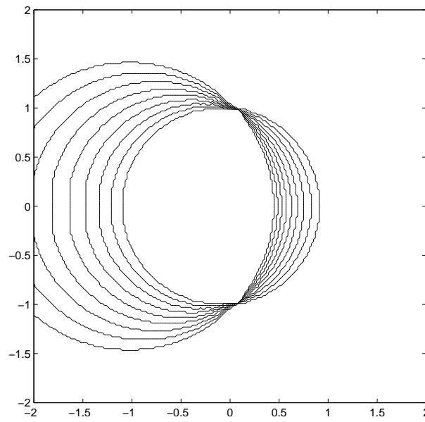
FIG. 6.16 – A propagating circle
