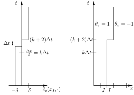
FIG. 6.12 – Velocity and evolution of the front for v .
