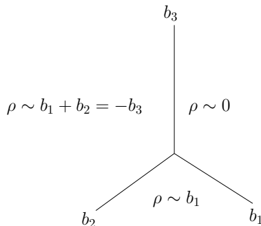
FIG. 7.1 – The junction of three dislocations as phase transitions of \rho .
