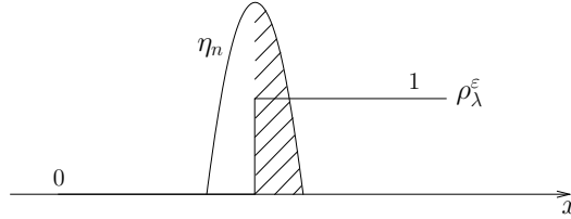
FIG. 4.2 – The convolution of \rho_\lambda^\varepsilon with the Dirac.
