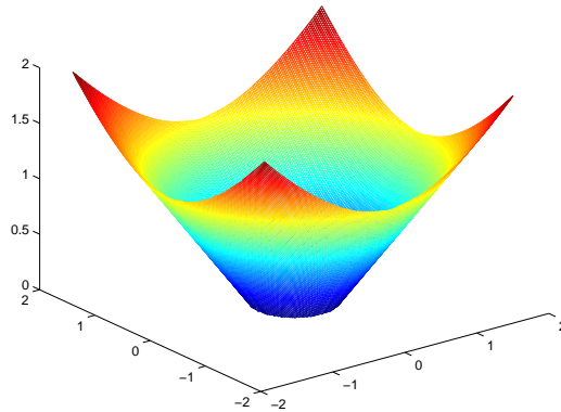
FIG. 6.17 – The discrete time u of a propagating circle with positive constant speed
