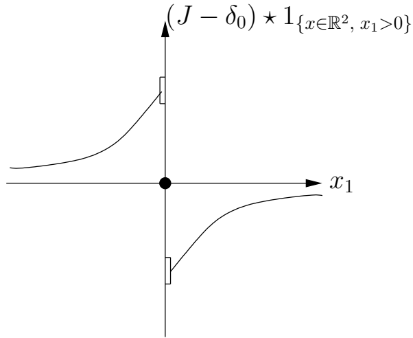
FIG. 8.3 – Typical profile for the Peach-Koeller force created by a dislocation straight line.
