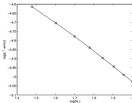
FIG. 9.3 – \log(L^\infty - \text{error}) of |u_{N_T} - u_{N_T-1}| versus \log(N_x) at T = \frac{1}{2}
