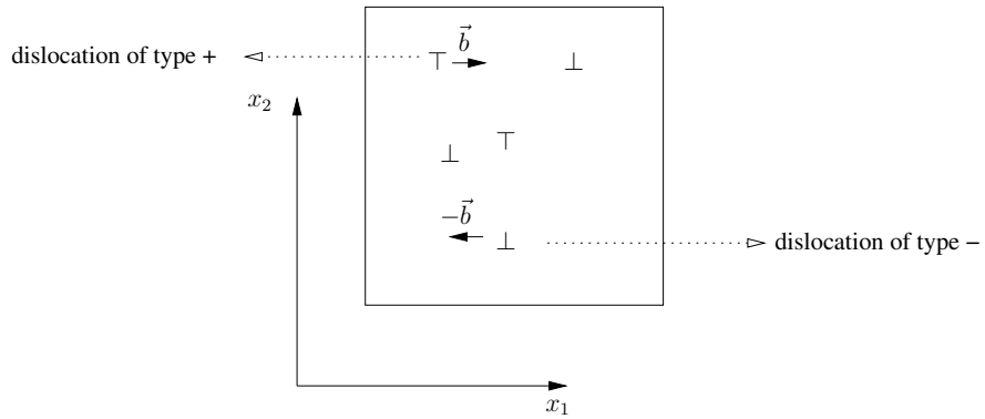
FIG. 9.1 – The cross-section of the dislocations lines.
