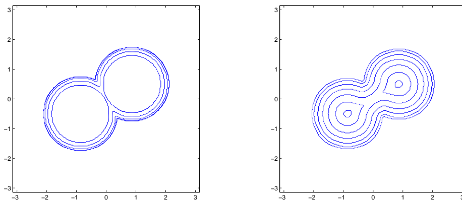
FIG. 6.18 – Two propagating circles
