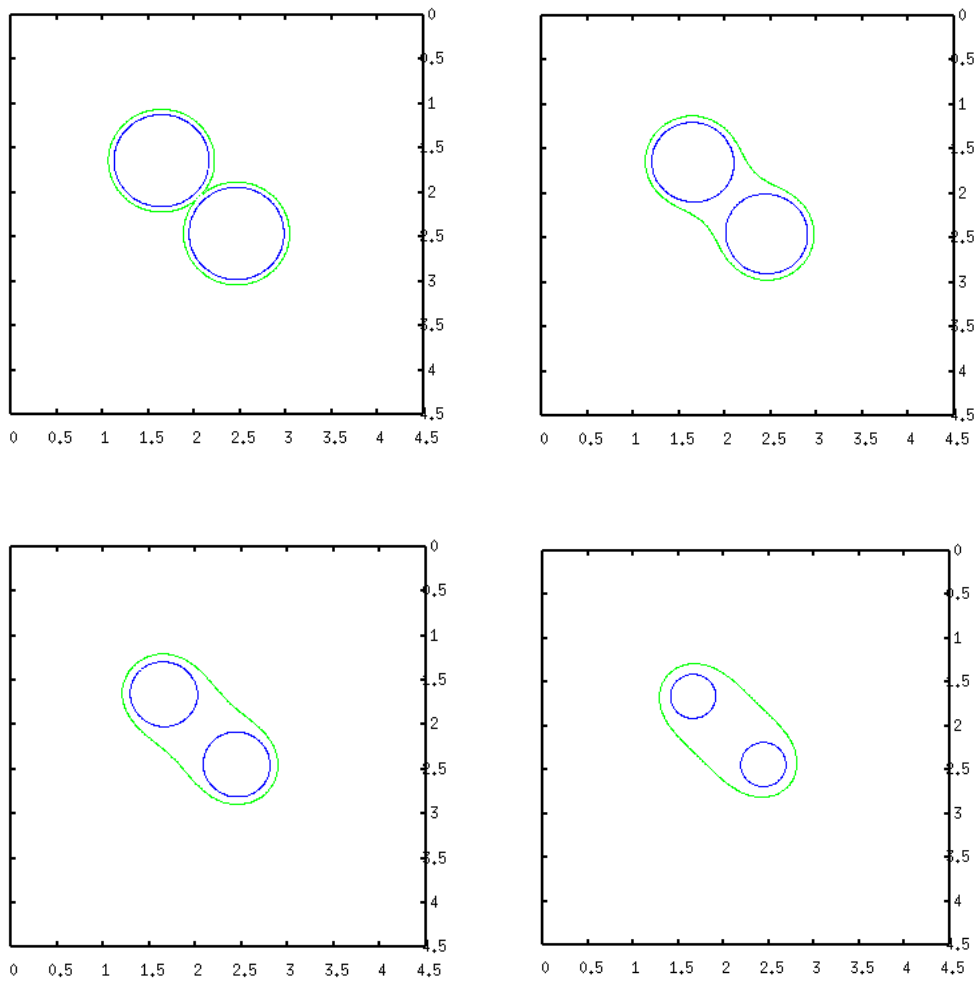
FIG. 5.3 – Evolution of the 8 at time 0, 0.05, 0.1 and 0.15.
