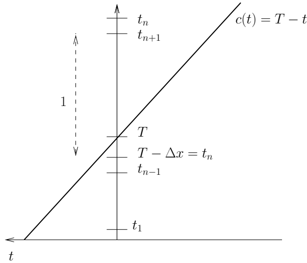
FIG. 6.6 – Jump in the discrete time without threshold \Delta t in the case of a linear in time velocity
