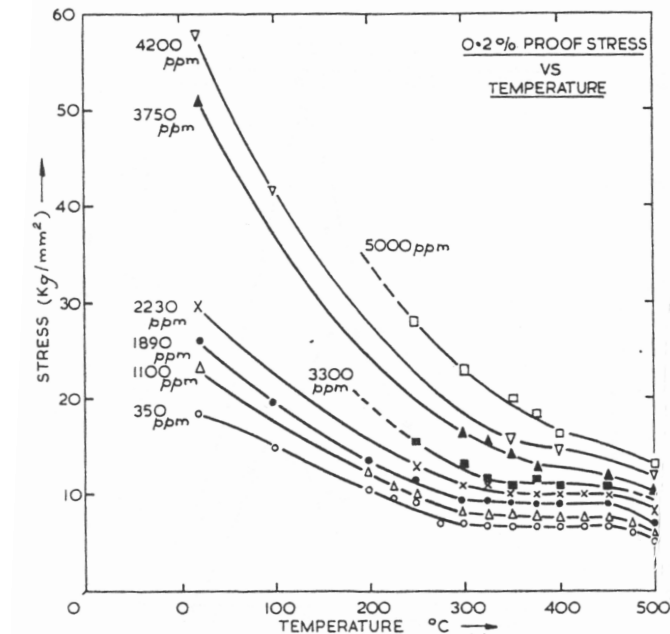
Figure IV.5 : Variation of yield stress with temperature for zirconium-oxygen alloys with different oxygen contents (Kelly and Smith, 1973).
