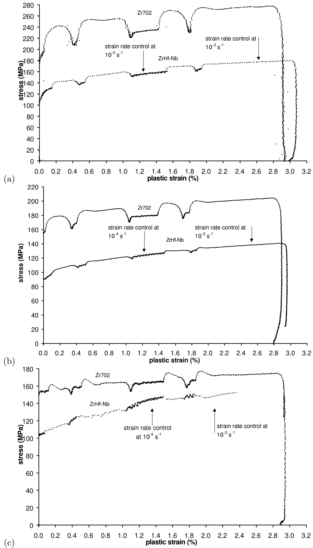
Figure II.5 : Influence of interstitial and substitutional atoms on the macroscopic true stress-plastic strain curves of the tensile tests with strain rate changes of Zr702 and ZrHf-Nb at : (a) 200^{\circ}\text{C} , (b) 300^{\circ}\text{C} , (c) 400^{\circ}\text{C} .
