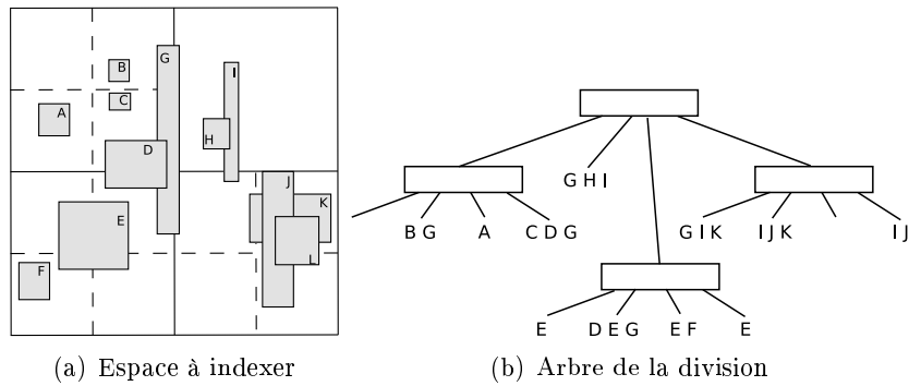
Figure 1.6 — Quadtree
