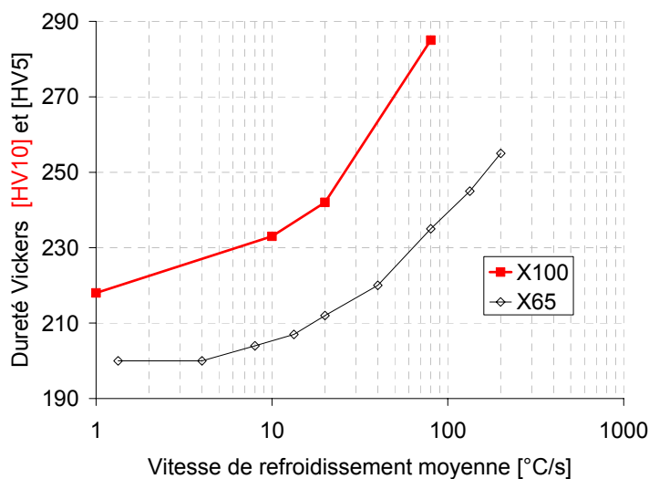
X100 : Duret  HV10, T_m = 1250  C / X65 : Duret  HV5, T_m = 1350  C [EP_TP_33]
