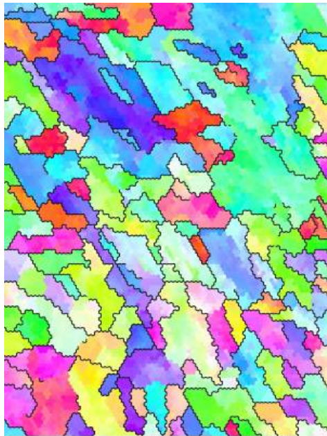
15.00 \mu\text{m} = 15 steps IPF [010] Boundary levels: 15°
