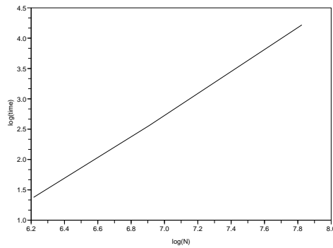
Figure 15.7: Evolution of \log(\text{time}) w.r.t \log(n)
