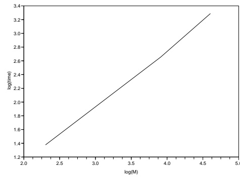
Figure 15.9: Evolution of \log(\text{time}) w.r.t \log(M)
