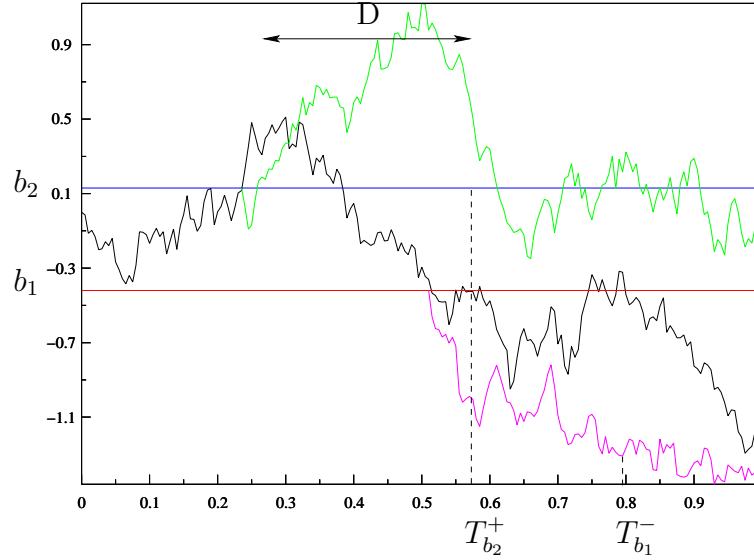
Figure 5.1: Brownian paths
