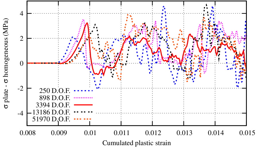
Figure VI.7 : Numerical global serrated stress minus homogeneous stress ( \frac{F}{S_0} - \sigma^{Homogeneous} ) for tensile plates at a constant strain rate of 10^{-4}s^{-1} . Simulations have been performed for five different meshes, for the same boundary value problem and material parameters.
