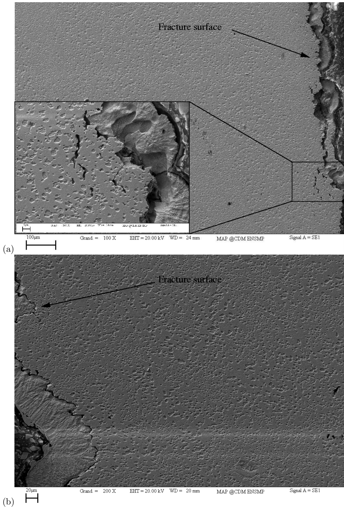
Figure III.13 : Longitudinal cross sections of fracture surfaces of (a) a smooth specimen (b) a notched specimen at room temperature for a prescribed strain rate of 10^{-3} s^{-1} .
