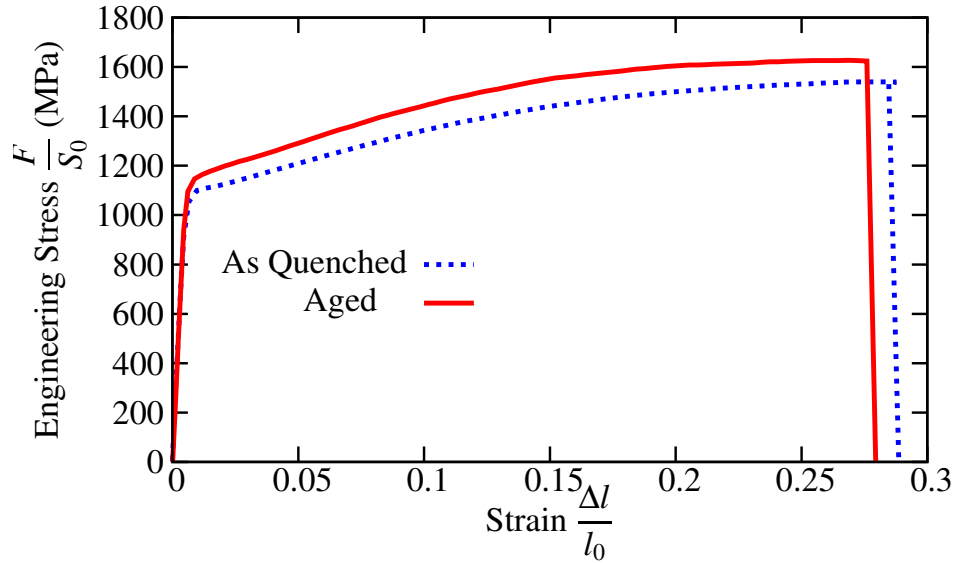
Figure III.6 : Tensile curve of axisymmetric smooth specimens in Udimet 720 at room temperature before and after ageing heat treatment for a prescribed strain rate of 10^{-3}\text{s}^{-1} .
