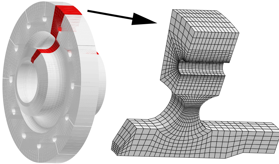
Figure IV.6 : S-Disk and B-Disk geometry and mesh
