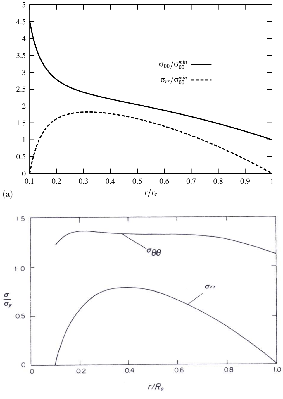
Figure IV.3 : Axisymmetrical stresses according to plane stress approximation for bored disks with r_i/r_o = 0.1 for (a) elastic behavior (Forest et al., 2006) (b) elastoplastic behavior (Tvergaard, 1978) ( r_i inner radius, r_o outer radius)
