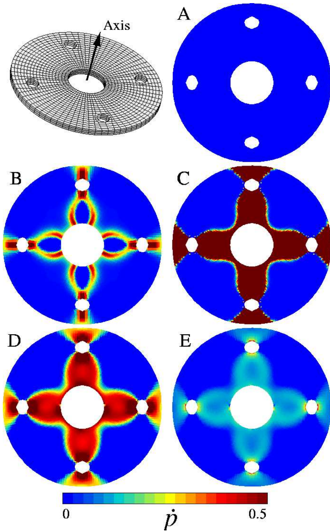
Figure VIII.6 : Maps of cumulated plastic strain rate corresponding to points A,B,C,D,E of figure VIII.5
