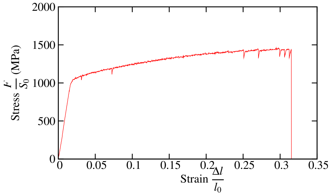
Figure III.16 : Tensile curve of axisymmetric smooth specimens in Udimet 720 at 500°C for a prescribed strain rate of 10^{-4} \text{ s}^{-1} .
