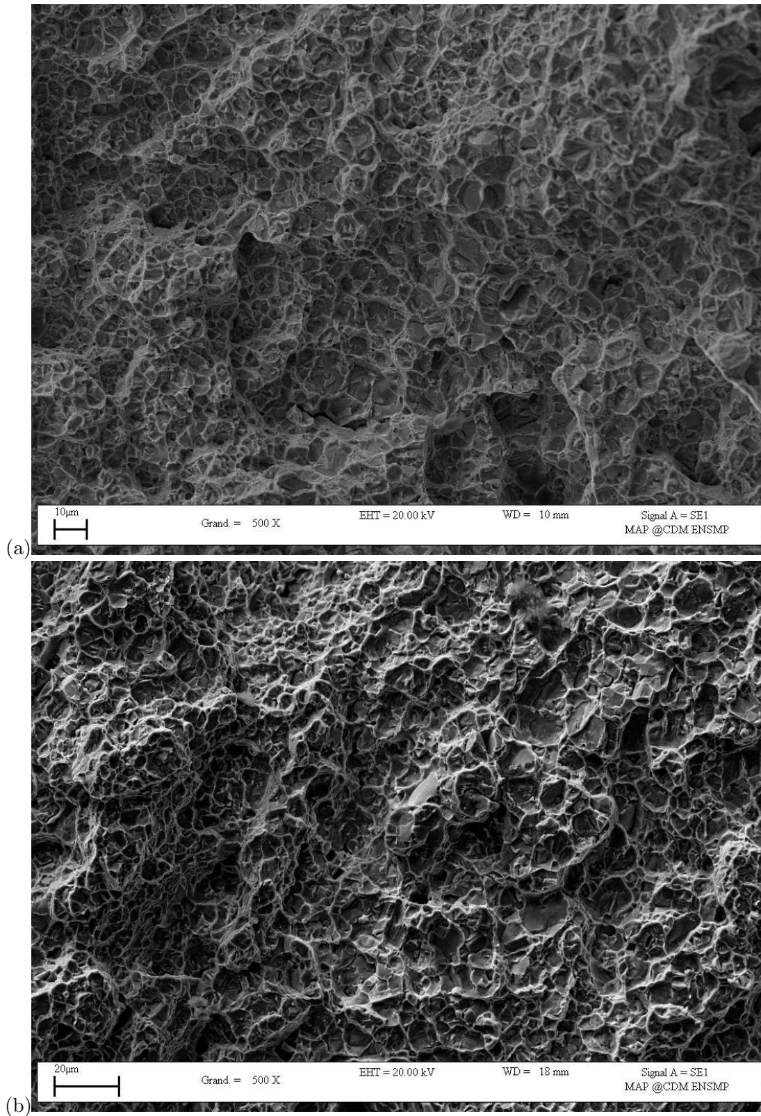
Figure III.12 : Fracture surfaces of (a) a smooth specimen (b) a notched specimen at room temperature for a prescribed strain rate of 10^{-3} s^{-1} .
