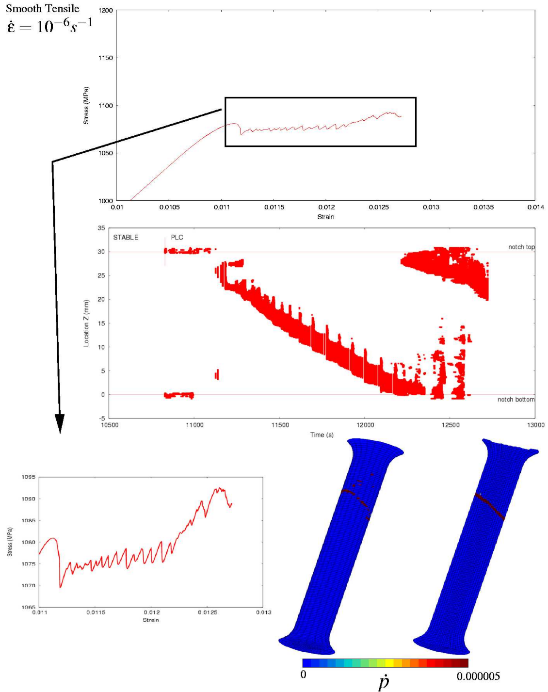
Figure VII.10 : Global stress/strain curve, location of bands as a function of time, zoom on serrations and plastic strain rate in the specimen at the end of the simulation for a smooth axisymmetric specimen at a prescribed strain rate \dot{\epsilon} = 10^{-6} s^{-1} . (Animated picture)
