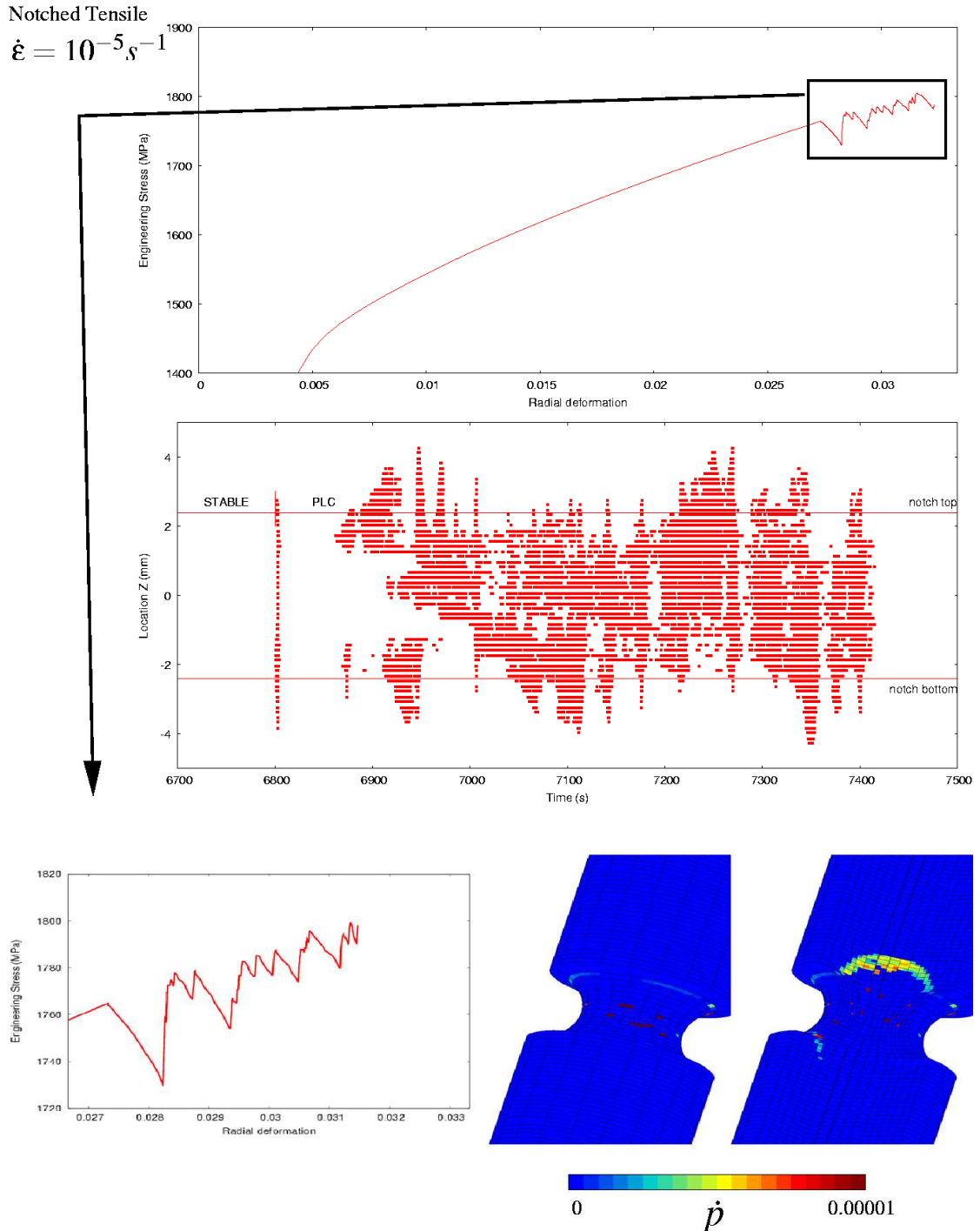
Figure VII.15 : Global stress/strain curve, location of bands as a function of time, zoom on serrations and plastic strain rate in the specimen at the end of the simulation for a notched axisymmetric specimen at a prescribed strain rate \dot{\epsilon} = 10^{-5} s^{-1} . (Animated picture)
