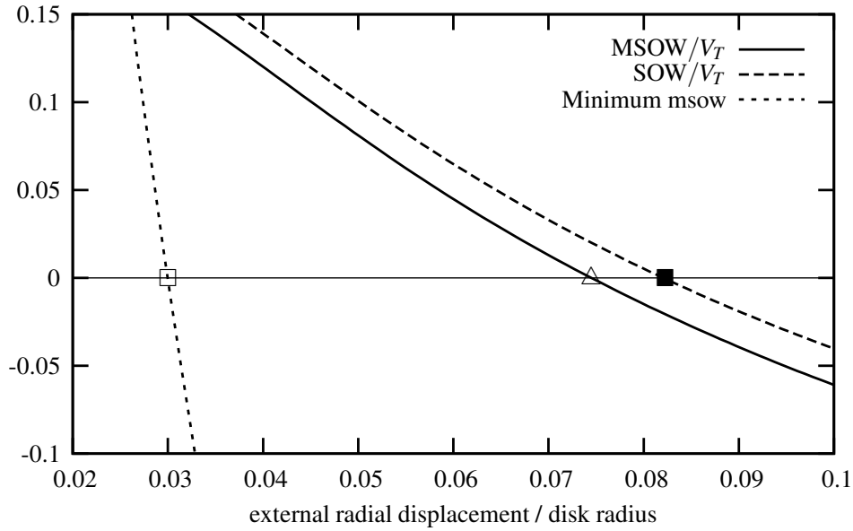
Figure II.6 : Influence of spin-softening on the stability criterion: MSOW, SOW, and minimum msow in the disk are plotted as a function of radial displacements. MSOW and SOW are divided by the total volume V_T .
