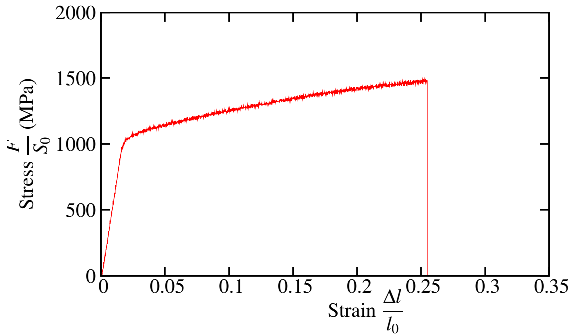
Figure III.17 : Tensile curve of axisymmetric smooth specimens in Udimet 720 at 500°C for a prescribed strain rate of 10^{-5} \text{ s}^{-1} .
