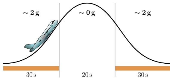
FIGURE II.1 – Parabola sequence
