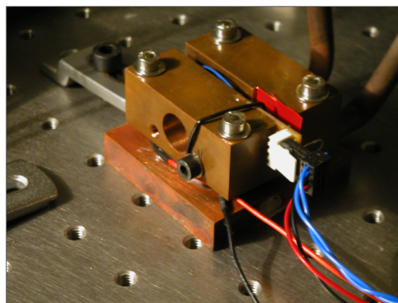
FIGURE IV.6 – Mechanical and thermal housing for the tapered amplifier (First-generation design)
