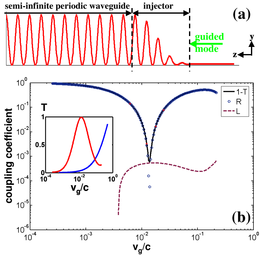
Figure 92 - Broadband injection from a planar waveguide to a periodic waveguide near the valence-band edge ( \lambda=1.65 \mu\text{m} ). (a) Injector geometry optimized for coupling at v_g/c \sim 0.01 . From left to right, the injector slit- and ridge-widths are 84, 143, 127, 158, 174 nm and 239, 213, 173, 166, 166 nm, respectively. The superimposed red curve represents the squared modulus of the transverse electric field at optimal coupling. (b) Performance of the injector predicted by fully vectorial computational results for the radiation loss L (dashed curve), the modal reflection R (blue circles) and the transmission T (actually 1-T is shown with a solid black curve). All quantities are displayed in a log scale. Inset: Injection efficiency T as a function of v_g with (red) and without (blue) injector. The maximum injection efficiency is as large as 0.999. In the absence of injector, this efficiency is only 0.25%.
