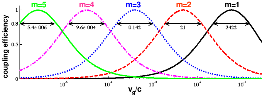
Figure 91 - Coupling efficiency into the slow-mode of a periodic stack ( n_H , n_L ) as a function of the group velocity (log scale) of the slow mode. Different injectors are considered. They are all composed of Bragg mirrors ( n_H , n_L ) with an increasing number of repeated pairs, m=1, \dots, 5 . The results are obtained in the vicinity of the valence band edge of the periodic stack. The horizontal arrows indicate the bandwidths in GHz of the different injectors for T=0.8 (-1dB).
