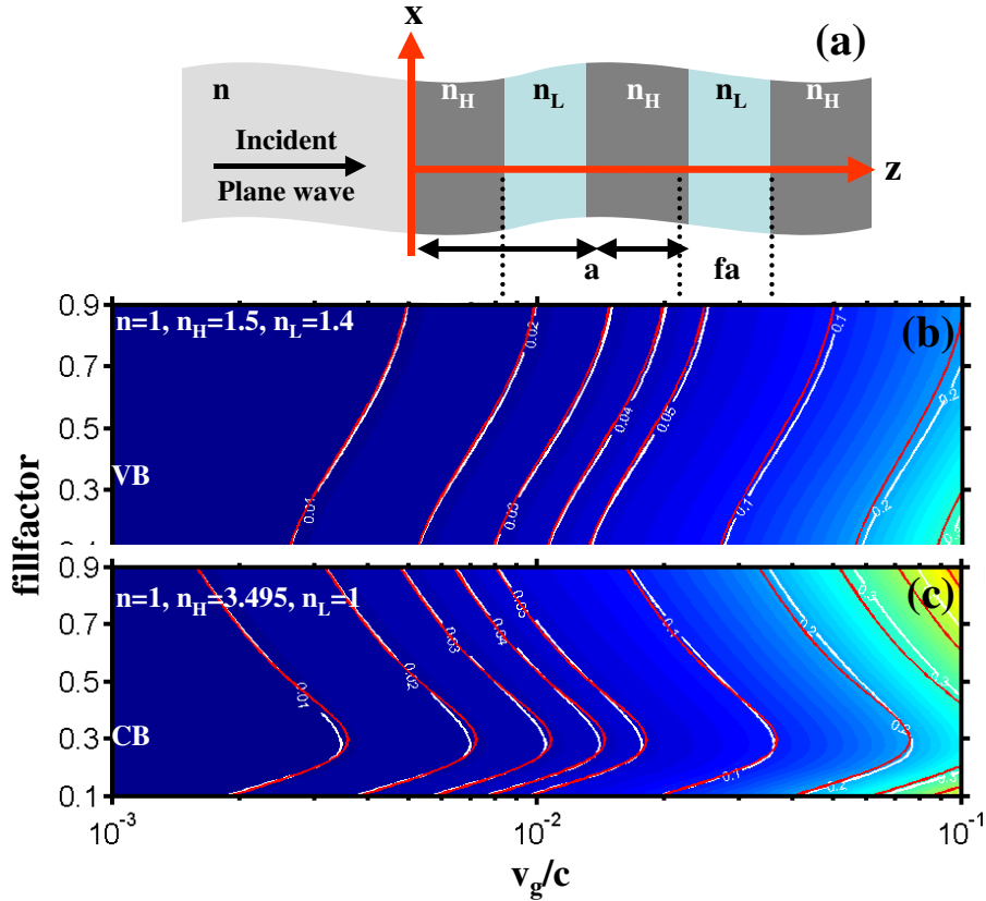
Figure 89 - Impedance mismatch problem. (a): Scattering at an interface between a uniform medium (refractive index n ) and a semi-infinite bi-layer periodic stack (refractive indices n_H and n_L ). (b) and (c): Injection efficiency T as a function of the group-velocity of the periodic-stack Bloch mode for different fill factors ( 0.1 < f < 0.9 ). Colormaps and white curves are exact numerical results obtained with the 2x2 transfer-matrix method in (YEH88), and the superimposed solid-red curves are obtained using the approximate closed-form expressions. (b): data obtained in the vicinity of the valence band edge of a
