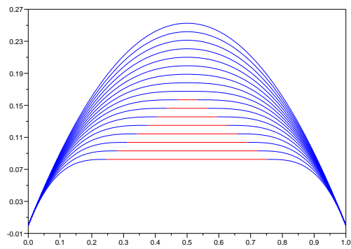
(b) q = 2
