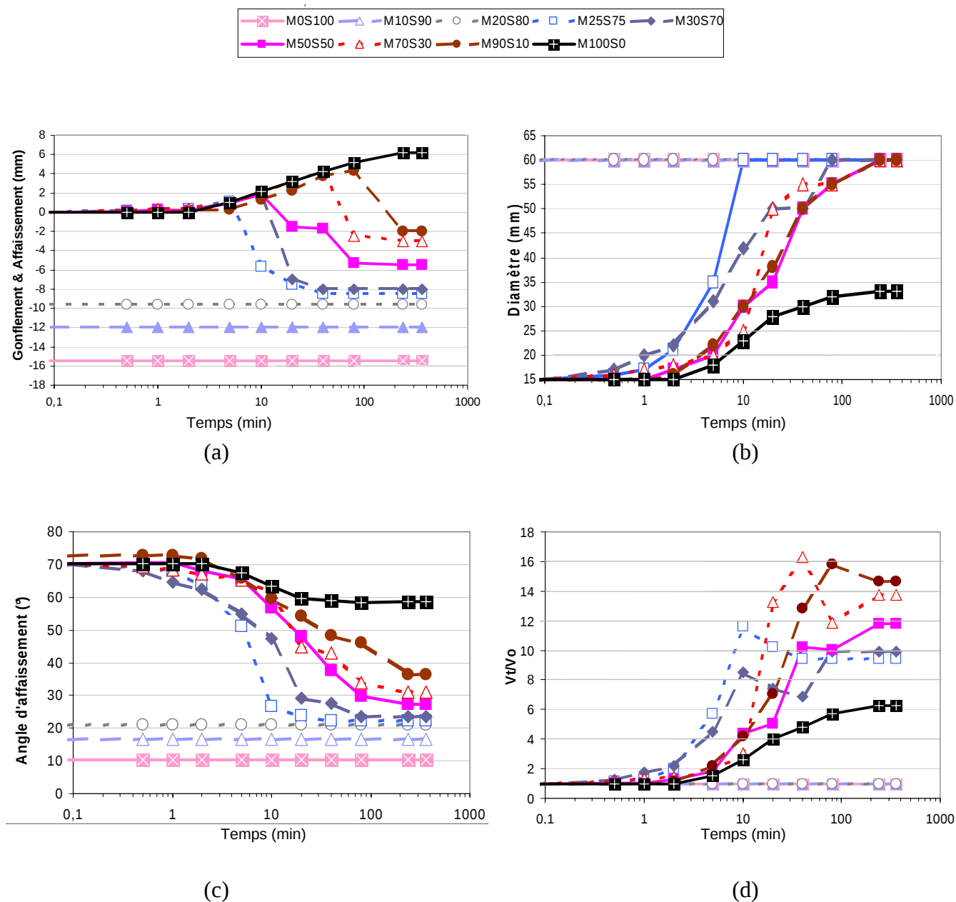
Figure 5-13. Mélange Montmorillonite (M)/sable (S)
