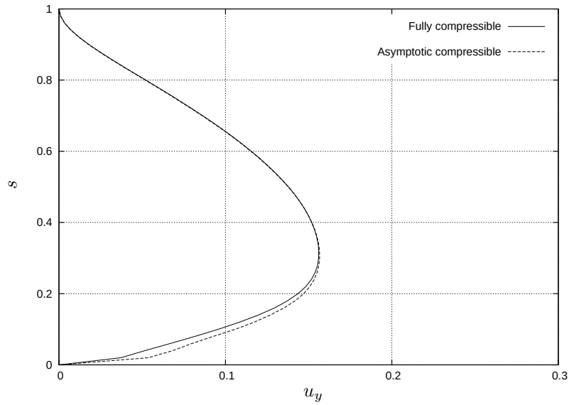
Figure 11.6.7: Tee Junction. Non-stationnary solution. Comparison between the density-based solver and the pressure-based solver. Curves of the velocity \tilde{u}_y in section P 23 P 33 at time level \tilde{t} = 15.7 s for a big value of the unsteady cut-off. All the quantities are expressed using SI units.
