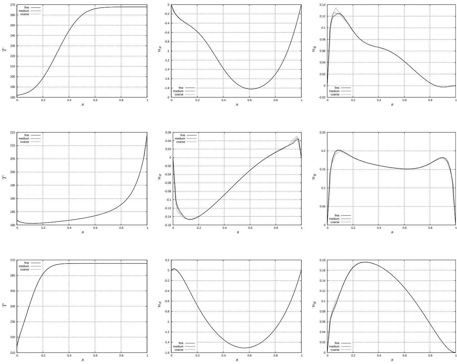
Figure 11.5.3: Tee junction. Asymptotic pressure-based compressible solver. Solution on the section P 23 P 33 (left), P 22 P 23 (middle) and P 22 P 32 (right). s is the curvilinear abscissa. All the quantities are expressed in the SI system.
