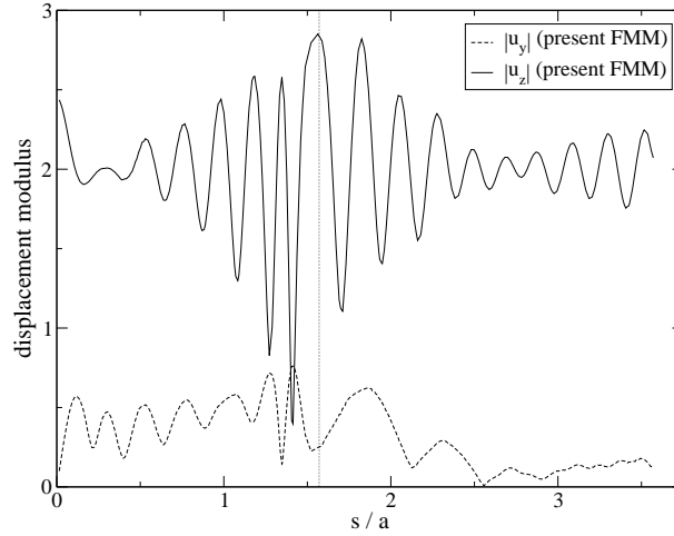
Figure 2.23: Diffraction of an incident plane P -wave by a semi-spherical canyon: horizontal and vertical computed displacement on line CDE (with points C , D , E defined on Fig. 2.21) plotted against normalized arc-length coordinate s/a along CDE (normalized frequency k_P a/\pi = 5 ).
