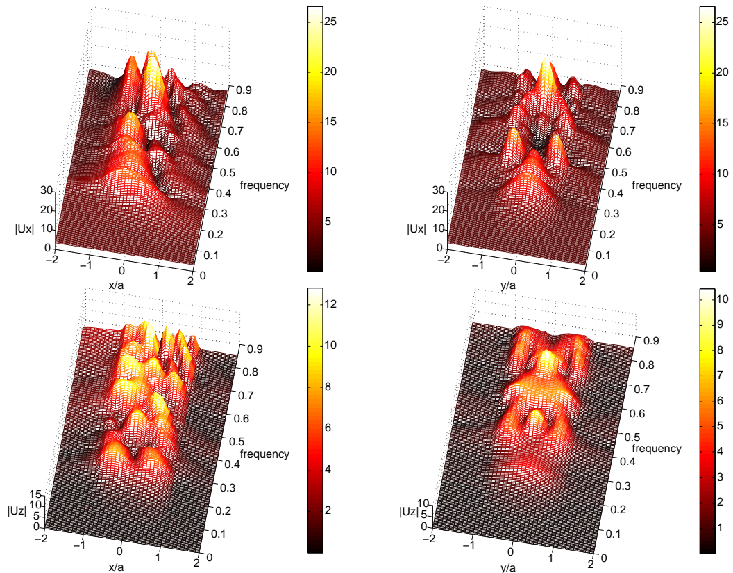
Figure 3.22: Propagation of an oblique ( \theta = 30^\circ ) incident plane SV-wave in a semi-spherical alluvial basin: x- (top) and z-component (bottom) of the FMM computed displacement against the x (left) and y (right) coordinate for the sample frequencies.
