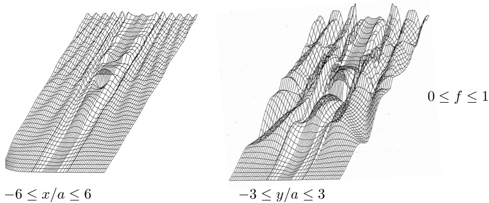
Figure 2.30: Diffraction of a vertically incident plane P -wave by a semi-ellipsoidal canyon: z -component of the BEM computed displacement against the Ox (left) and Oy (right) axes for 0 \text{ Hz} \leq f \leq 1 \text{ Hz} (results from [49]).
