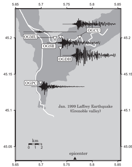
Figure 1.2: Seismic wave amplification in deep alluvial deposits (Grenoble, France): velocities (N-S component) recorded at various locations during the 1999 Laffrey earthquake (data: French accelerometric network, www-rap.obs.ujf-grenoble.fr ), from Semblat and Pecker [193].
