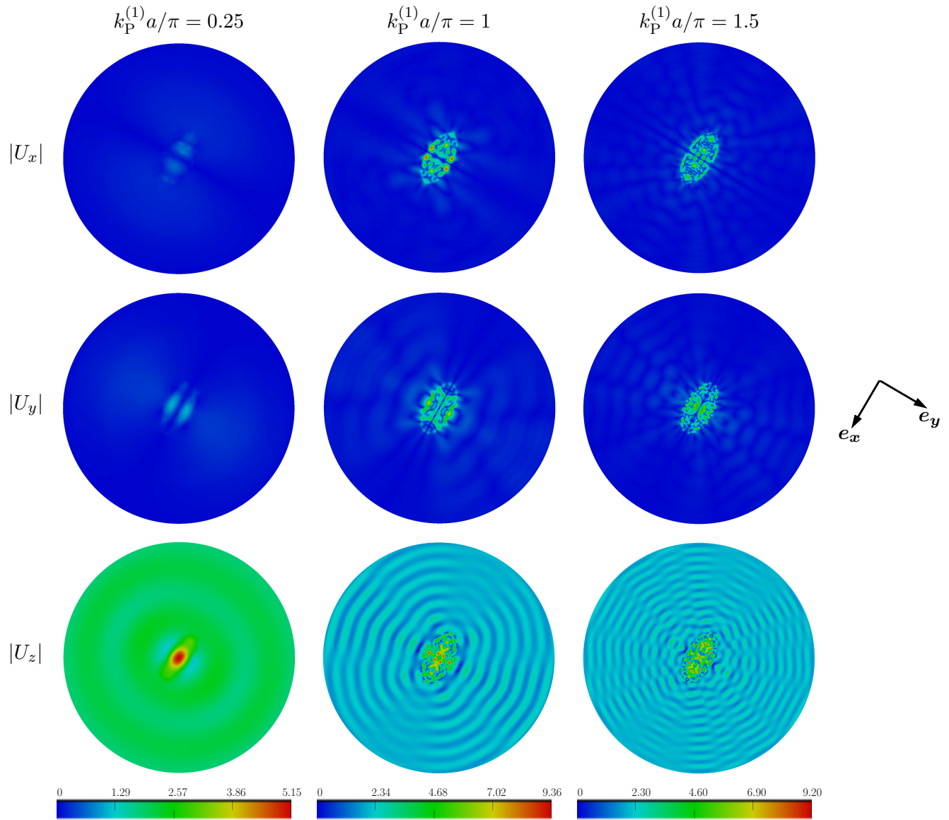
Figure 5.17: Diffraction of a vertical incident plane P-wave by a semi-ellipsoidal basin: x- (top), y- (middle) and z- (bottom) components of surface displacement for the normalized frequencies k_P a / \pi = 0.25 (left), k_P a / \pi = 1 (middle) and k_P a / \pi = 1.5 (right).
