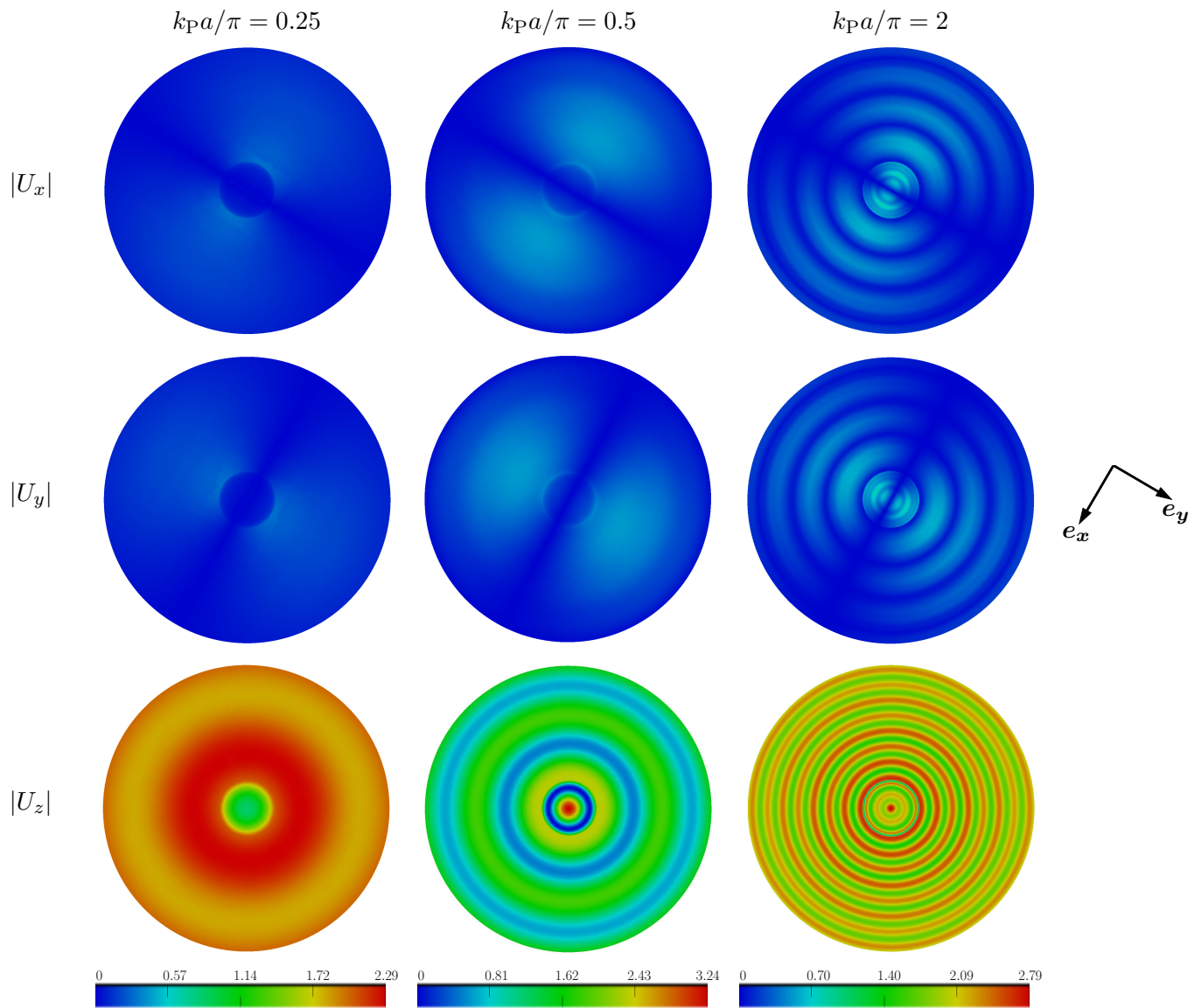
Figure 5.4: Diffraction of a vertical incident plane P-wave by a semi-spherical canyon: modulus of the x- (top), y- (middle) and z- (bottom) components of displacement for the normalized frequencies k_{Pa}/\pi = 0.25 (left), k_{Pa}/\pi = 0.5 (middle) and k_{Pa}/\pi = 2 (right).
