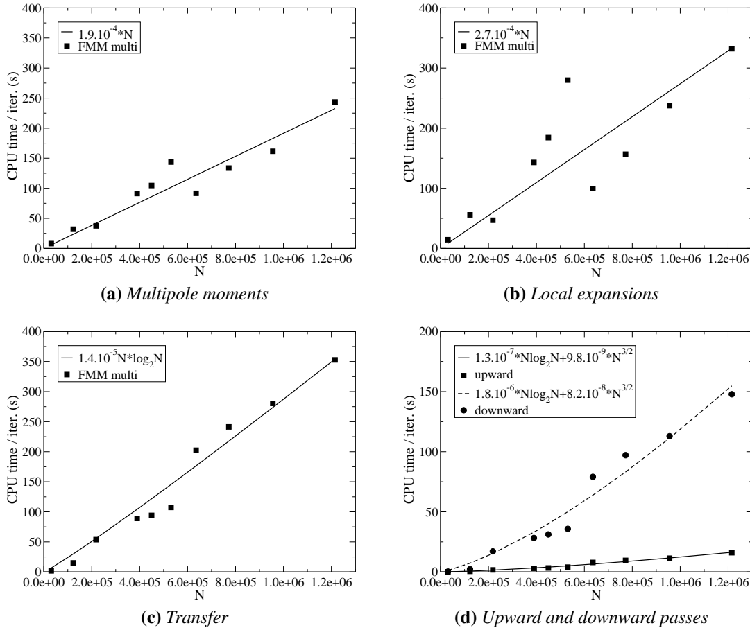
Figure 2.16: Theoretical complexity and recorded CPU times for the main steps of the multi-level elastodynamic FMM.
