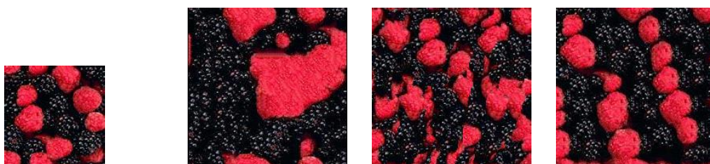
FIG. 5.9: (a) Sample 128 \times 128 pixels, (b) Efron and Leung's result, (c) Our method with o = 3 ( 250 \times 250 pixels in each case).
