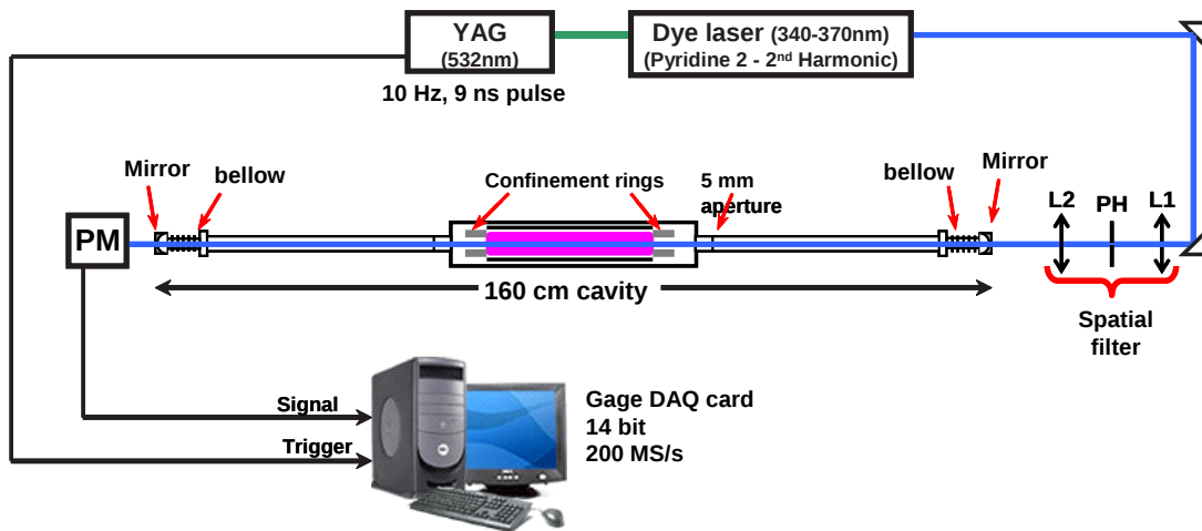
Figure 2.36: Schematic of the UV-CRDS experimental setup
