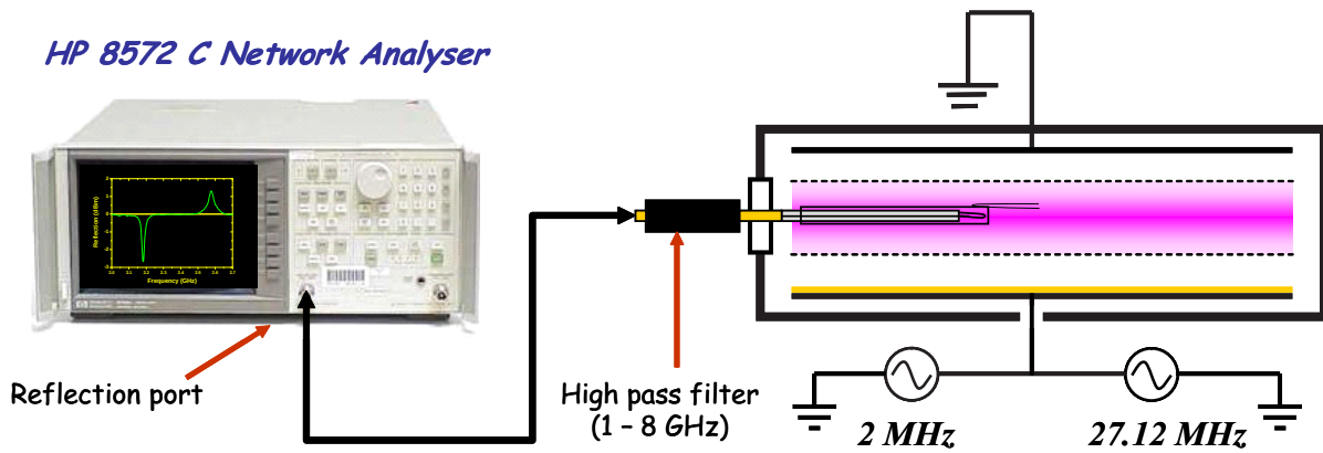
Figure 2.27: Experimental setup of the hairpin probe on the LPTP Exelan dual frequency reactor.
