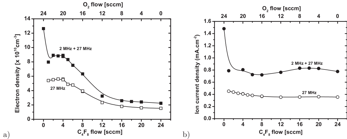
Figure 3.7: Ar/O 2 / c\text{-C}_4\text{F}_8 dual-frequency plasma with varying c\text{-C}_4\text{F}_8 and O 2 flow rates. a) Electron density b) Ion current
