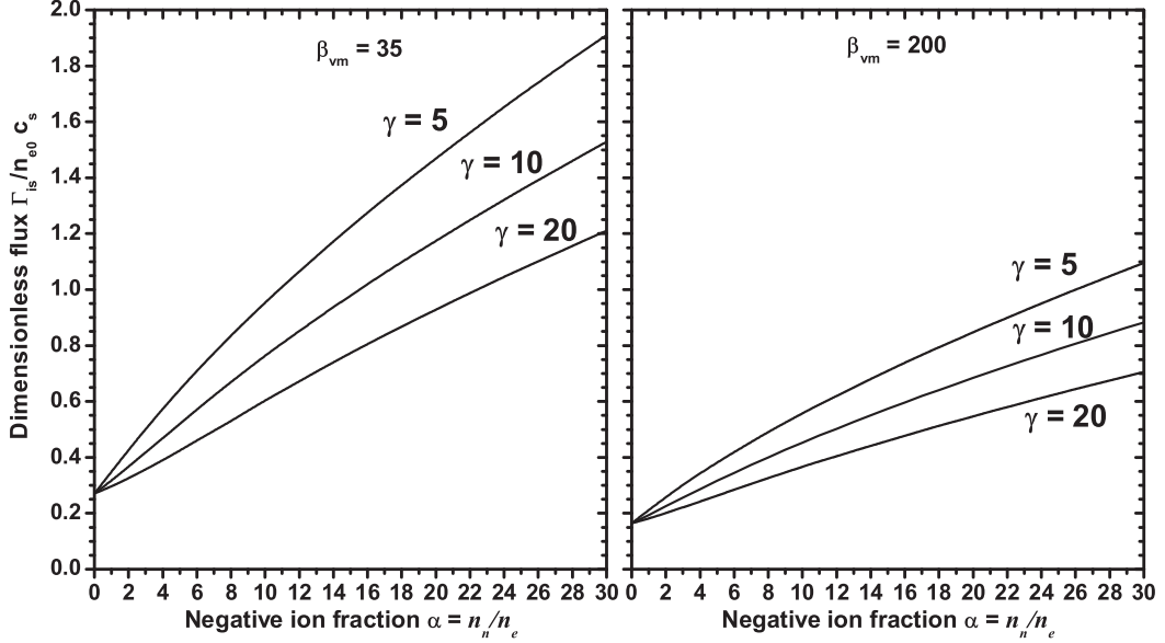
Figure 3.17: The normalised ion flux as a function of \alpha for \beta_{vm} = 35 and 200 , corresponding to electropositive h_I -factors of 0.275 and 0.17 respectively.
