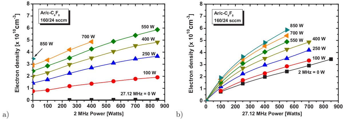
Figure 3.43: Electron density measurements in a dual frequency (27.12 MHz + 2 MHz) Ar/c-C 4 F 8 plasma as a function of (a) 2 MHz power for various set 27.12 MHz powers and (b) 27.12 MHz power for various set 2 MHz powers.
