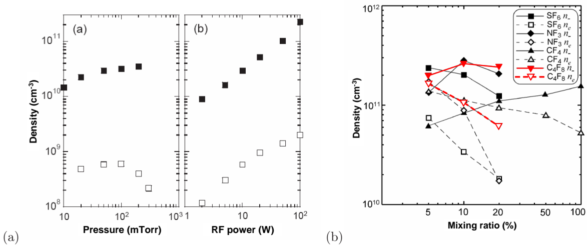
Figure 1.21: Negative ion and electron densities (a) in c -C 4 F 8 CCP plasma as a function gas pressure and power [Kono 00b] (b) in various ICP gas mixtures with argon at a total pressure of 25 mTorr and 300 W power [Kono 02].
