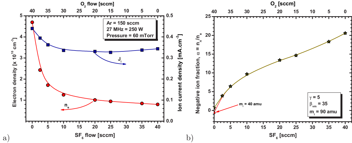
Figure 3.29: (a) Electron density and ion current and (b) negative ion fraction in a single frequency Ar/ \text{O}_2 / \text{SF}_6 plasma with varying of \text{O}_2 / \text{SF}_6 flows.
