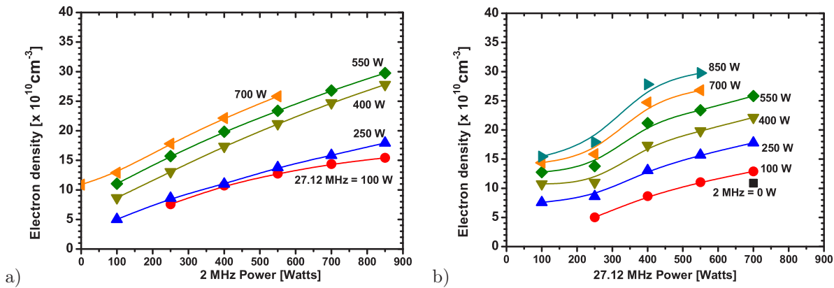
Figure 3.45: Electron density measurements in a dual frequency (27.12 MHz + 2 MHz) Ar/O 2 plasma as a function of (a) 2 MHz power for various set 27.12 MHz powers and (b) 27.12 MHz power for various set 2 MHz powers.
