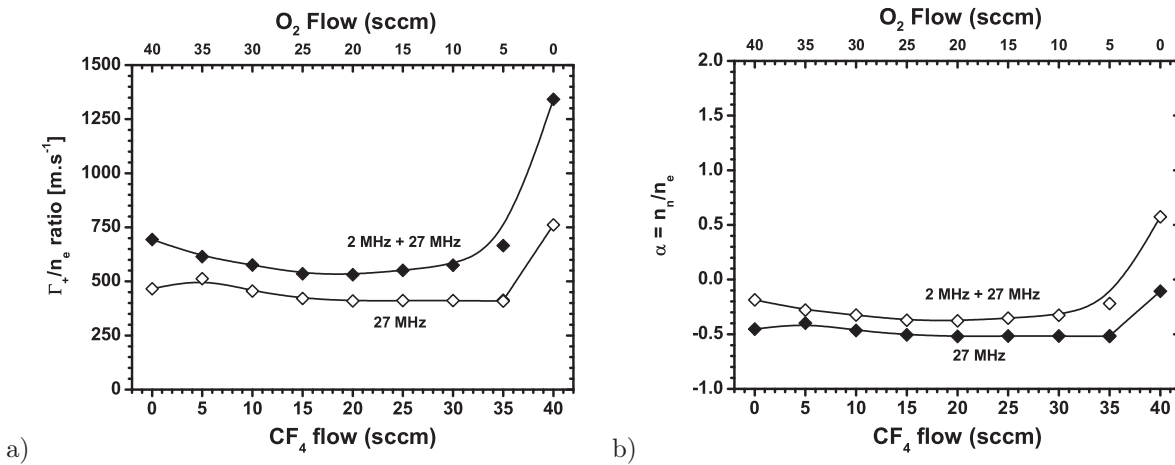
Figure 3.10: Ar/O 2 /CF 4 dual-frequency plasma with varying CF 4 and O 2 flow rates. a) \Gamma_i/n_e ratios; b) negative ion fractions calculated using the simple model. T_e is taken as 5 eV and m_i is assumed to be \sim 50 amu.
