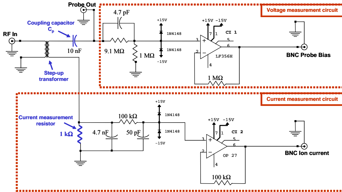
Figure 2.11: LPTP ion flux probe measurement circuit
