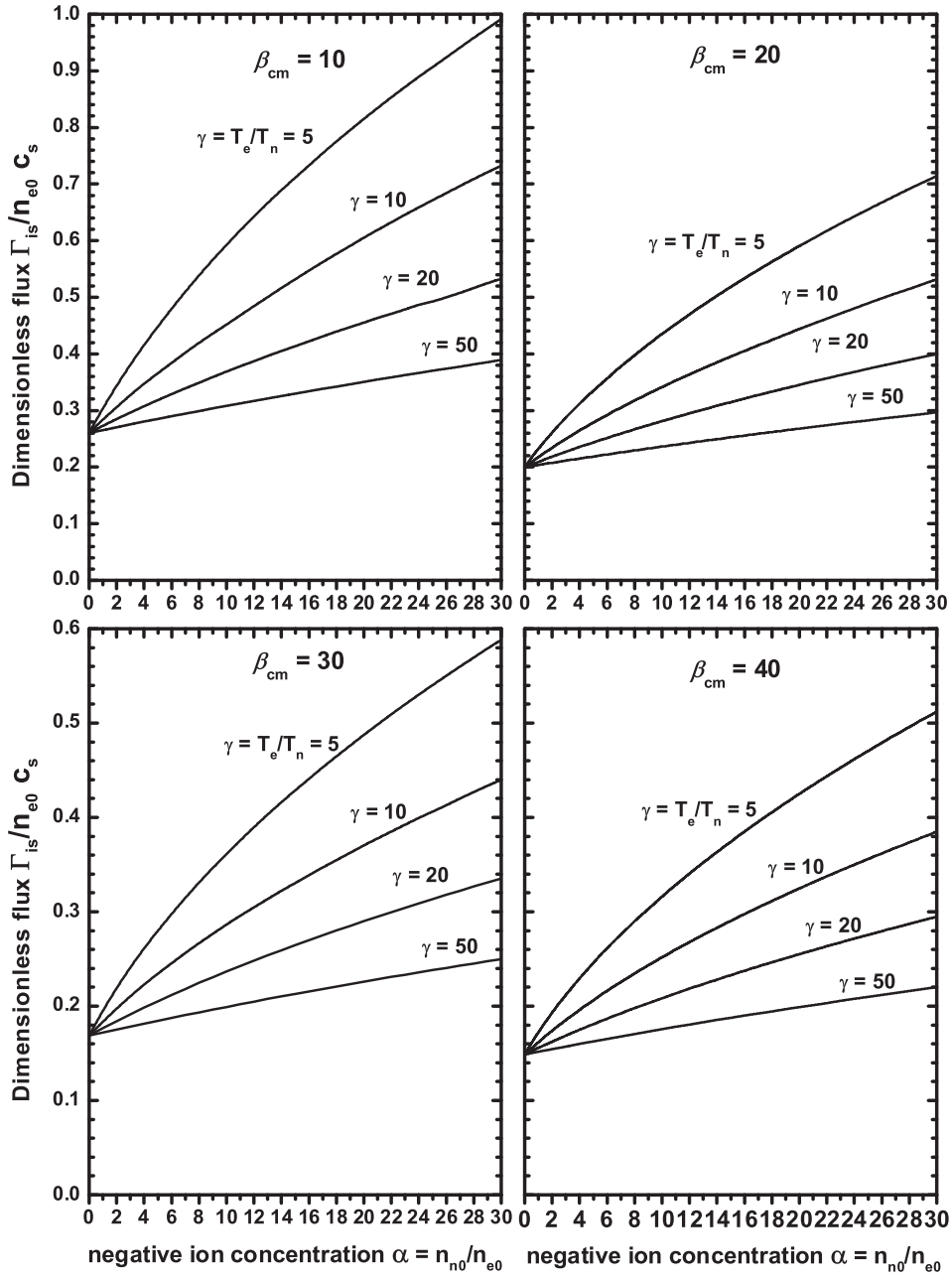
Figure 1.20: The normalised ion flux as a function of alpha for \beta_{cm} = 10, 20, 30 and 40 .
