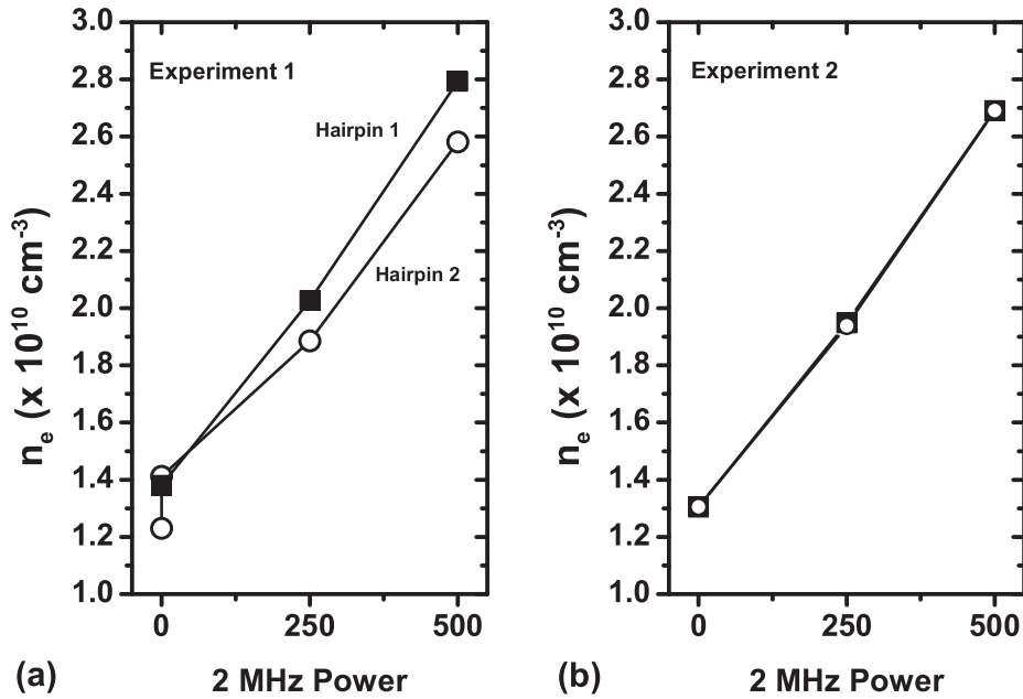
Figure 2.30: Electron density measurements as a function of 2 MHz power with two different hairpins in an Ar/O 2 /c-C 4 F 8 plasma, 52 mTorr at a constant 27 MHz power of 250 W. (a) both probes were not identically aligned axially; (b) both probes in same axial position.
