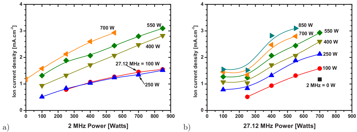
Figure 3.44: Ion current measurements in a dual frequency (27.12 MHz + 2 MHz) Ar/O 2 plasma as a function of (a) 2 MHz power for various set 27.12 MHz powers and (b) 27.12 MHz power for various set 2 MHz powers.
