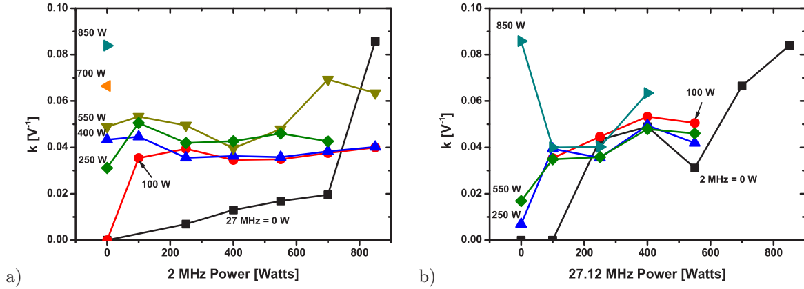
Figure 3.39: k -factor measurements in a dual frequency (27.12 MHz + 2 MHz) Ar/O 2 /c-C 4 F 8 plasma as a function of (a) 2 MHz power for various set 27.12 MHz powers and (b) 27.12 MHz power for various set 2 MHz powers.
