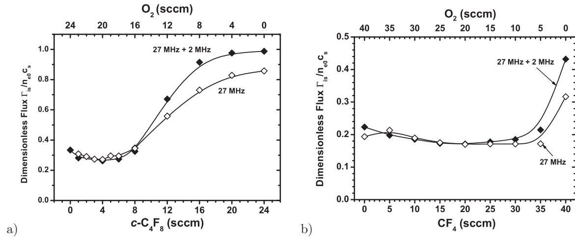
Figure 3.13: The normalised ratio in a) Ar/O 2 /c-C 4 F 8 and b) Ar/CF 4 /O 2 plasma mixtures for both single and dual frequency RF power modes. The c_s used for normalising used a T_e of 3 eV in the single frequency data and 5 eV in the dual frequency data. Positive ion masses of 100 amu and 50 amu for the c-C 4 F 8 and CF 4 containing plasmas respectively.
