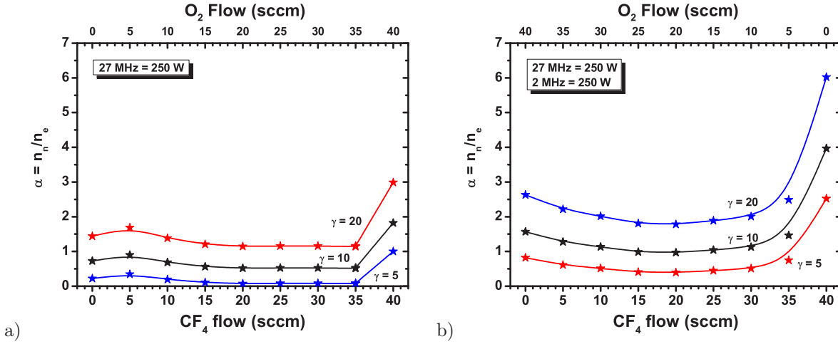
Figure 3.12: Ar/O 2 /CF 4 plasma mixtures with varying CF 4 and O 2 flow rates. Negative ion fractions calculated using the simple model, but using the modified Bohm velocity for various values of \gamma (5,10 and 20) in a) single frequency and b) dual frequency. T_e is taken as 5 eV and m_i is assumed to be \sim 50 amu.
