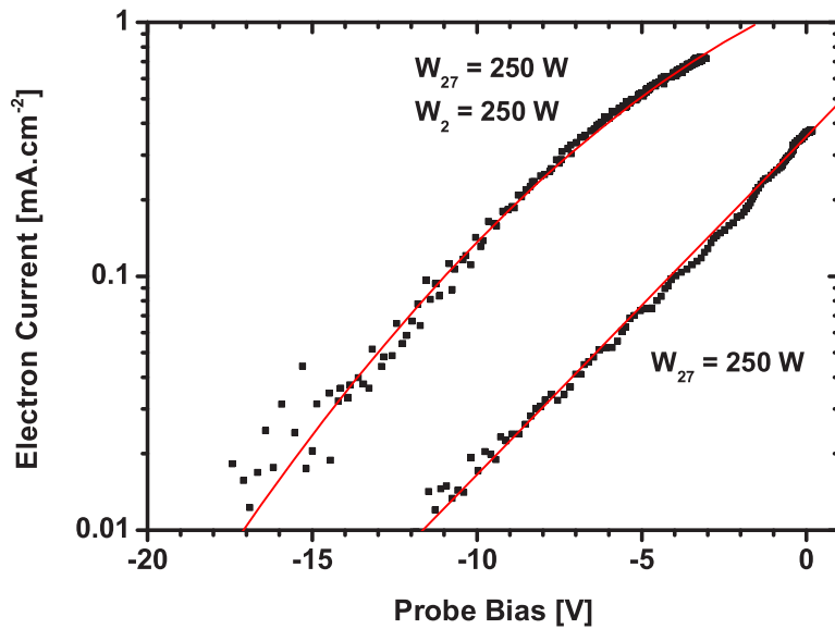
Figure 2.14: The electron current as a function of probe bias voltage, obtained by subtracting the ion current (with slope) from the data shown in figure 2.13. The experimental data (black dots) is fitted with a straight (red) line in the single frequency case, and a 2^{nd} order polynomial (red) line in the dual frequency case.
