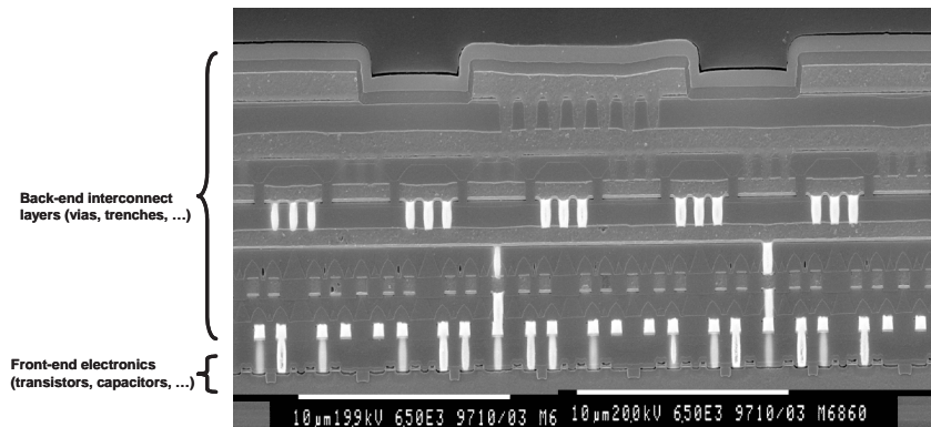
Figure 1.2: Superposition of layers of doped silicon, conductor (Al, W) and dielectric ( \text{SiO}_2 ) all etched and deposited by plasma processing. This photo is of 0.25 \mu\text{m} CMOS architecture. Source: STM.
