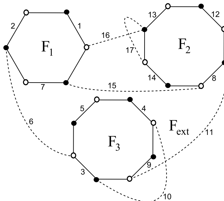
FIG. 6.9 – Example of a well-labeled cumulant map of resultant (1 \dots 17)
