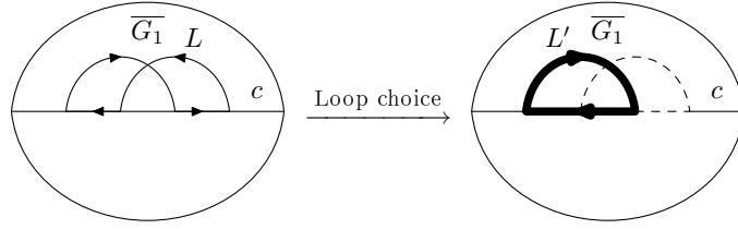
FIG. 8.12 – Good choice of cycle
