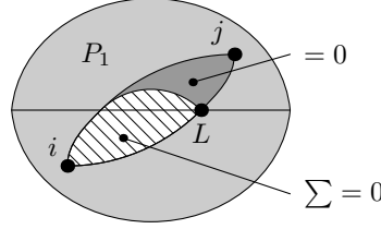
FIG. 8.17 – Case 1 : i \notin V_c and j is not in the same region than j .
