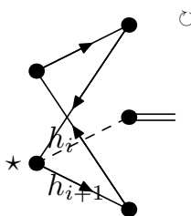
FIG. 8.9 – Example of a map M' with an admissible cycle of type 2.
