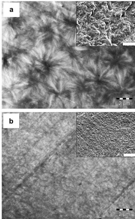
Fig. 6. TEM images of PA-6/MWNT composites with (a) 0 wt%, (b) 0.1 wt% and inset shows the SEM images of the same composites – scale bar 2 μm for TEM and 5 μm for SEM.
