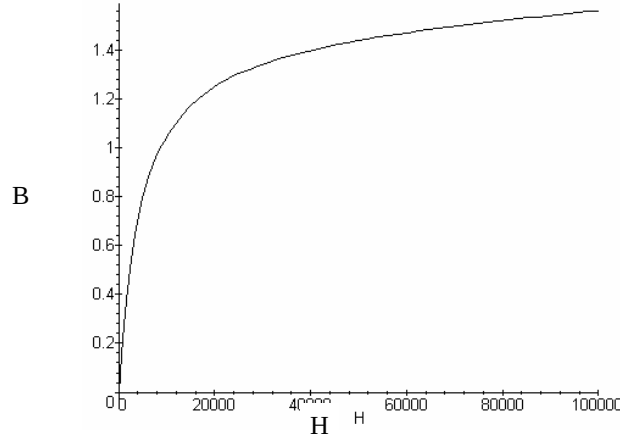
Figure 10: Typical magnetization curve B(H) obtained with the Frohlich-Kenelly model. B is expressed in Tesla and H in A/m. Coefficients a and b are respectively 1.5 and 4500.
