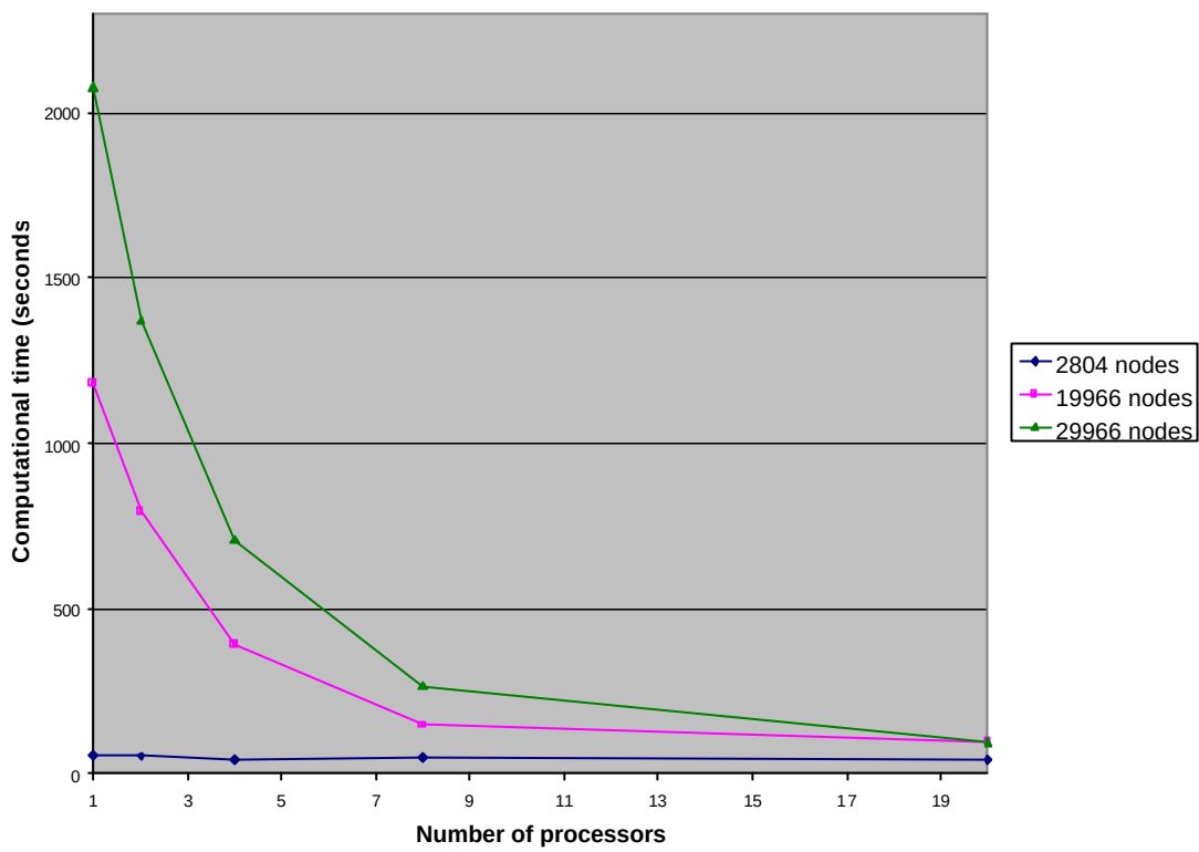
Figure 66 : Computational time versus the number of processors for three different mesh sizes
