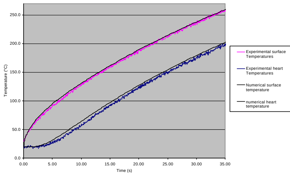
Figure 17: Long inductor case: comparison between experimental and computed temperature evolutions
