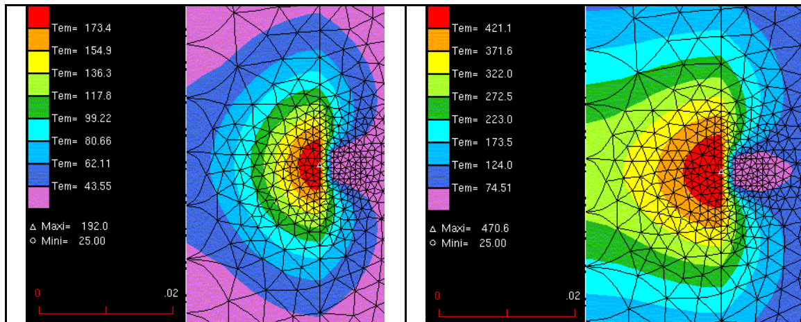
Figure 25: Temperature at two time steps at a frequency of 60 Hz for a non magnetic part ( m_{relative} = 1 ); a) t=5s b) t=25s
