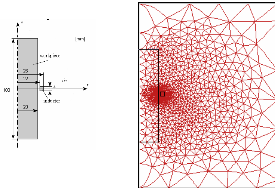
Figure 20: Static short inductor case: geometry and mesh
