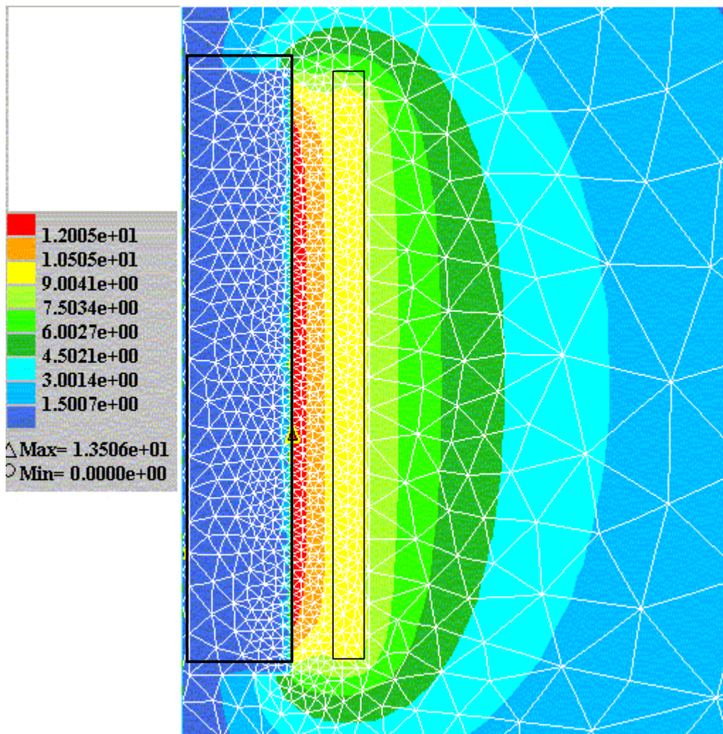
Figure 15: Long inductor case: effective electric field isovalues
