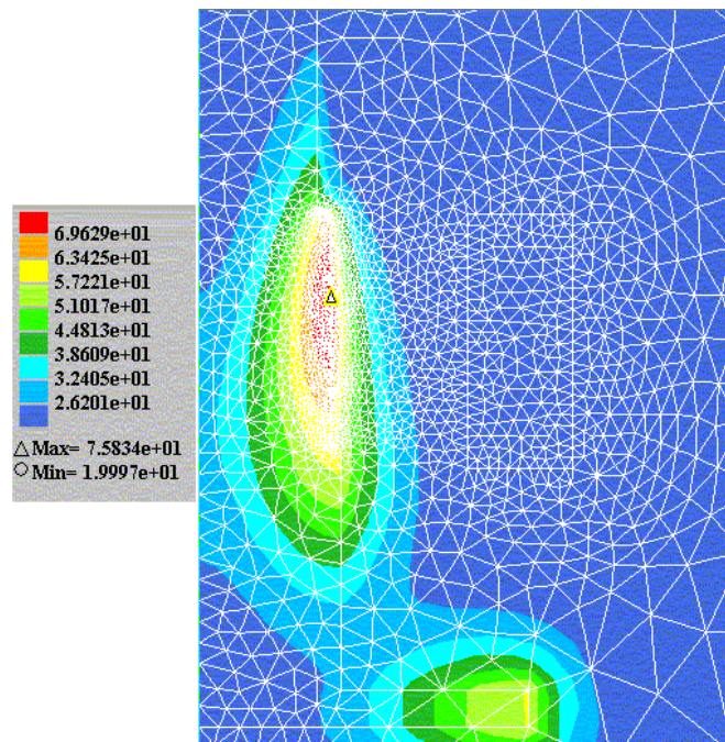
Figure 29: Moving inductor case: temperature isovalues at a given displacement step of the inductor
