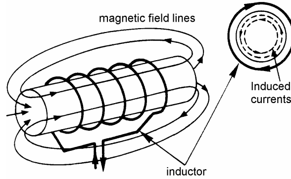
Figure 9: Induction heating setup
