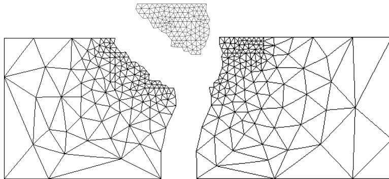
Figure 58: Splitting of an initial multi-material mesh of 714 elements in three sub-meshes of 240, 236 and 238 elements.
