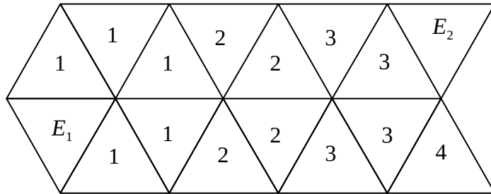
Figure 57: Exemple of distance value between two elements. Here d(E_1, E_2) = 4 .
