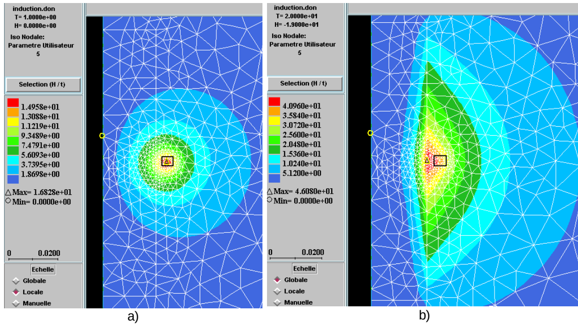
Figure 22: Static short inductor case: effective electric field isovalues for two different permeabilities of the part at a frequency of 60 Hz. a) m_{relative} = 1 b) m_{relative} = 90
