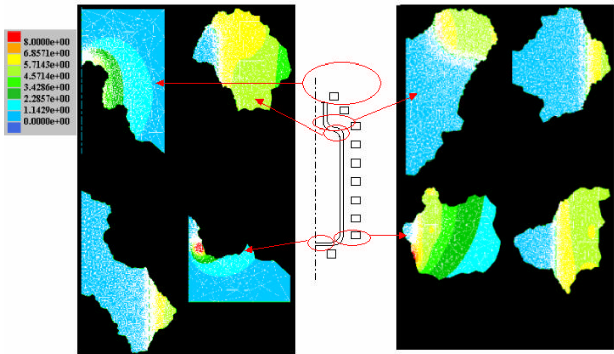
Figure 75 : ISO curves of the effective electrical field on a partition into 8 sub-meshes from the initial mesh of size 70000 nodes.
