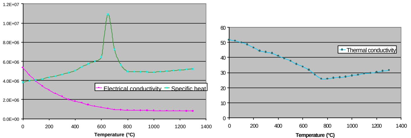
Figure 14: Electrical conductivity, specific heat and thermal conductivity versus Temperature
