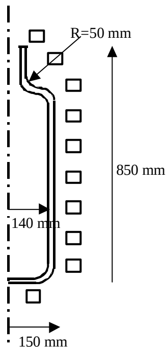
Figure 73 : Geometry of the gas bottle and of the ten inductors
