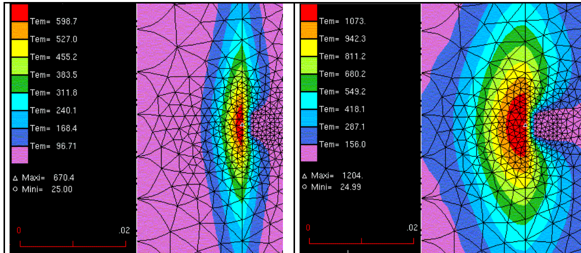
Figure 26: Temperature at two time steps for a magnetic part ( m_{relative} = 90 ); a) t=1s b) t=5s
