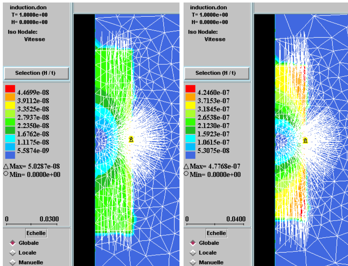
Figure 27: Nodal velocities in the workpiece due to dilatation effects for a frequency of 60Hz; a) non magnetic material ( m_{relative} = 1 ), b) non magnetic material ( m_{relative} = 90 )
