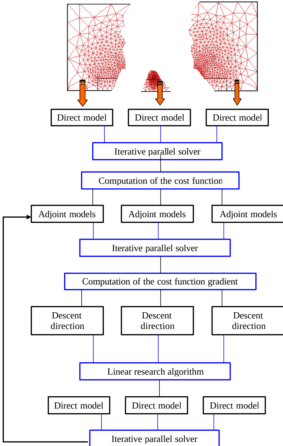
Figure 72 : General organization of the parallel optimization algorithm.
