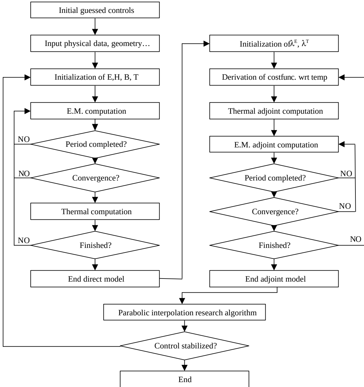
Figure 70: General algorithm for the optimization procedure coupled to the induction heating model.
