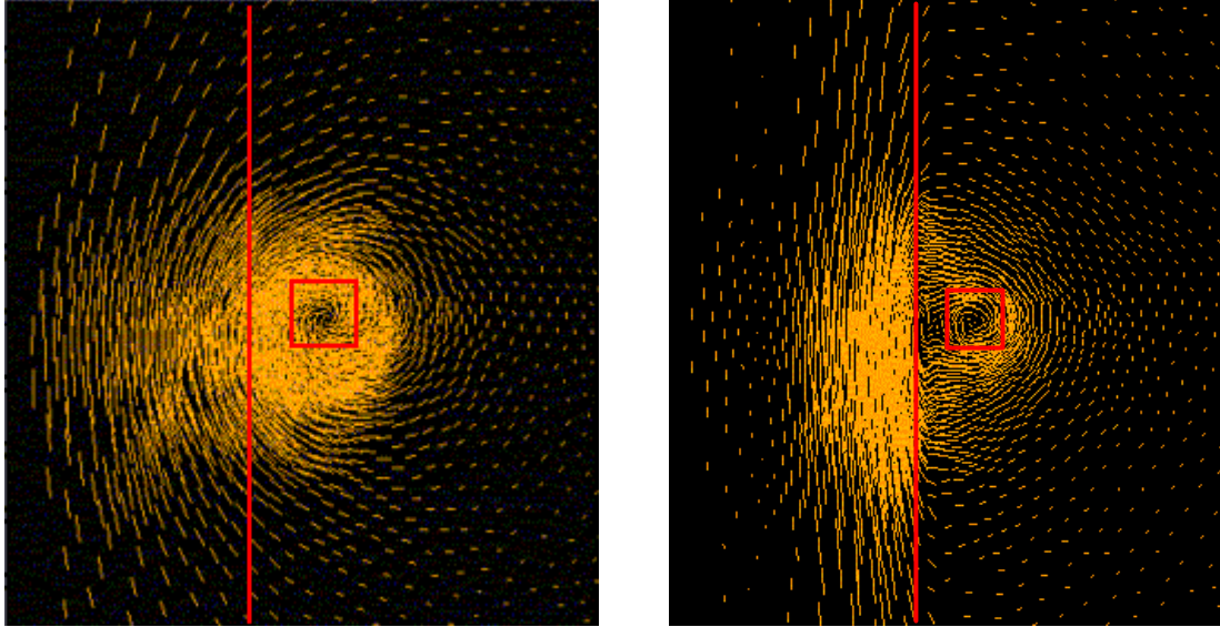
Figure 24: Static short inductor case at 60Hz: magnetic lines for m_r = 1 and m_r = 90
