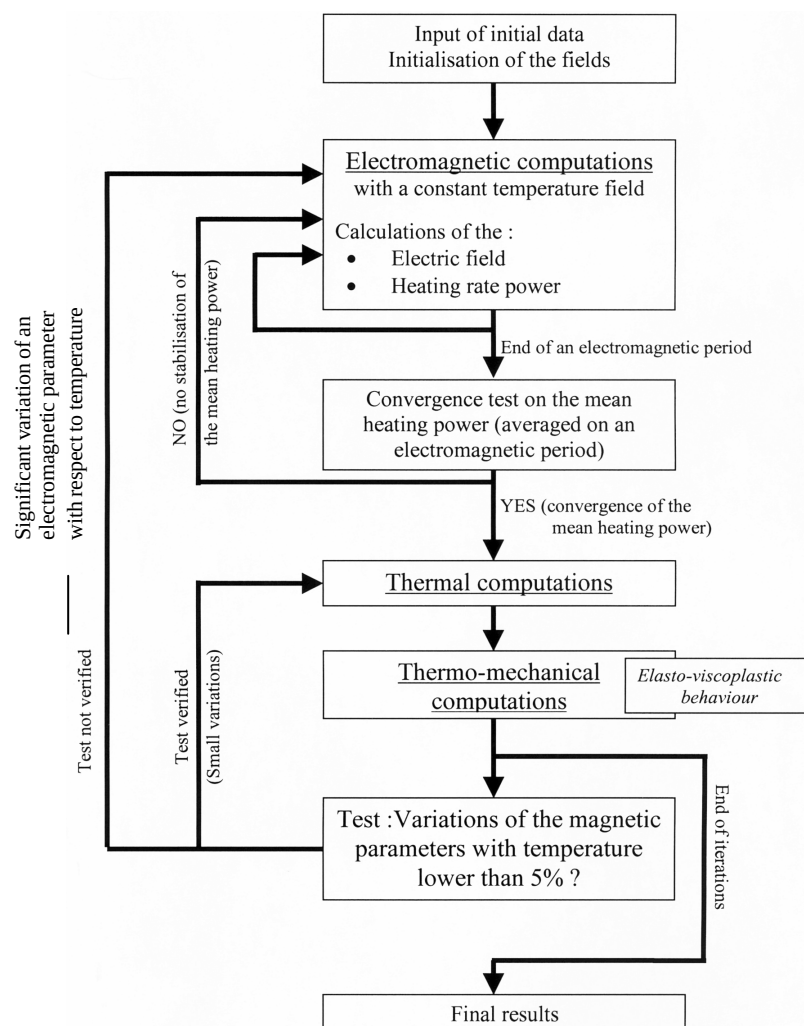
Figure 69: Algorithm of the direct model
