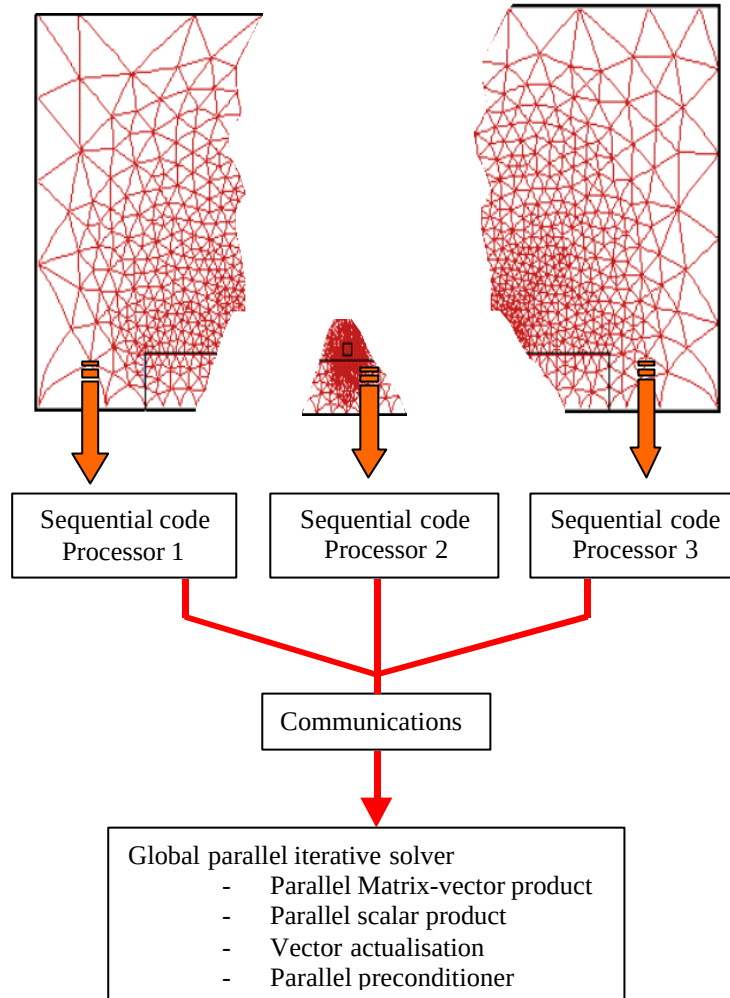
Figure 56 : Partitioning method strategy
