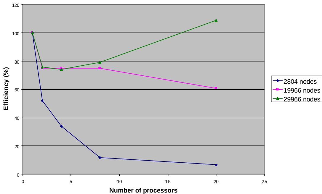
Figure 67 : Efficiency versus the number of processors for different mesh sizes
