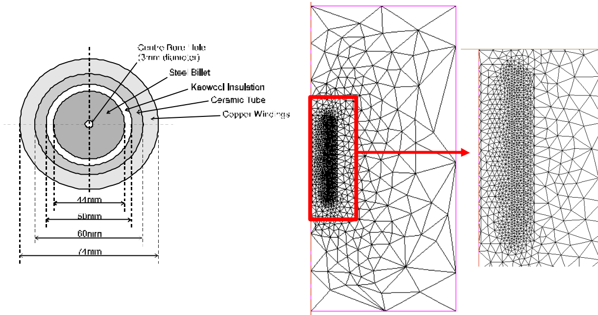
Figure 13: Static long inductor case: geometry and mesh (12000 nodes)
