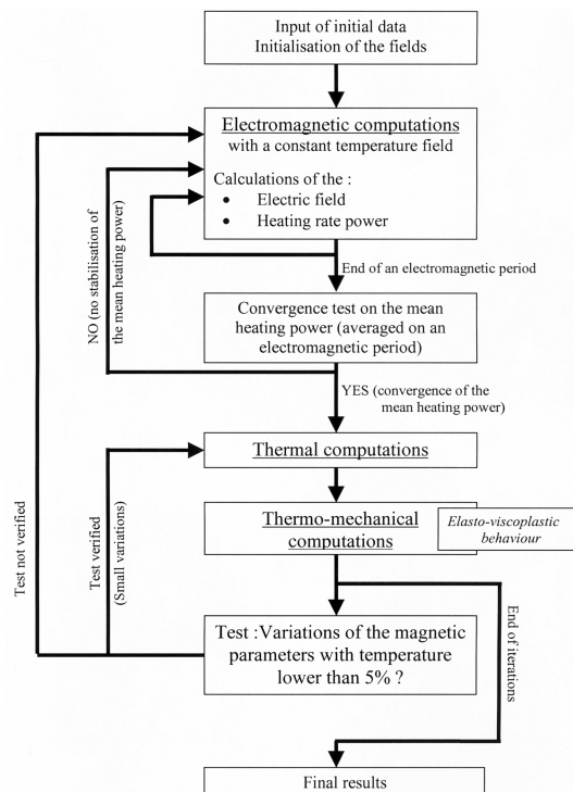
Figure 55: Flow chart of the induction heating code
