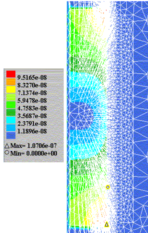
Figure 19: Long inductor case: nodal velocities in the mesh at a given time step
