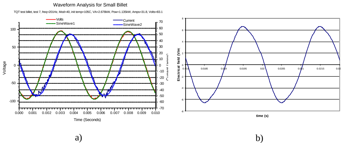
Figure 16 : a) Evolution with respect to time of the experimental intensity in the coil ; b) Evolution with respect to time of the numerically computed electrical field in the part.
