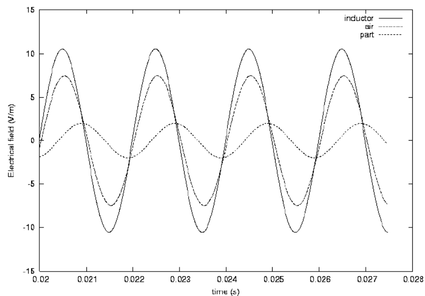
Figure 21 : Evolution of the electric field versus time for a non magnetic material at three given locations in the coil, the part and in the space in between. The electrical field is maximum in the coil.
