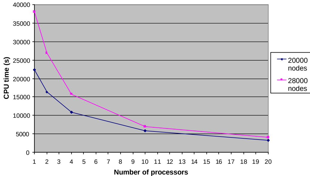
Figure 79 : Evolution of the CPU time with respect to the number of processors for a mesh of about 20000 and 28000 nodes
