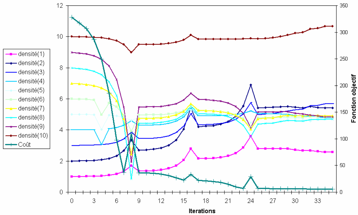
Figure 74 : Evolutions of the current densities and of the cost function versus the number of iterations
