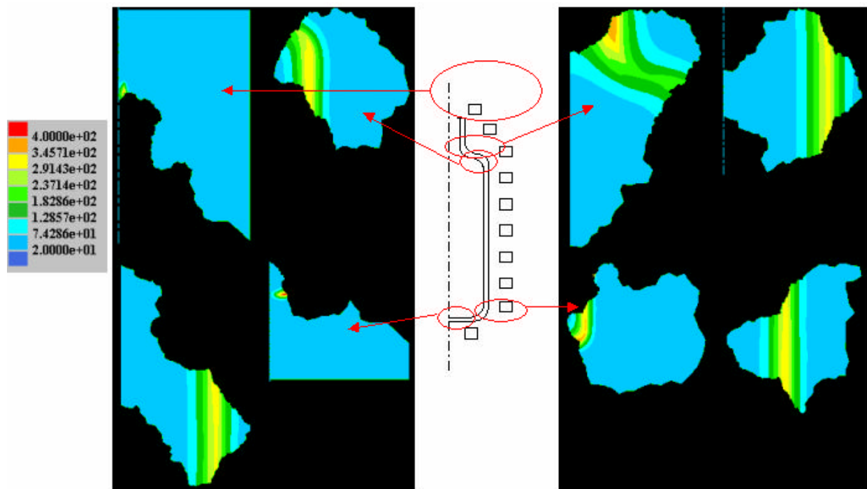
Figure 76 : ISO curves of temperature field on a partition into 8 sub-meshes from the initial mesh of size 70000 nodes. The colored regions are parts of the gas container.
