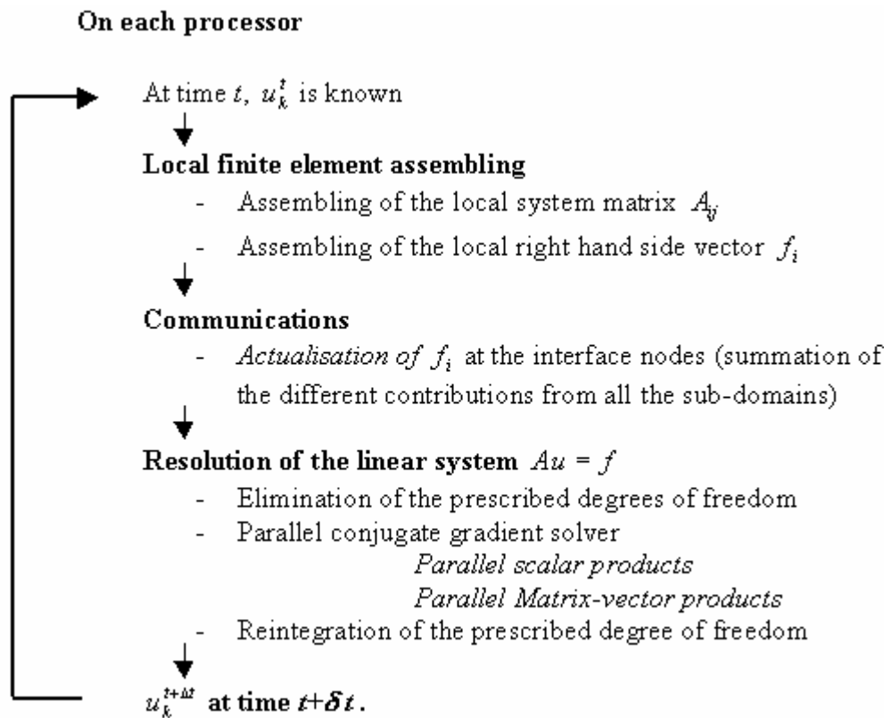
Figure 71: The domain partitioning algorithm
