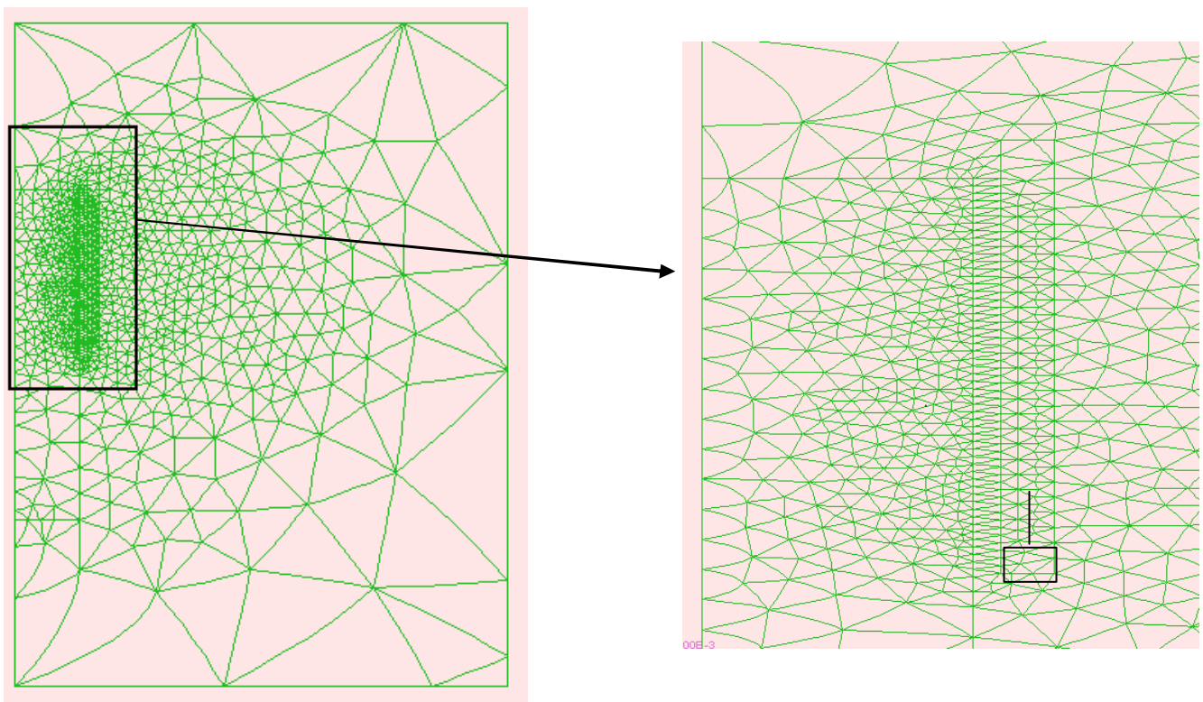
Figure 11: Example of mesh for a simulation with a coil displacement: the area of displacement is delimited and meshed
