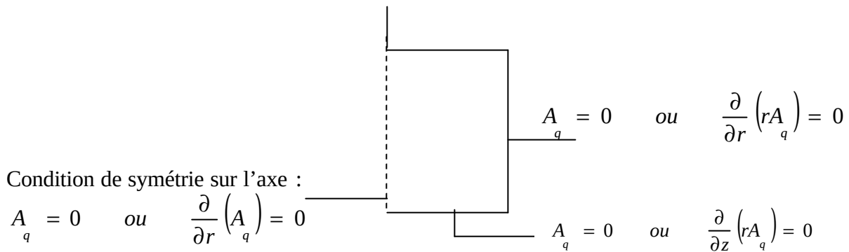
Figure 7 : Conditions aux limites standards
