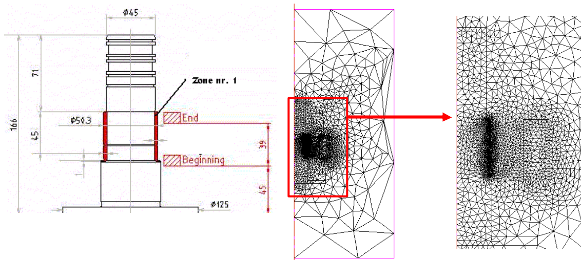
Figure 28: Moving inductor case: geometry and initial mesh
