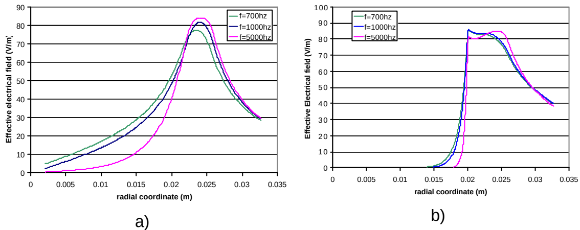
Figure 23: Effective electrical field profiles on the radial axis for 3 different frequencies f=700\text{Hz} , 1000\text{Hz} and 5000\text{Hz} . a) The part is a non magnetic material (relative magnetic permeability of the part equal 1), b). The part is a ferromagnetic material (relative magnetic permeability of the part equal 90).
