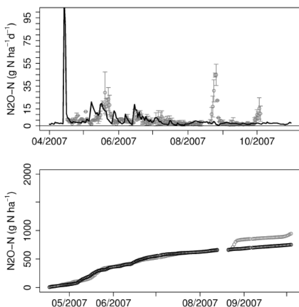
Figure A8-1: CERES-NOE (best set of parameter values) Simulated fluxes in black, observed in grey Uncompacted sugar beet plot in 2007 RMSE (N 2 O daily emissions): 7.3 g N-N 2 O ha -1 d -1 RMSE (cumulated N 2 O emissions): 79.08 g N-N 2 O ha -1
