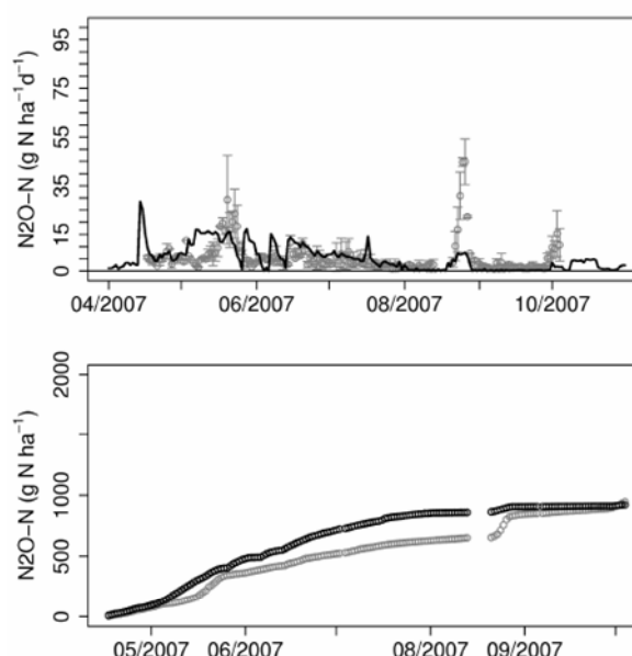
Figure A8-2: CERES-NOE2 (best set of parameter values) Simulated fluxes in black, observed in grey Uncompacted sugar beet plot in 2007 RMSE (N 2 O daily emissions): 6.97 g N-N 2 O ha -1 d -1 RMSE (cumulated N 2 O emissions): 138.89 g N-N 2 O ha -1
