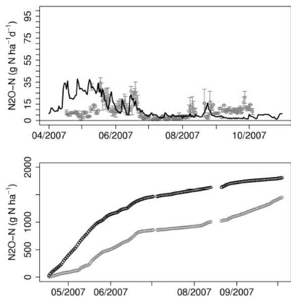
Figure A8-3: CERES-NOE (best set of parameter values) Simulated fluxes in black, observed in grey Compacted sugar beet plot in 2007 RMSEP (N 2 O daily emissions): 10.83 g N-N 2 O ha -1 d -1 RMSEP (cumulated emissions): 557.39 g N-N 2 O ha -1
