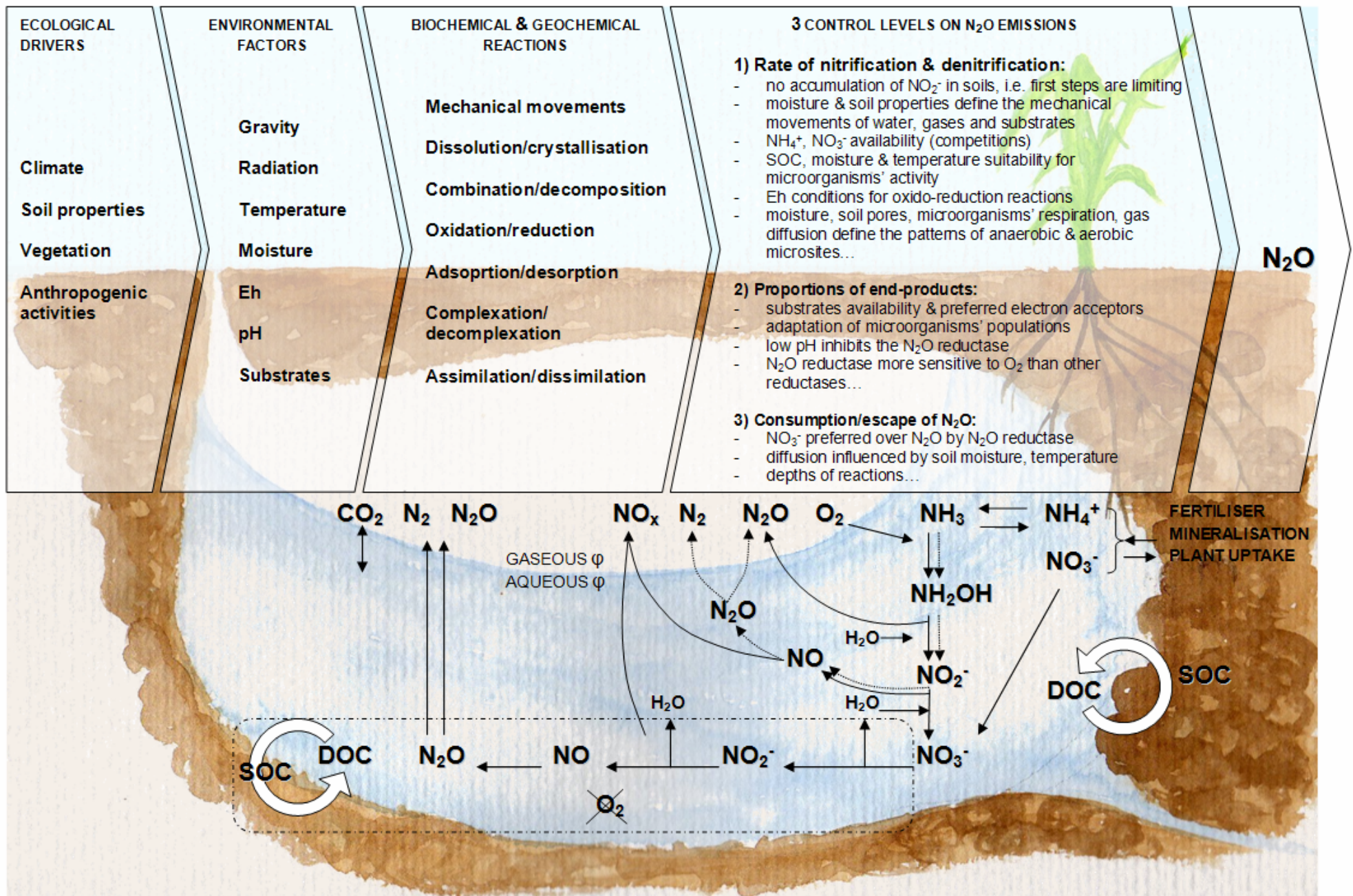
Figures 18: Scheme of the determinism of N 2 O emissions by soils adapted from Li (2007); Wrage et al. (2005); Farquharson and Baldock (2008). Soil particles, gaseous and aqueous phases ( \phi ) are artificially “well distinguished”. The two extremities of the symbolised pore represent the pore continuum throughout the soil matrix. Reactions take place at the interface of soil particles and aqueous phase where microorganisms and substrates are. Denitrification takes place in the “anaerobic dashed-line rectangle”. Dashed arrows lead to N 2 O emissions by nitrifier denitrification occurring in low O 2 conditions, which implies that some NH 3 oxidisers process the whole reaction chain (Wrage et al. , 2001).
