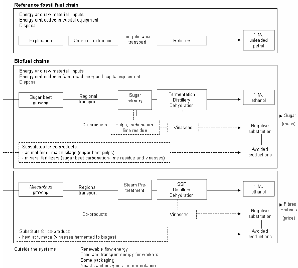
Figure 1: Well-to-Tank system boundaries of studied fuel chains.
