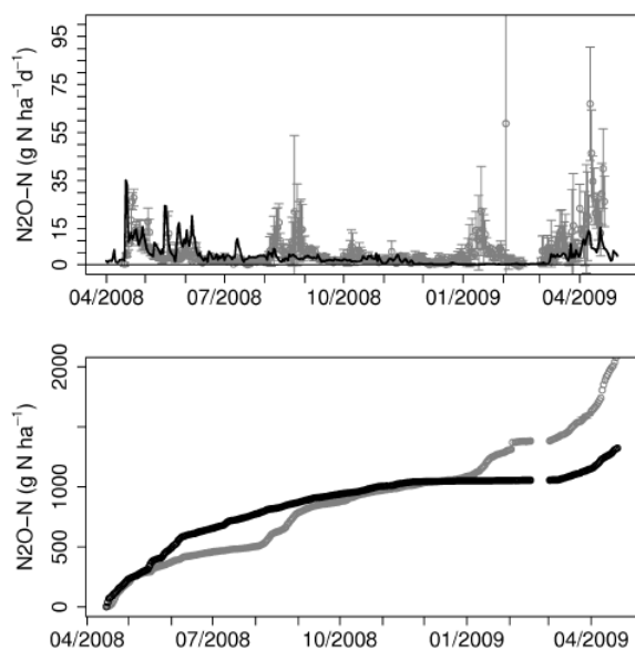
Figure A8-5: CERES-NOE (best set of parameter values) Simulated fluxes in black, observed in grey Uncompacted sugar beet plot in 2008 RMSEP (N 2 O daily emissions): 8.12 g N-N 2 O ha -1 d -1 RMSEP (cumulated emissions): 232.02 g N-N 2 O ha -1
