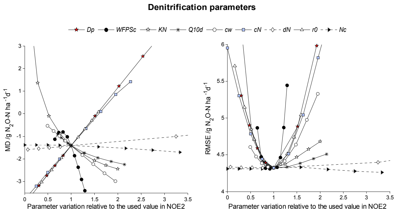
Figure 7: Sensitivity analysis of NOE2 when the values of denitrification parameters vary: mean difference (MD, left graph) and root mean square error (RMSE, right graph). MD and RMSE were calculated for the 16 sequences (= 4 periods * 2 treatments * 2 years). The x axis represents the ratio of the parameter value to its nominal value.
