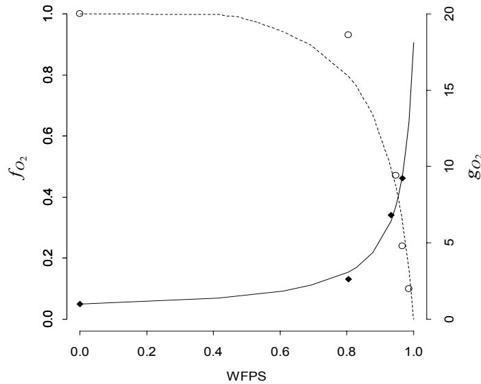
Figure 1 Functions simulating the effect of anoxia ( WFPS ) on the nitrification rate ( f_{O_2} , dotted line) and the fraction of N_2O emitted per unit of N nitrified ( g_{O_2} , continuous line) in model NOE2 (see Eq. 16 and 23 in Table 1). The curves were fitted to the observed values (open and filled-up points, respectively) reported by Khalil et al. (2004).
