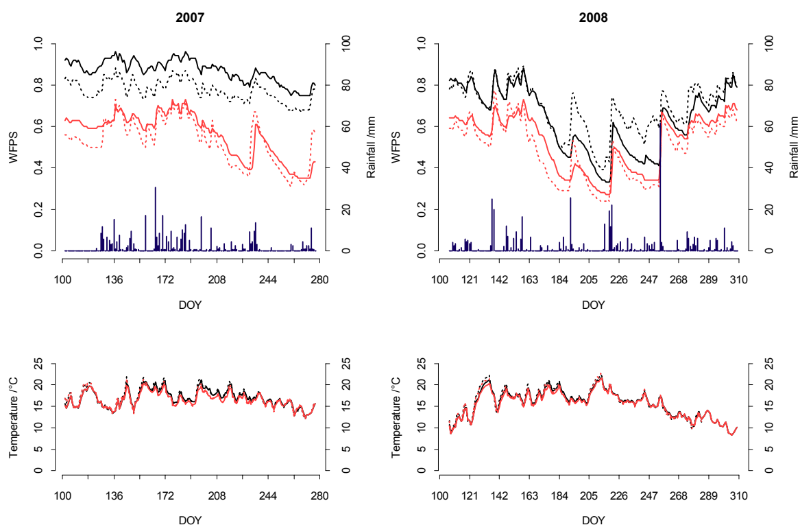
Figure 2 Evolution of rainfall, water-filled pore space ( WFPS ) and temperature in the soil at -10 cm (full lines) and -20 cm depth (dotted lines) in the compacted soil (black line) and uncompact soil (red line) cropped with sugar beet during 2007 and 2008.
