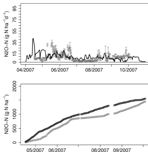
Figure A8-4: CERES-NOE2 (best set of parameter values) Simulated fluxes in black, observed in grey Compacted sugar beet plot in 2007 RMSEP (N 2 O daily emissions): 8.31 g N-N 2 O ha -1 d -1 RMSEP (cumulated N 2 O emissions): 207.91 g N-N 2 O ha -1
