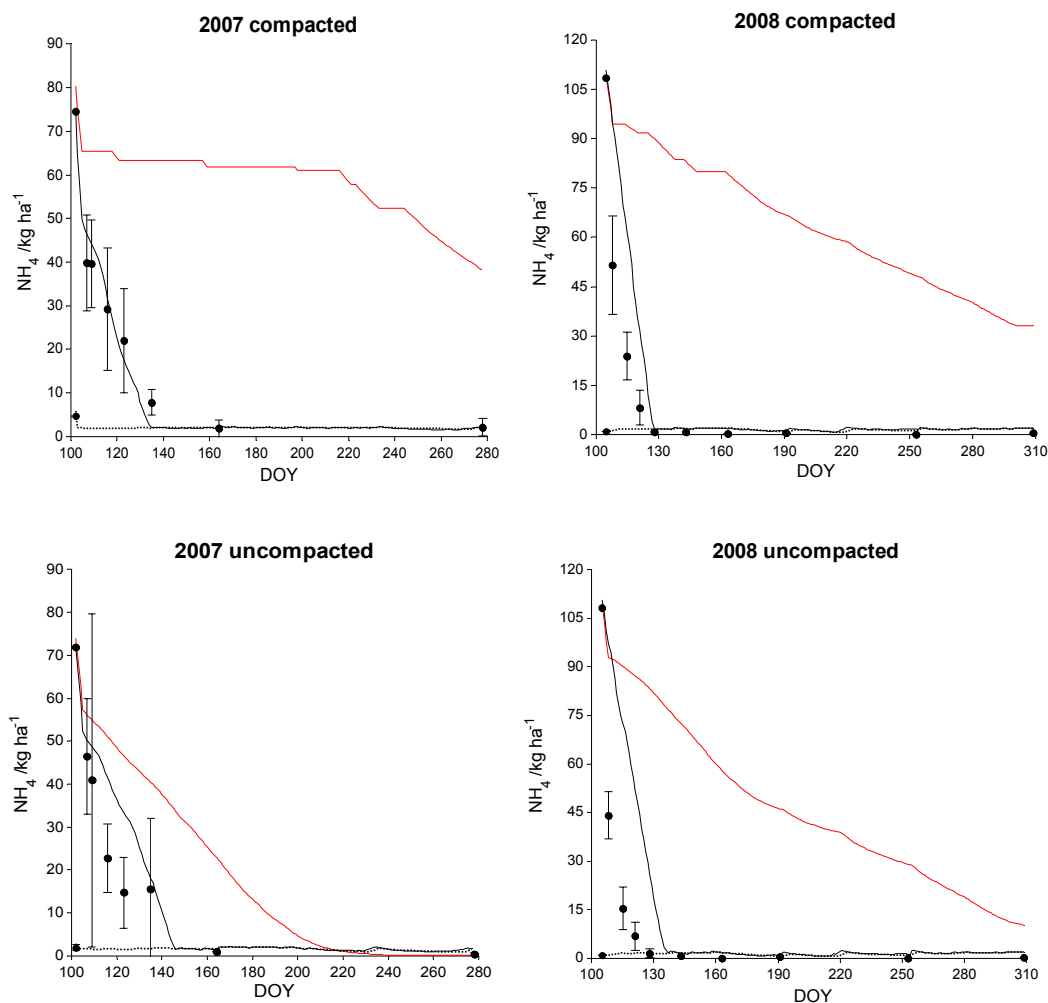
Figure 4 Observed (symbols) and simulated ammonium contents in soil over 0-10 cm (full lines) and 10-20 cm (dotted lines) in the two treatments during the two years. Simulations were run with NOE (red lines) and NOE2 (black lines). The error bars indicate the confidence intervals on measurements ( p < 0.05 ).
