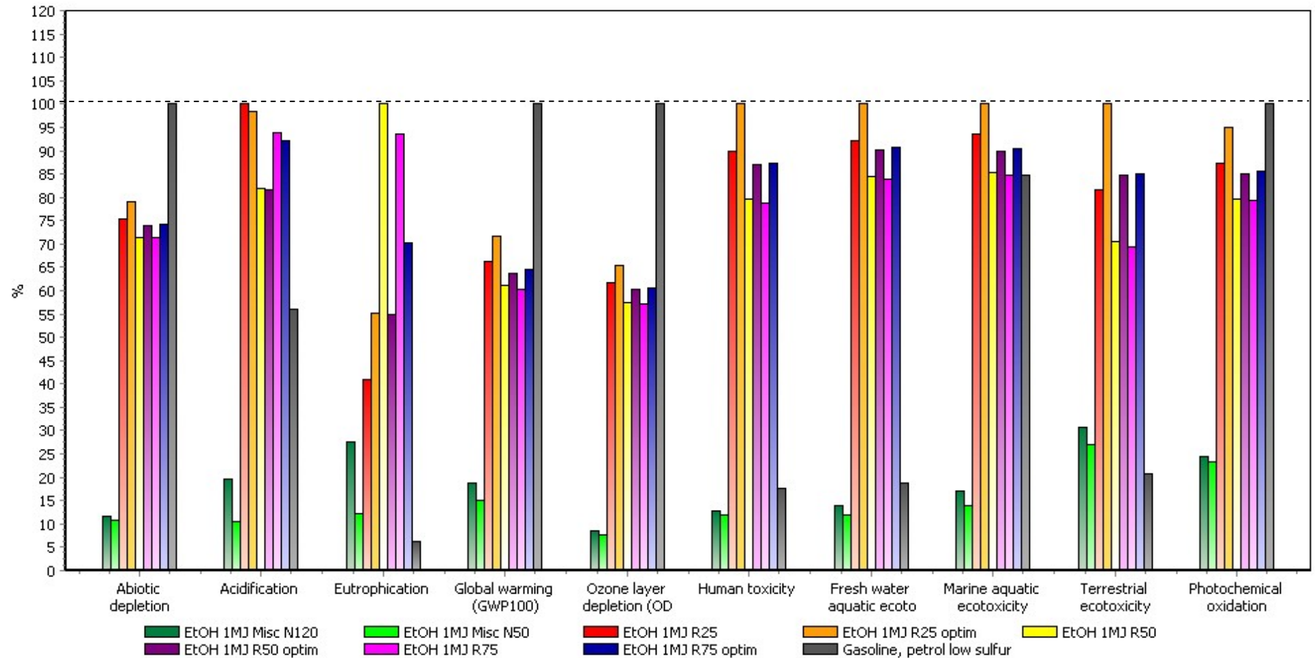
Figure 4: Comparison of the impact assessment with CML2 Baseline method on a MJ basis. Ethanol from sugar beet are in red, orange, yellow and pink (EtOH 1MJ R25-50-75, with optimized scenarios), Miscanthus two fertilizer levels are in green, and gasoline at the refinery doors in grey.
