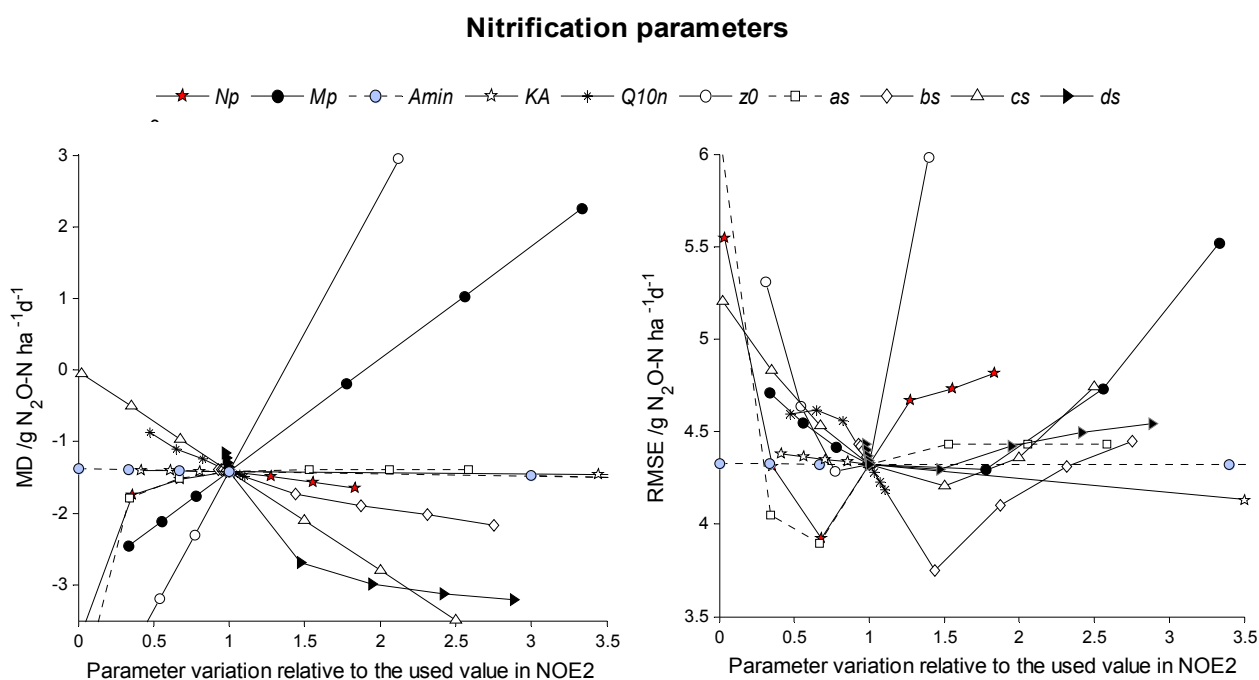
Figure 5 Sensitivity analysis of NOE2 when the values of nitrification parameters of vary: mean difference (MD, left graph) and root mean square error (RMSE, right graph). MD and RMSE were calculated for the 16 studied sequences (= 4 periods * 2 treatments * 2 years). The x axis represents the ratio of the parameter value to its nominal value.
