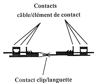
Figure 1.7: Contact clip-langue [1.9]
