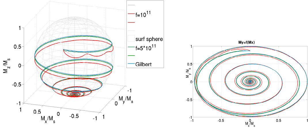
(a) The 3D trajectory of the magnetisation for different values of the frequency f .
