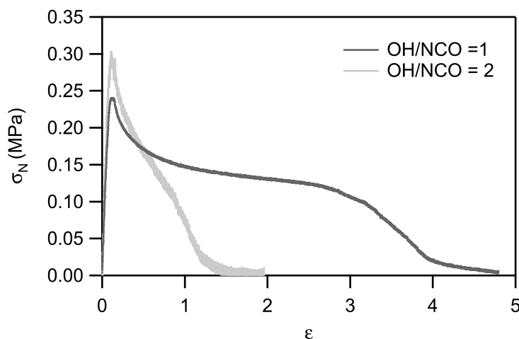
Figure 6-11 : Probe-tack curves of samples with HEMA/BPA=0.5 and different OH/NCO; V_{deb} = 10 \mu\text{m}\cdot\text{s}^{-1}
