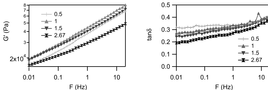
Figure 6-1 : Evolution of the elastic modulus G' (left) and of the phase angle \tan\delta (right) with frequency for different HEMA/BPA ratios; Strain \sim 8\%
