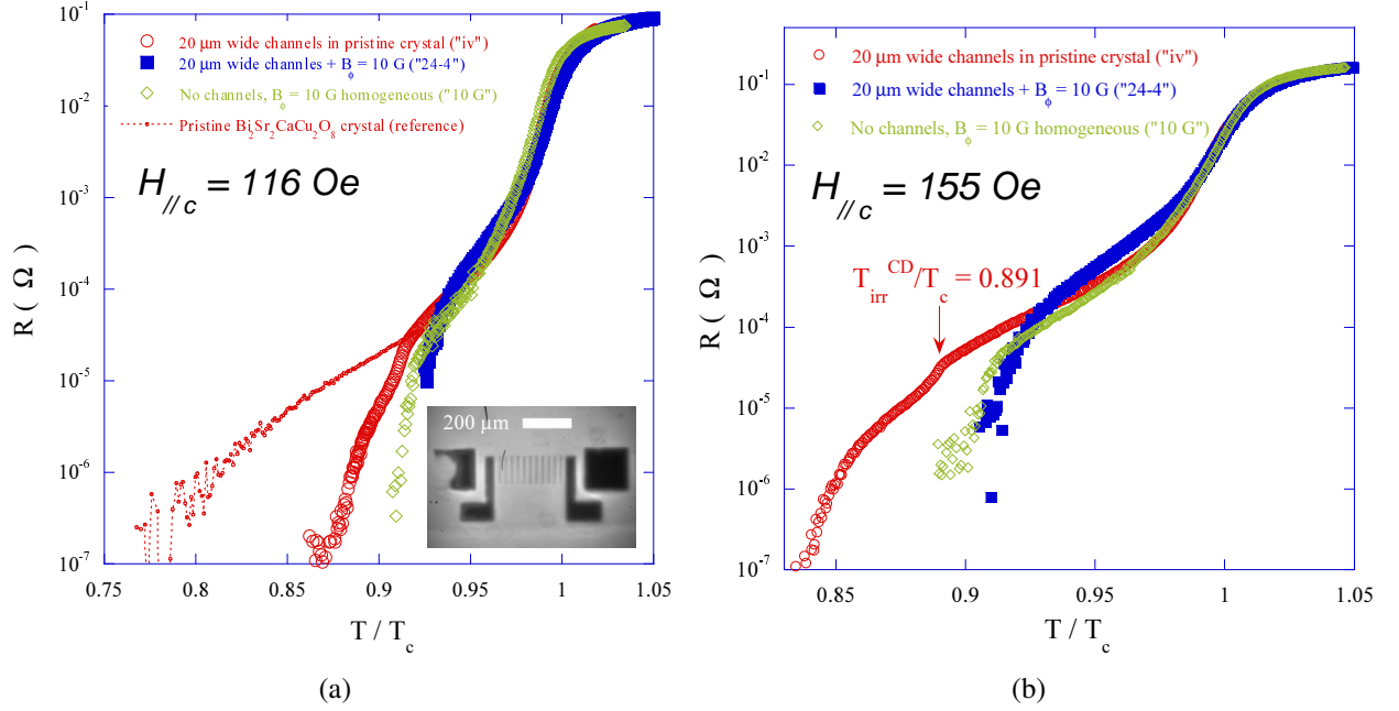
Figure 5.28: Renormalized resistance as a function of the temperature for three Bi_2Sr_2CaCu_2O_8 crystals. (a) Resistance data under the field H_{//c} = 116 Oe. The thin line presents the resistance data of a pristine sample under the same magnetic field (multiplied by a factor of 0.024 for comparison). It shows the continuation of the resistance for a sample without confinement effect. Inset: direct magneto-optical image of the central part of the crystal BSCCO "24-4", taken as T = 35 K and an applied field H_{//c} = 456 Oe. The bright regions correspond to those parts of the crystal that are penetrated by the magnetic field and the dark regions are the irradiated areas that screen the magnetic field. (b) Resistance data under the field H_{//c} = 155 Oe.
