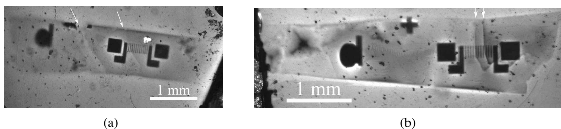
Figure 5.18: Channel structure perturbed by surface steps, marked by the arrows. (a) Direct MO image taken at T = 32.66 K, H_{//c} = 333 Oe in sample BSCCO 23-2 . (b) Direct MO image taken at T = 25.93 K, H_{//c} = 274 Oe in sample BSCCO "26" .
