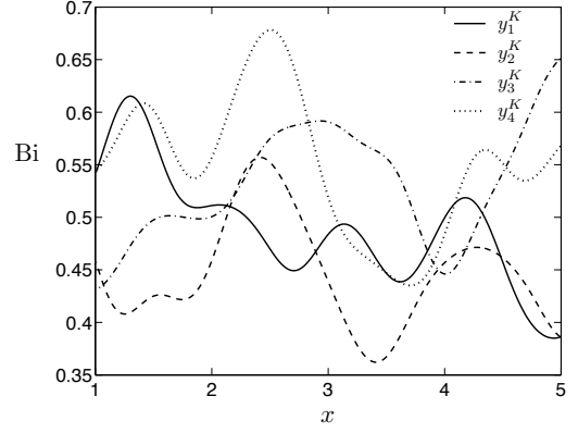
FIG. 6.3 – Four realizations of the Biot number x \rightarrow \text{bi}(x; \overline{\text{Bi}}=0.5, y_i^K) - 1 \leq i \leq 4 .
