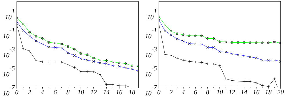
FIG. 7.9 – Algorithm 1 for FENE model with b=9 : Minimum + , mean \times and maximum \circ of the absolute variance (7-IV.8) in samples of parameters (left : offline sample \Lambda_{\text{trial}} \setminus \{\lambda_i, i=1, \dots, I\} ; right : online sample \Lambda_{\text{test}} ) with respect to the size I of the reduced basis.
