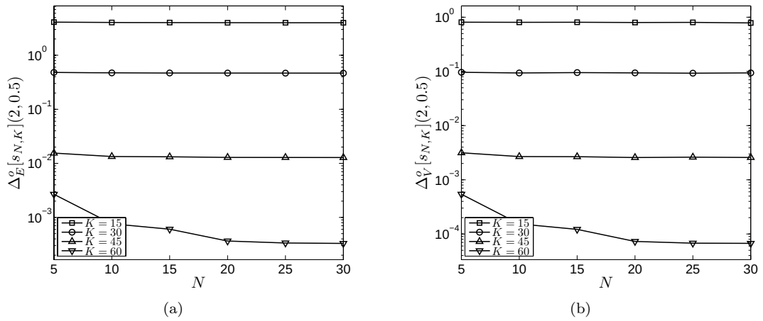
FIG. 6.13 – (a) \Delta_E^o[s_{N,K}(\mathcal{M}_K)] and (b) \Delta_V^o[s_{N,K}(\mathcal{M}_K)] as functions of N and K with \delta = 0.2 , \Upsilon = 0.074 and \varrho = (2.0, 0.5) .
