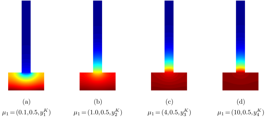
FIG. 6.4 – The temperature field u_{N,K}(\mu_i) for four different realizations \mu_i = (\kappa_i, \overline{\text{Bi}}=0.5, y_i) - 1 \leq i \leq 4 – when K = \mathcal{K} , corresponding to the four realizations of \text{bi}(\cdot; \overline{\text{Bi}}=0.5, y_i^K) in Figure 6.3.
