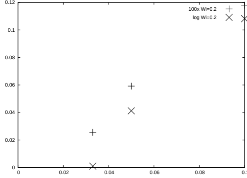
FIG. 2.5 – Relative errors for the stationary free energy at Wi = .2 with numerical schemes for \psi_h and \sigma_h (then multiplied by 100 in the latter case), with respect to the size h of the mesh.
