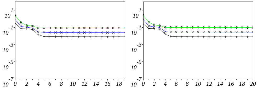
FIG. 7.10 – Algorithm 1 for FENE model with b=4 : Minimum + , mean \times and maximum \circ of the absolute variance (7-IV.8) in samples of parameters (left : offline sample \Lambda_{\text{trial}} \setminus \{\lambda_i, i=1, \dots, I\} ; right : online sample \Lambda_{\text{test}} ) with respect to the size I of the reduced basis.
