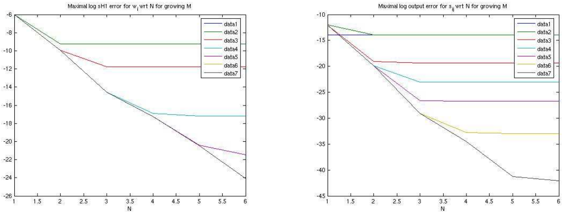
FIG. 5.6 – Left : maximal H^1 error for the RB approximations w_{N,M}(x, \cdot) in a random test sample using empirical interpolation and magic points with different M , with respect to the size N of the reduced-basis. Right : maximal L^\infty error for the RB approximations s_{N,M}(x) in the same random test sample of outputs s(x) using empirical interpolation and magic points with different M , with respect to the size N of the reduced-basis. The line termed data1 corresponds to M=1 , etc. until M=6 , and data7 corresponds to the error of the RB approximation without empirical interpolation.
