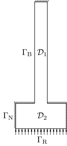
FIG. 6.1 – Geometry of the heat sink : a spreader \mathcal{D}_2 and a fin \mathcal{D}_1 .
