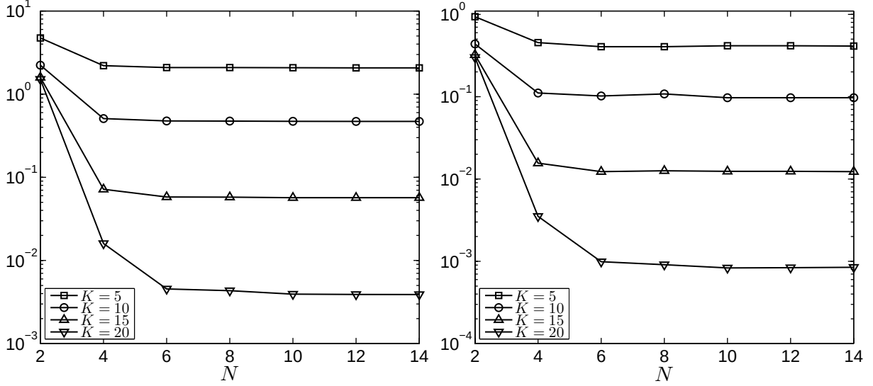
FIG. 4.5 – Global error bounds for the RB approximation error and the KL truncation error in the output expectation (left : \Delta_E^0(S_{K,N,N}) ) and the output variance (right : \Delta_V^0(S_{K,N,N}) ), as functions of the size N = 2, \dots, 14 of the reduced basis, at different truncation orders K = 5, 10, 15, 20 .
