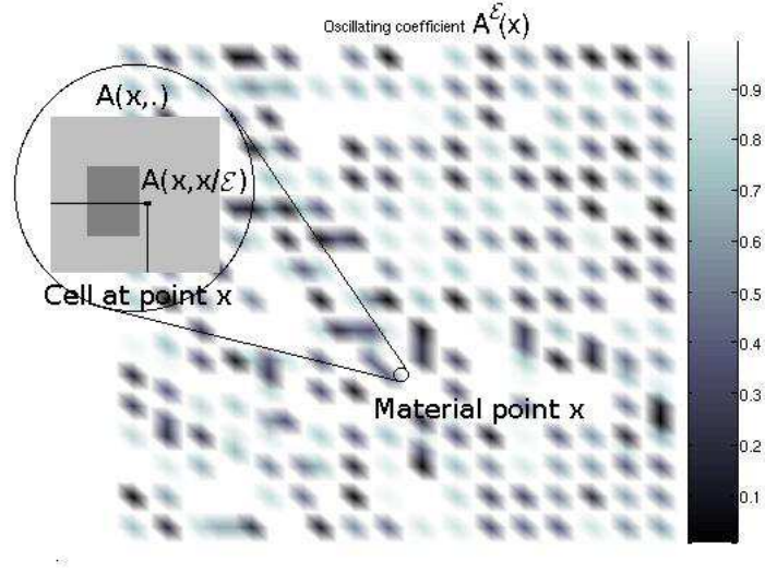
FIG. 4.3 – Example of fast oscillating coefficient \underline{A}_{i,i}^\epsilon : x \in \mathcal{D} \rightarrow \underline{A}_{i,i}^\epsilon(x) \in (0,1) , i=1,2 .
