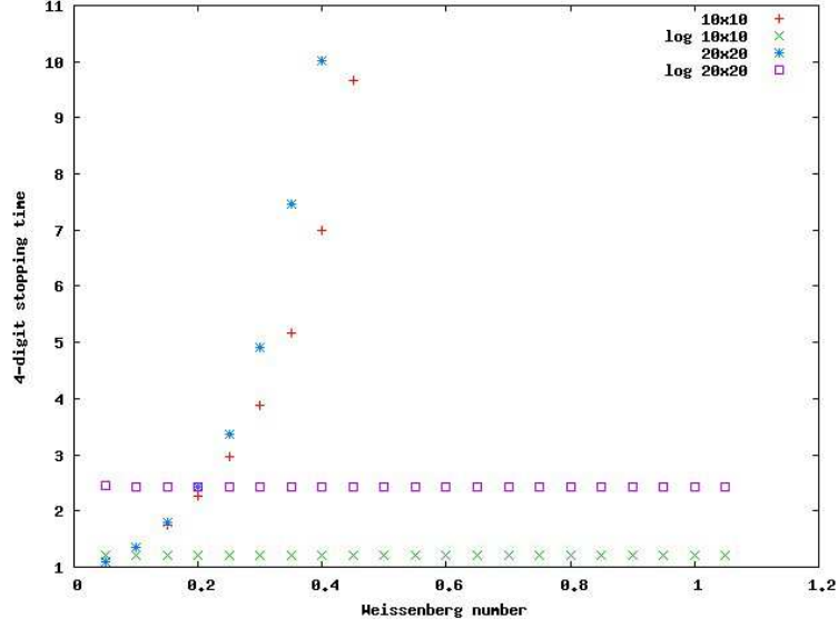
FIG. 2.1 – First time when the four digits in the L^\infty norm of the three fields (\mathbf{u}, p, \boldsymbol{\sigma}) seem stabilized (that is, do not evolve after three consecutive steps), with respect to the Weissenberg numbers, for two meshes : h = .1 ( 10 \times 10 ) and .05 ( 20 \times 20 ). Also for (\mathbf{u}, p, \boldsymbol{\psi}) , using the log-formulation (log 10 \times 10 and log 20 \times 20 ).
