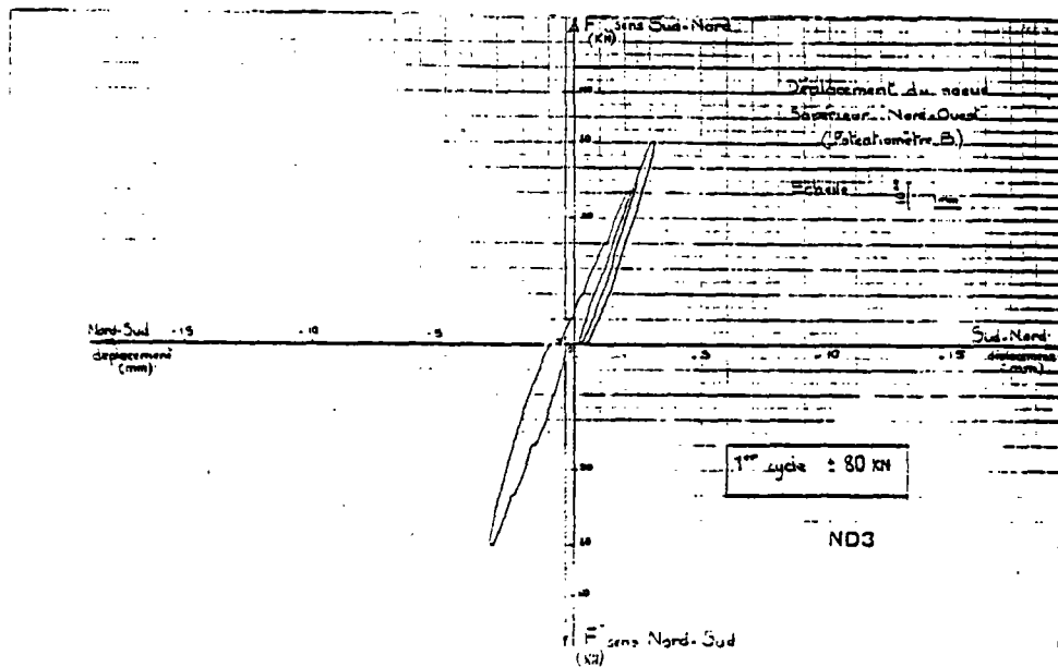
Fig. 3.3.3.1. - COURSE FORCE - DEPLACEMENT
