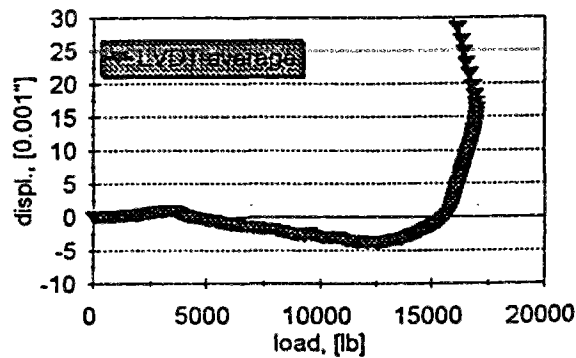
Figure 2 : Test Results; Concrete Compressive Strength 5300 psi (Oregon State University)
