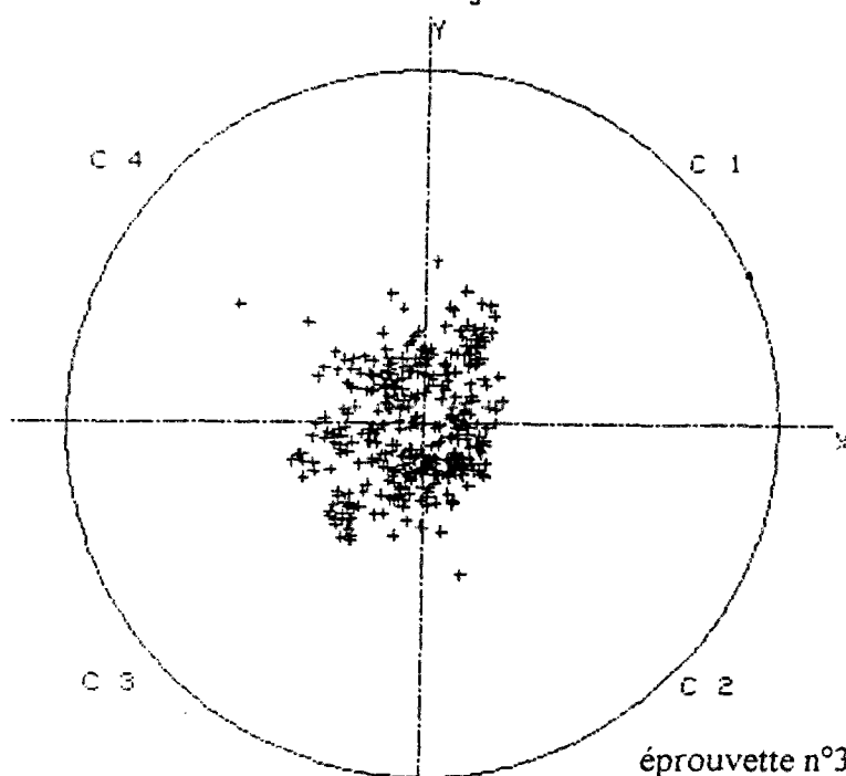
Figure 30 : Localisation plane
