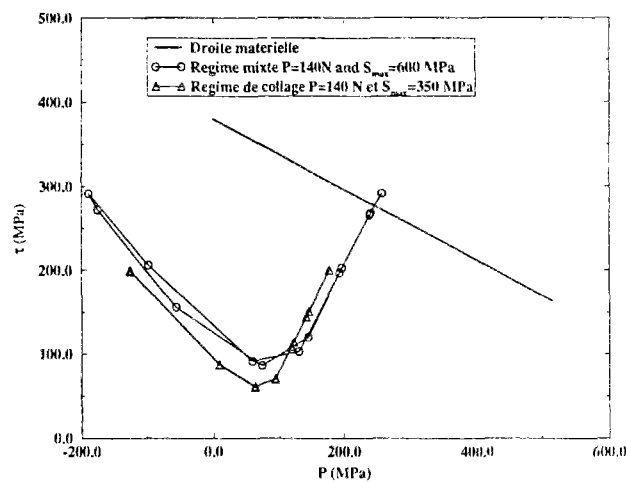
Figure 2.11: Diagrammes de Dang Van
