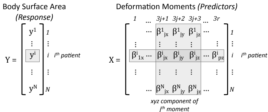
Figure 6.14: Matrices of BSA, Y , and centred moment vectors that parameterise the deformations, X .
