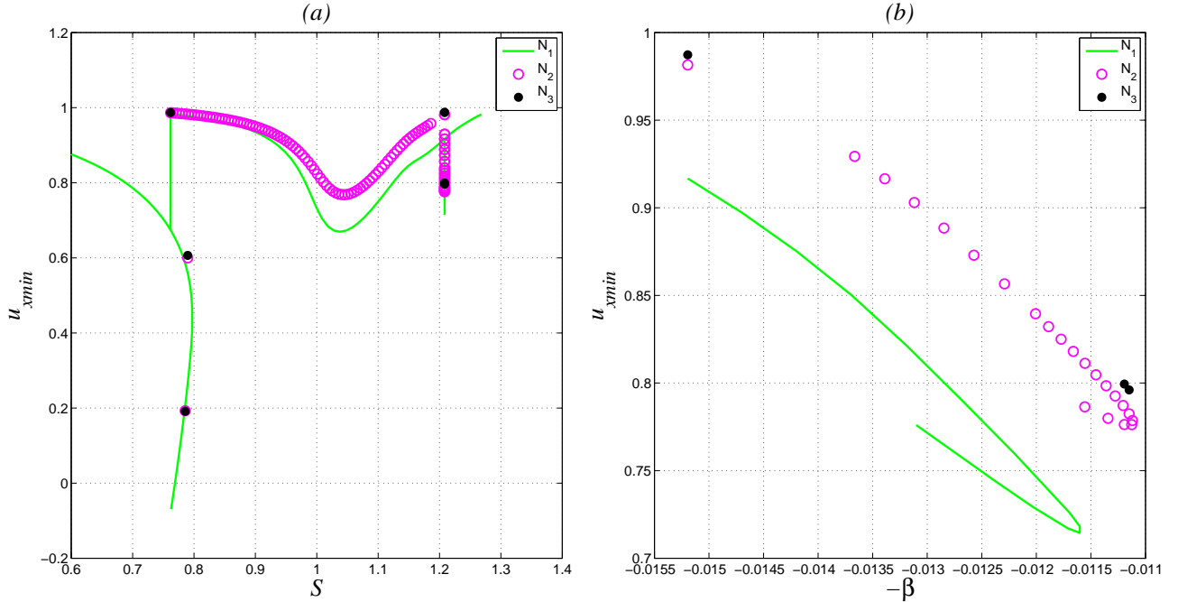
Figure 4.3: Bifurcation diagram for Re = 1000 : on the left the minimum axial velocity u_{xmin} is plotted as a function of the swirl number S ; on the right u_{xmin} is plotted as a function of the \beta for S = 1.2 . According to the theoretical prediction the solutions across the gap are linked to each other through homotopy in \beta . Green line corresponds to grid N_1 ( N_R = 127 , N_x = 257 ), magenta circles correspond to grid N_2 ( N_R = 253 , N_x = 513 ) and black dots correspond to grid N_3 ( N_R = 379 , N_x = 769 ).
