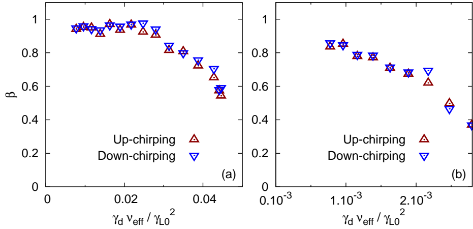
Fig. 4.13: Correction to Eq. (4.7) when the time-scale of frequency shift is relatively short compared to the bounce period, measured in \delta f simulations with \gamma_{L0} = 0.1 . The ratio \gamma_d/\nu_{\text{eff}} is such that \delta\omega(1/\nu_{\text{eff}}) = 0.2 in Eq. (4.7). (a) In the Krook case, spectrograms for two extreme points are shown in Fig. 4.12. (b) With drag and diffusion, \nu_f/\nu_d = 0.1 .
