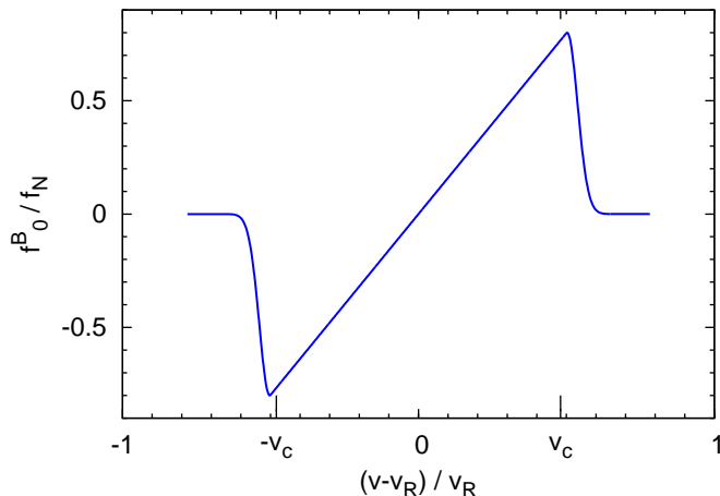
Fig. 3.2: Initial velocity distribution function, normalized to f_N \equiv \gamma_{L0}/(\sqrt{2\pi}v_R) .
