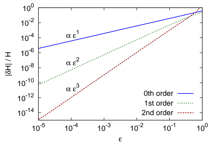
Fig. A.2: Relative error in total energy conservation for solutions obtained with Lie perturbation theory at t = 12.5\pi . For small \epsilon , solid, dotted, and dashed lines scale as \epsilon , \epsilon^2 , and \epsilon^3 , respectively.
