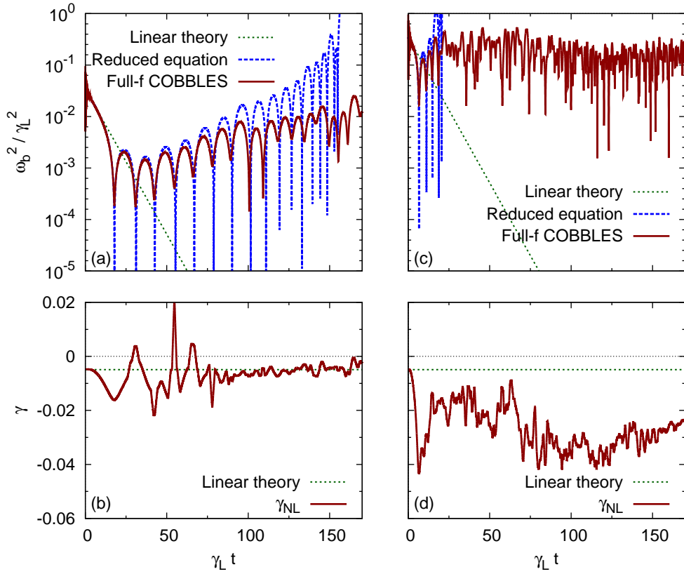
Fig. 4.20: (a) and (c) Time-evolution of electric field amplitude obtained by linear theory (dotted line), by solving Eq. (4.3) (dashed line), and by solving the full- f initial value problem (solid line). (b) and (d) Dynamic estimation of nonlinear growth rate (solid line). Dotted horizontal line is the value predicted by linear theory.
