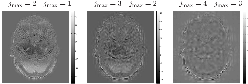
Figure 4.11: Influence of the number of resolution levels on the anatomical reconstructed images using our CWR-SENSE method for R = 4 ; from left to right: reconstructed images with j_{\max} = 2 - j_{\min} = 1 , j_{\max} = 3 - j_{\min} = 2 and j_{\max} = 4 - j_{\min} = 3 .
