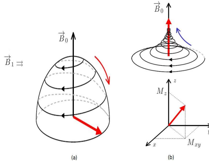
Figure 2.2: Precession movement of the magnetic moment.
