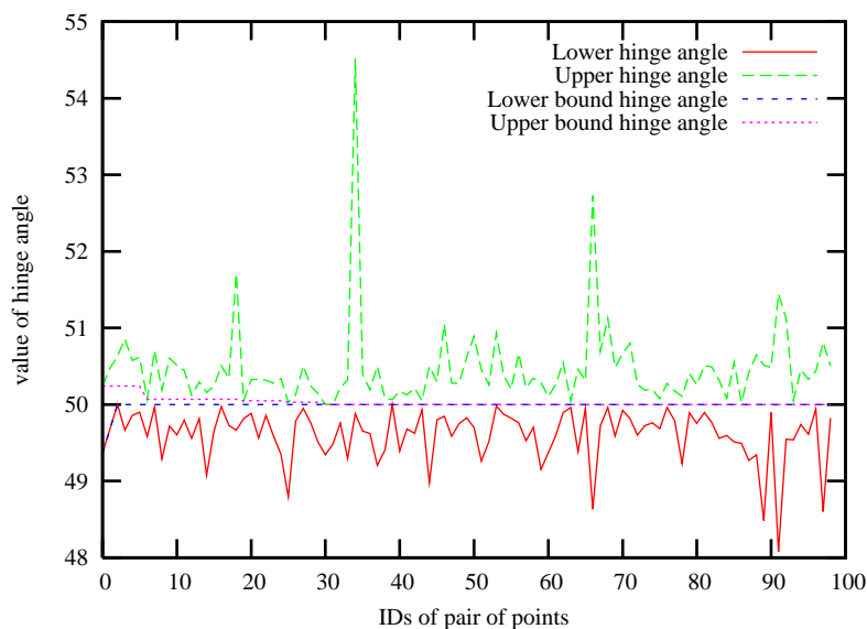
FIGURE 3.6: Result of our algorithm applied on the sets of points in Figure 3.5 .
