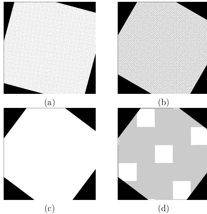
FIGURE 2.2: The DER rotation of a white image by the four angles (a) \alpha = 15^\circ , (b) \alpha = 30^\circ , (c) \alpha = \sin^{-1} \frac{3}{5} \approx 36.87^\circ and (d) \alpha = 37^\circ
