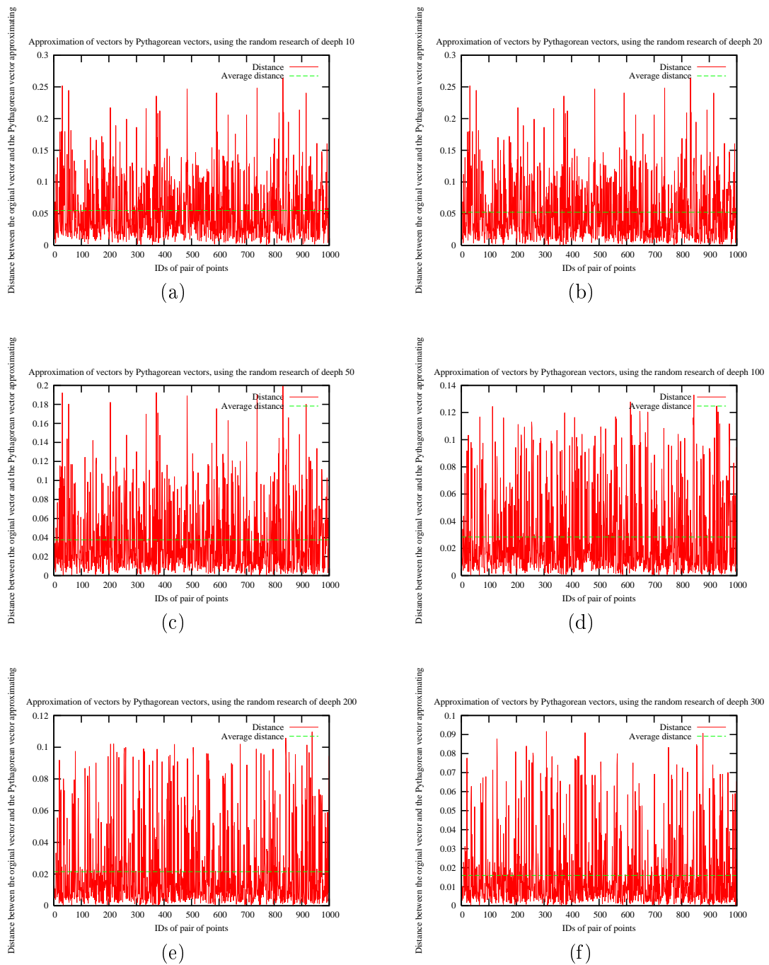
FIGURE 6.14: Distance between 1000 vectors and their approximated Pythagorean vector for a random Pythagorean tree of depth 10 (a), of depth 20 (b), of depth 50 (c), of depth 100 (d), of depth 200 (e) and of depth 300 (f)
