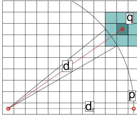
FIGURE 3.10: Problem of corresponding points with real data.
