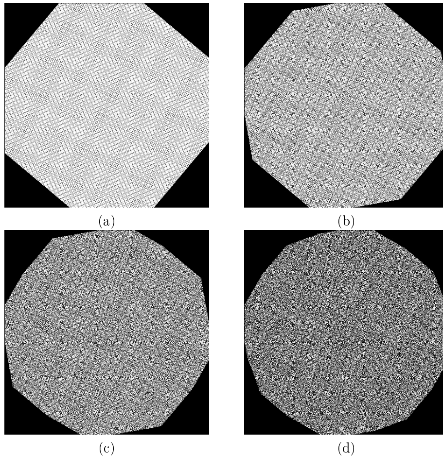
FIGURE 2.4: During the composition of DER, the number of points lost due to double point is cumulative. For an angle \alpha = 40^\circ we lost approximately 15% of points for (a), 28% for (b), 39% for (c) and 50% for (d).
