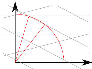
FIGURE 5.2: In a rational multi-grid \mathcal{M}^{A,\vec{p}} a convexels can have four intersections with the locus of rotation of \vec{p} .
