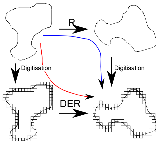
FIGURE 2.5: If a discrete rotation is DER-like, then the red way that discretize then rotate will gives the same result than the blue way that rotate then discretize.
