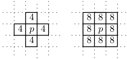
FIGURE 4.3: Left: 4-neighborhood of p represented by boxes labeled by 4 or p . Right: 8-neighborhood of p represented by boxes labeled by 8 or p .
