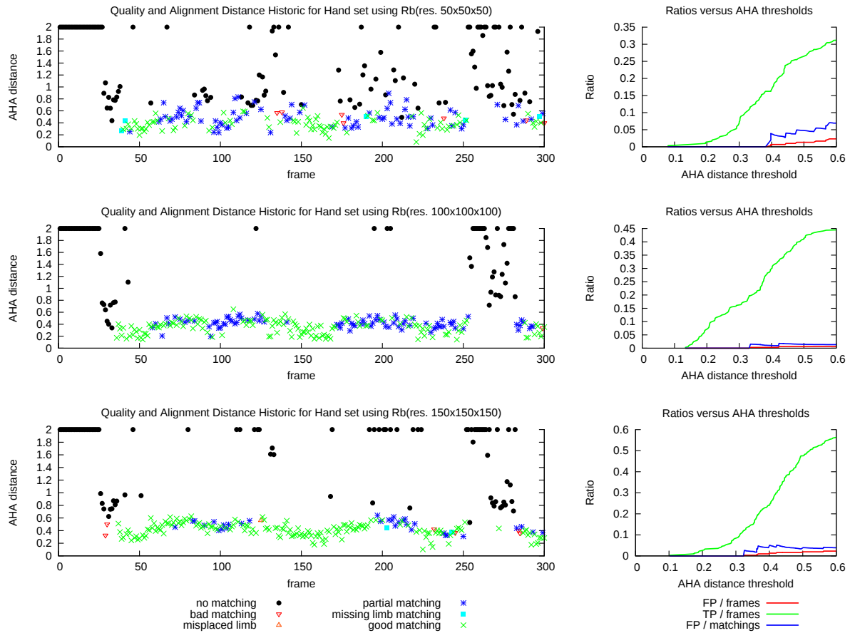
FIGURE 13.6: Study of correlations between AHA distance and matching quality for hand data set with different grid resolutions, using betweenness relation R_b . Left: historic of AHA distances and matching qualities all along the sequence. Right: different ratios in regard of given AHA distance threshold. From top to bottom: for resolutions 50^3 , 100^3 and 150^3 .
