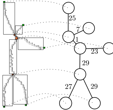
FIGURE 7.11: Left: example of connected components, each rectangle representing a connected component (CC). In this example, there is five E -points CC, seven B -points CC and two I -points CC. Right: data tree constructed from the skeleton at left. Dot lines show the CC associate to each vertex.
