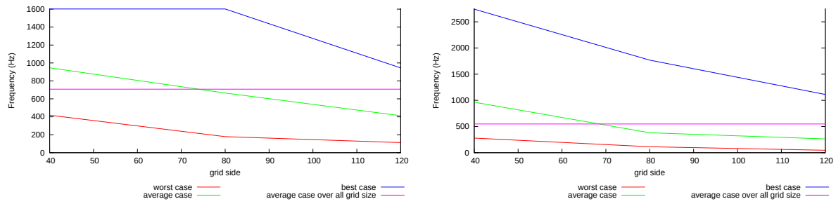
FIGURE 11.14: Average frequencies of asymmetric homeomorphic alignment for different sizes of grid. Left: in full human body context. Right: in hand context.
