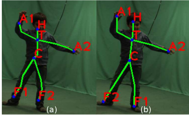
FIGURE 13.9: Sample of accuracy difference of pose estimation for different grid resolutions: (a) 50 \times 50 \times 50 resolution, (b) 150 \times 150 \times 150 resolution.
