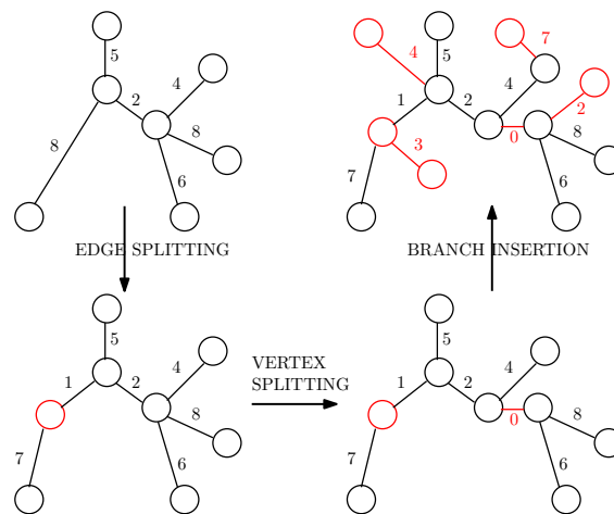
FIGURE 11.1: Illustration of structural noise generation.
