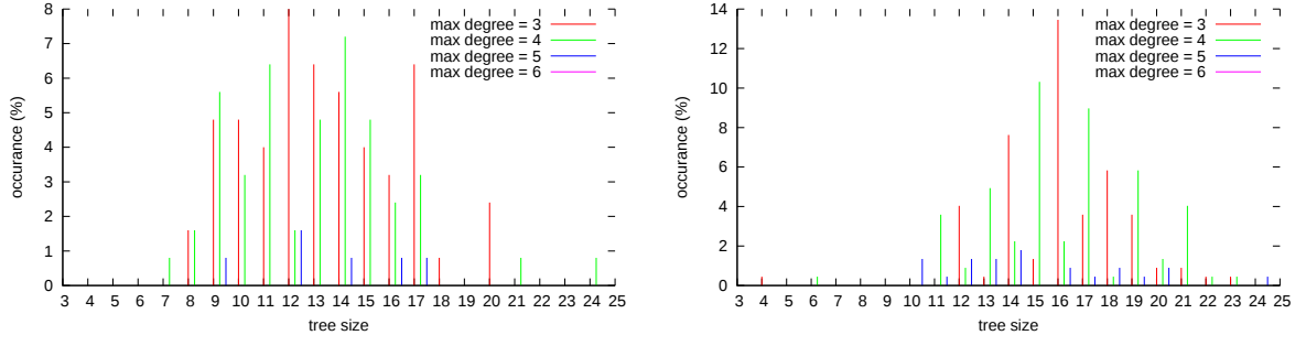
FIGURE 11.10: Distributions for a grid sided by 120. Left: dancer data set. Right: hand data set.
