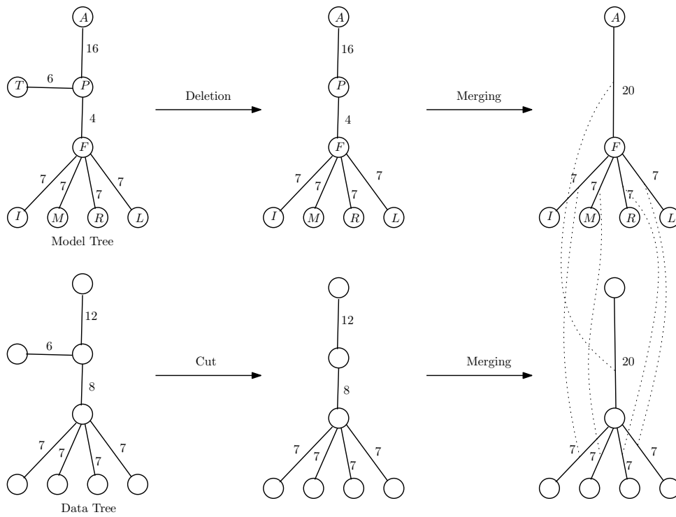
FIGURE 9.10: Example of bad homeomorphic alignment matching due to merging on model tree: the "thumb" edge is removed for a cost of 6, as the merging of "arm" edge and "palm" edge in both trees reduce the matching cost by 8.
