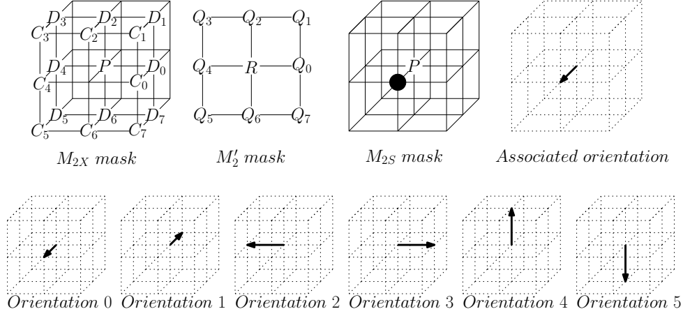
FIGURE 5.5: New masks for 2-crucial points detection, and all possible orientations of these masks.
