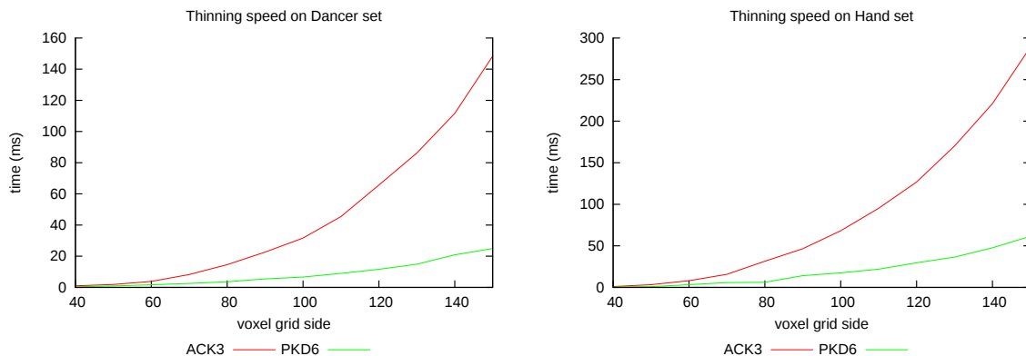
FIGURE 5.13: Thinning speed of fully optimized ACK3 and PKD6 on two data sets.
