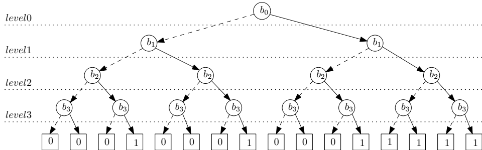
FIGURE 5.2: A binary decision tree containing the results of the function f .
