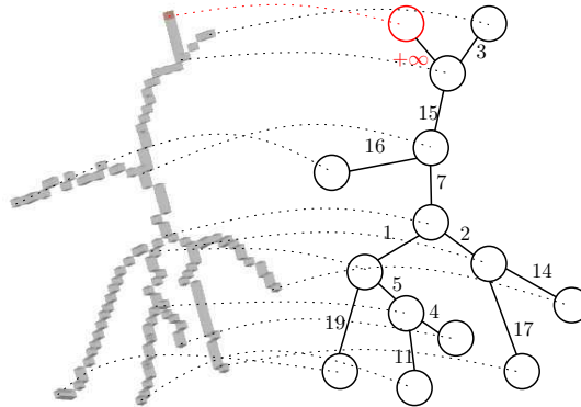
FIGURE 7.12: Example of data tree construction for incomplete model. Left: hand skeleton, with in orange, a border point. Right, the data tree constructed from the skeleton.
