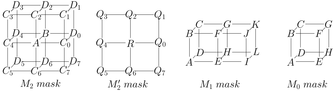
FIGURE 5.4: Masks used for crucial cliques detection.
