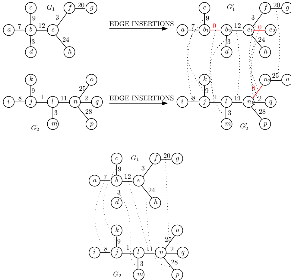
FIGURE 8.13: Example of alignment for weighted trees. Top left: initial trees G_1 and G_2 . Top right: trees after edge insertions G'_1 and G'_2 , dotted lines representing the alignment. Bottom: associated alignment mapping of G_1 and G_2 .
