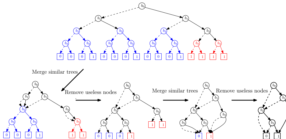
FIGURE 5.3: Transformation of a binary decision tree into a binary decision diagram.
