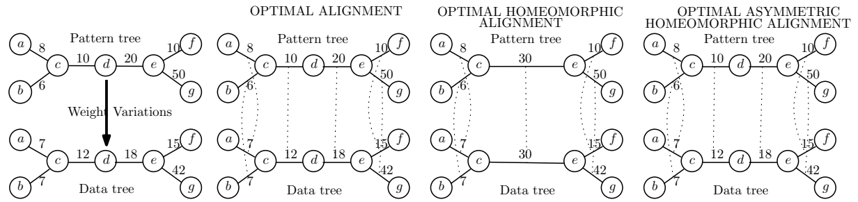
FIGURE 11.6: Example where alignment provide better result than homeomorphic alignment.
