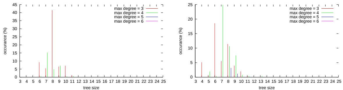
FIGURE 11.8: Distributions for a grid sided by 40. Left: dancer data set. Right: hand data set.
