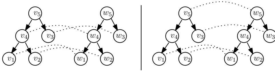
FIGURE 8.11: At left: a mapping which is bottom up. At right: a mapping which is not bottom up.
