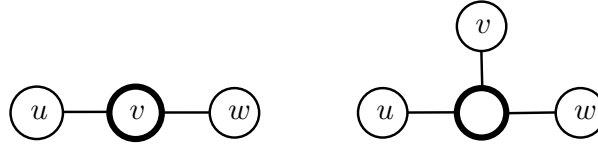
FIGURE 8.7: Illustrations of the center, represented by the bold circle.
