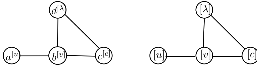
FIGURE 7.7: Example of labeled graph representation. In order to avoid confusion with vertex identifier, the label associated to each vertex is write between brackets. In the case where the identifier must be represented, we use the representation shown on the left graph: the identifier with the label between brackets in exponent. In other case, we just write the label between brackets, like in the right graph.
