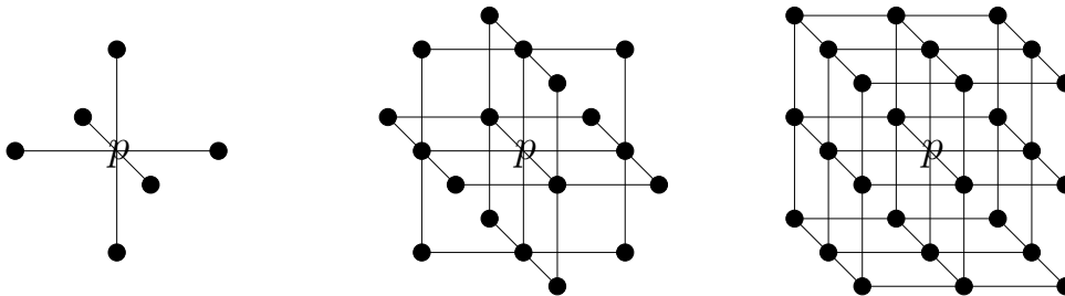
FIGURE 4.4: From the left to the right: 6-neighborhood, 18-neighborhood and 26-neighborhood of point p , represented by black disks and p .
