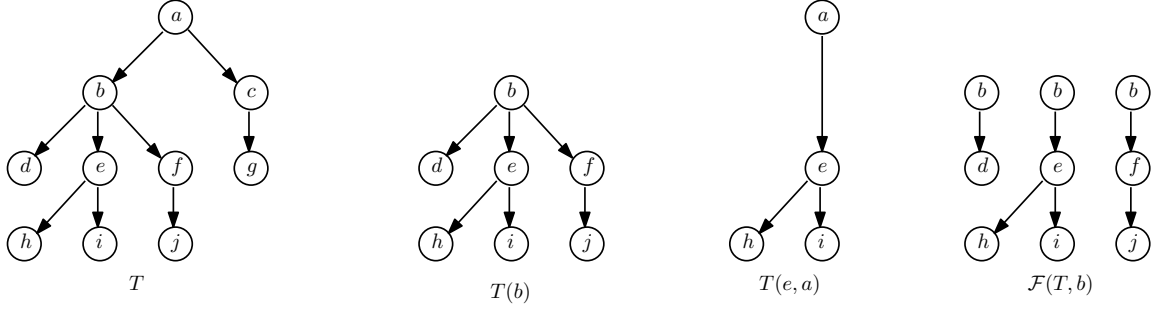
FIGURE 9.7: From the left to the right: a tree T , a subtree of T rooted in b , a subtree of T rooted in a and pruned in e , and a forest of T with origin b .
