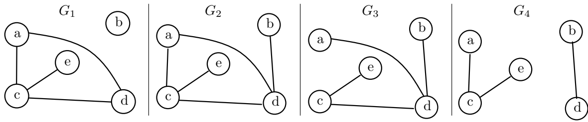
FIGURE 7.2: From the left to the right, four undirected graphs: G_1, G_2, G_3 and G_4 . G_2 and G_3 are connected, contrary to G_1 and G_4 . G_3 is a tree, contrary to the three others. G_3 and G_4 are forests, composed respectively by one and two trees.
