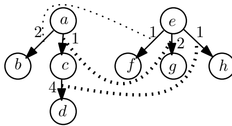
FIGURE 8.4: An invalidate mapping: the ancestor condition is not respected (due to bold pair: c is an ancestor of d , contrary to g which is not an ancestor of h ).
