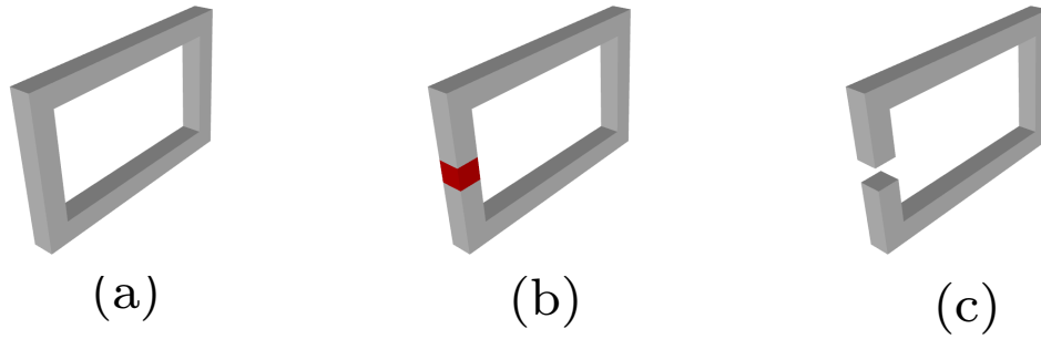
FIGURE 4.5: (a) A shape with a tunnel. (b) Deletion of the red point. (c) The shape has no tunnel.
