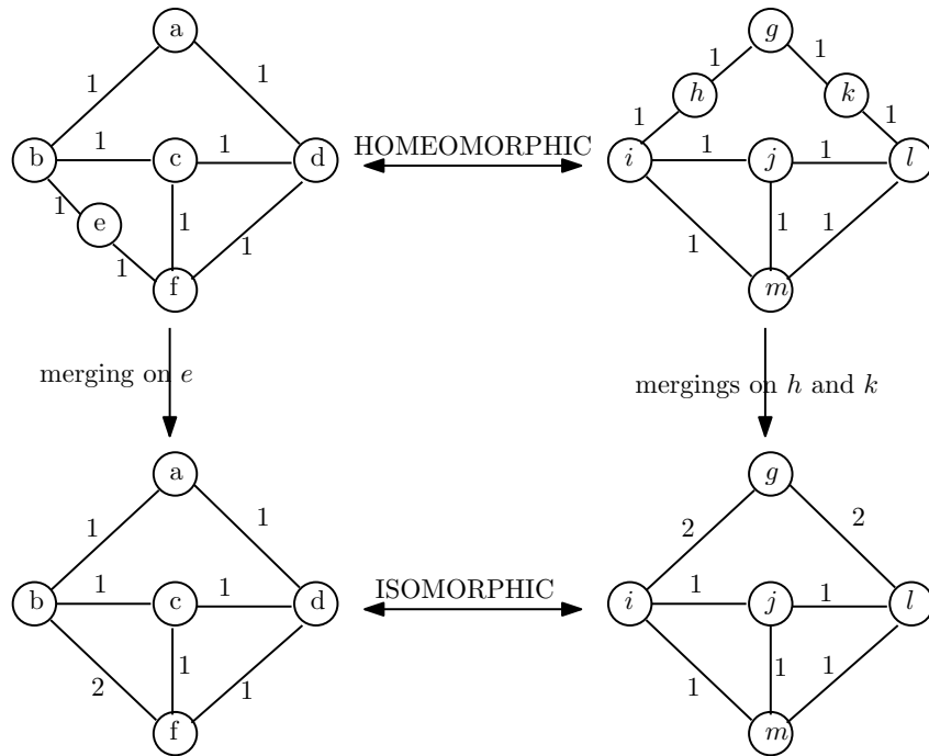
FIGURE 9.3: Examples of homeomorphism.
