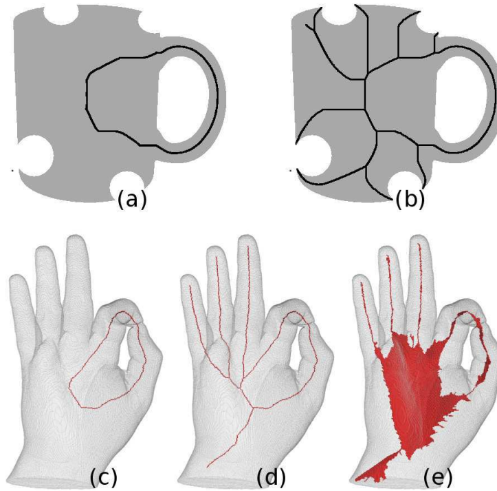
FIGURE 4.6: Examples of the different kinds of skeleton. Top, 2D skeletons: (a) ultimate skeleton, (b) curvilinear skeleton. Bottom, 3D skeletons: (c) ultimate skeleton, (d) curvilinear skeleton, (e) surface skeleton.
