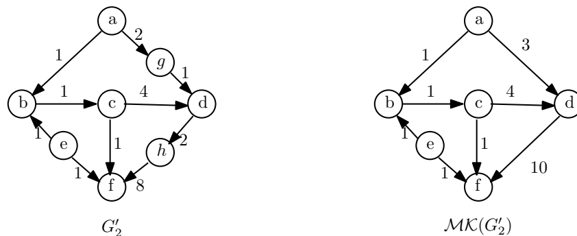
FIGURE 9.5: Example of merging kernel of a directed graph.
