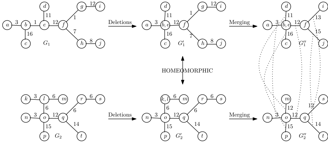
FIGURE 9.6: Example of homeomorphic alignment.
