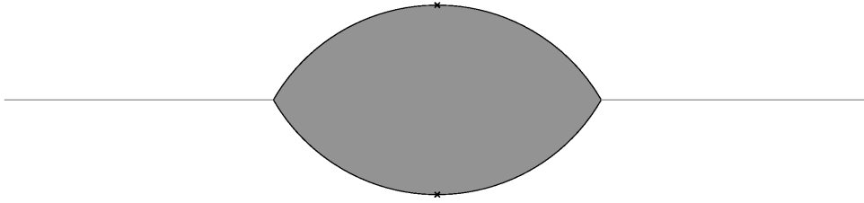
FIGURE 12.7: All points in the grey area are between the two points represented by black crosses (in the sense of R_i ).
