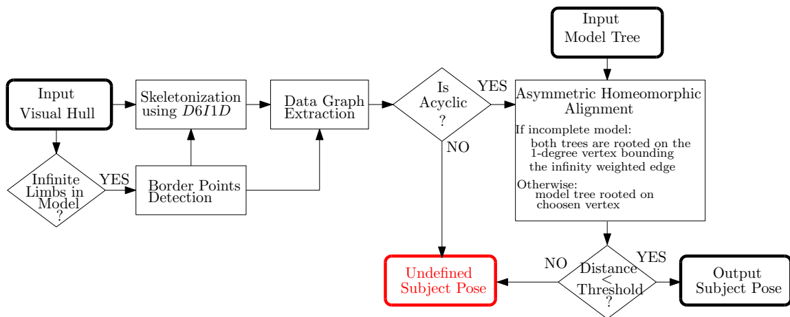
FIGURE 12.1: Detailed pipeline of our method. Rounded rectangles represent input and output data. Other rectangles represent steps of the method.
