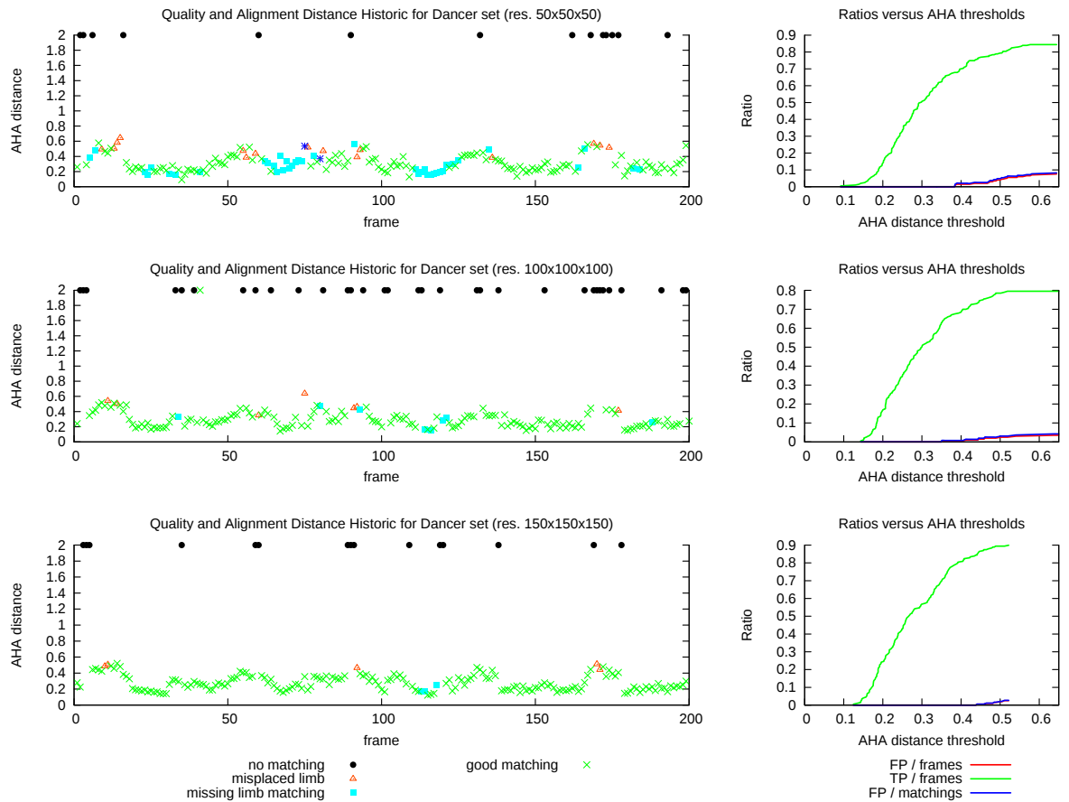
FIGURE 13.4: Study of correlations between AHA distance and matching quality for dancer data set with different grid resolutions. Left: historic of AHA distances and matching qualities all along the sequence. Right: different ratios in regard of given AHA distance threshold. From top to bottom: for resolutions 50^3 , 100^3 and 150^3 .
