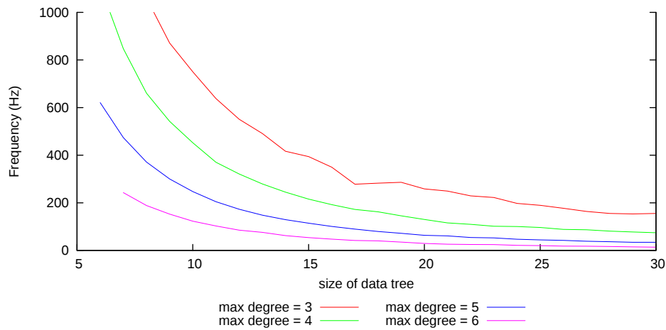
FIGURE 11.12: Frequencies of asymmetric homeomorphic alignment of hand rooted model tree with different rooted data trees.
