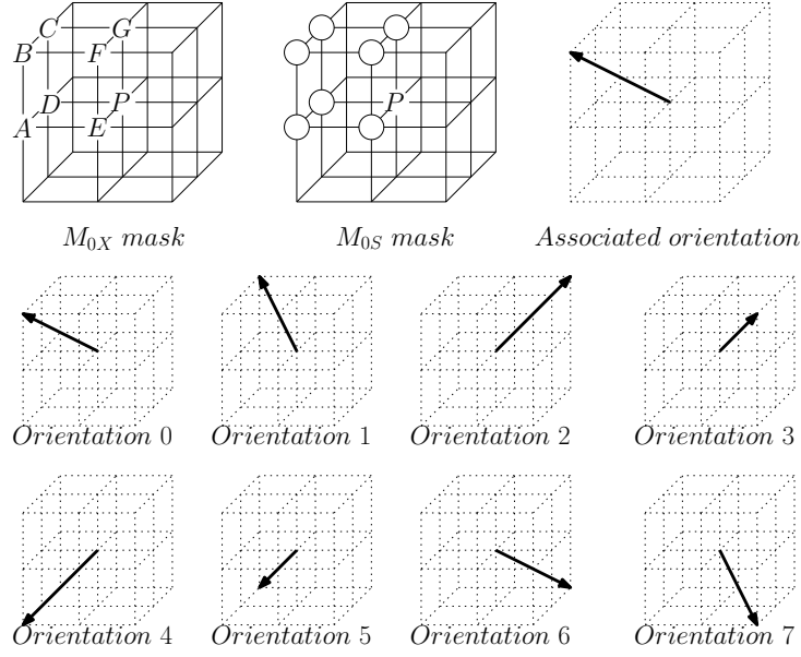
FIGURE 5.7: New masks for 0-crucial points detection, and all possible orientations of these masks.
