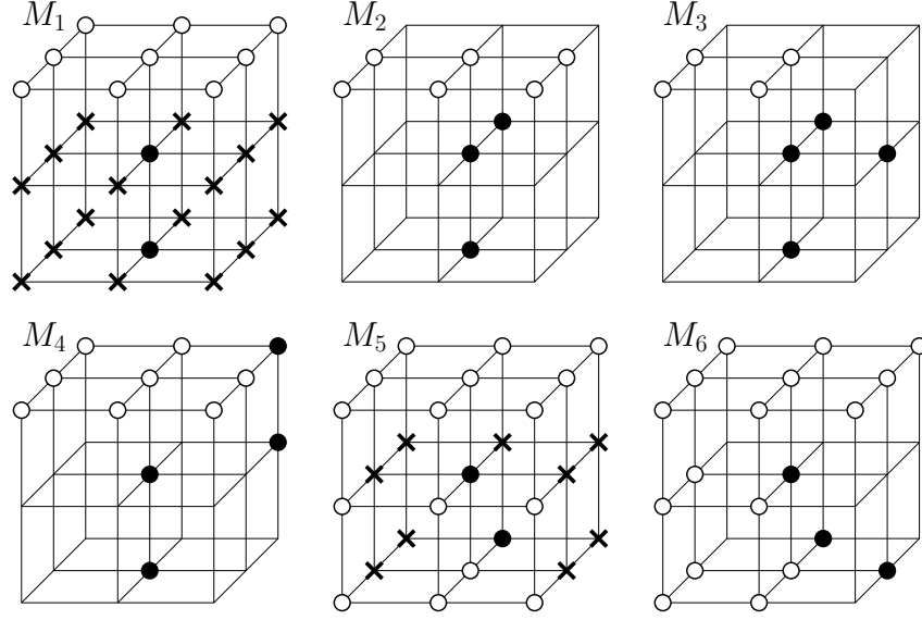
FIGURE 6.1: Base masks M_1 - M_6 and their rotations around the vertical axis form the set of masks \mathcal{M}_U for direction UP . Points marked by a black disk have to belong to the object, points marked by a white disk have to be out of the object, and at least one point marked by a cross in masks M_1 and M_5 has to belong to the object.
