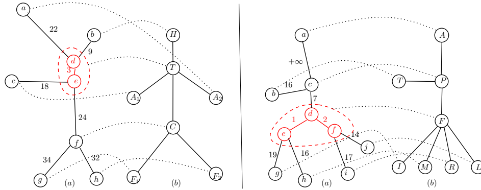
FIGURE 7.15: (a): data tree with splitted vertices (in red). (b): model tree to match. Dotted lines represent the expected matching.
