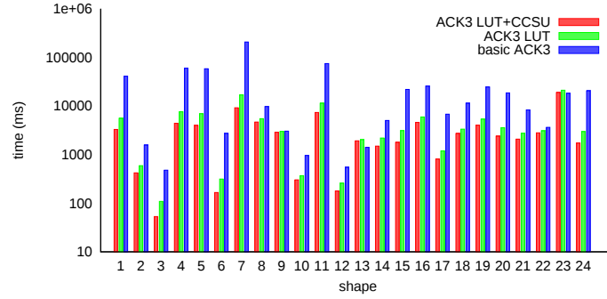
FIGURE 5.9: Computation speed results for ACK3 implemented with different levels of optimization, for each image of our test set.
