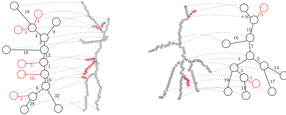
FIGURE 7.13: Examples of spurious branches and ghost limbs (in red) for a full human body shape (left) and a hand shape (right).
