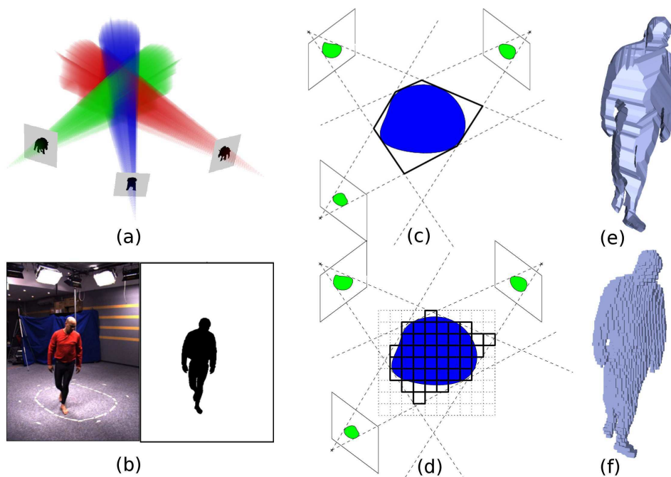
FIGURE 2.3: (a) Illustration of silhouette cones, reprinted from Matusick et al. paper [109]. (b) Example of input camera image and associated silhouette. (c) and (d) Illustrations of surface and volumetric visual hulls reconstructions, respectively: object is represented in blue, its silhouettes in green, silhouette cones by dashed lines, and result by bold lines. (e) and (f) surface and volumetric visual hulls of a same object, respectively. Figures (b), (e) and (f) are reprinted from Menier thesis [110].
