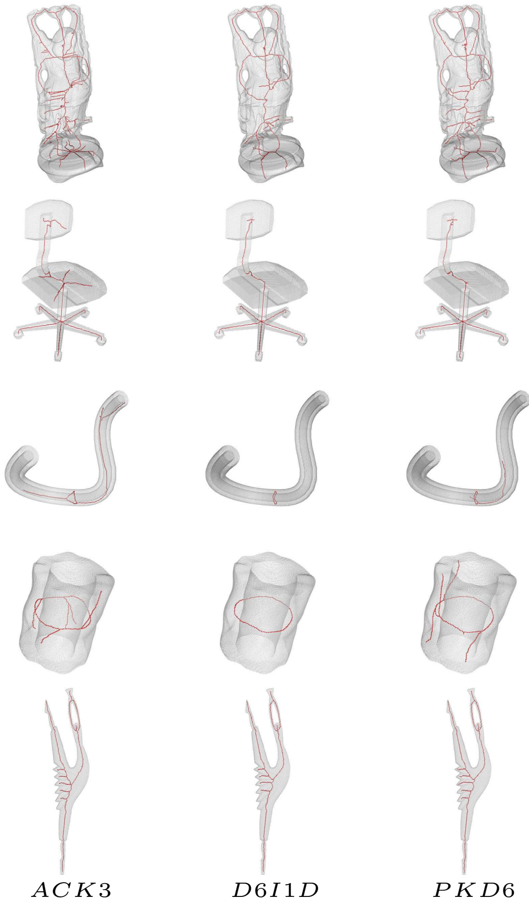
FIGURE 6.5: Skeletons resulting of different algorithms for several shapes. From the left to the right: algorithms ACK3, D6I1D, and PKD6. From the top to the bottom: shapes 4, 18, 23, 20 and 13.
