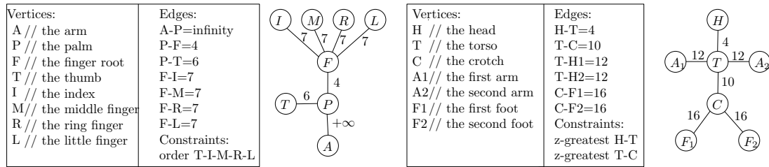
FIGURE 12.9: Full description of two different subjects. On the left, the hand model description (incomplete model). On the right, the full human body model description (complete model).
