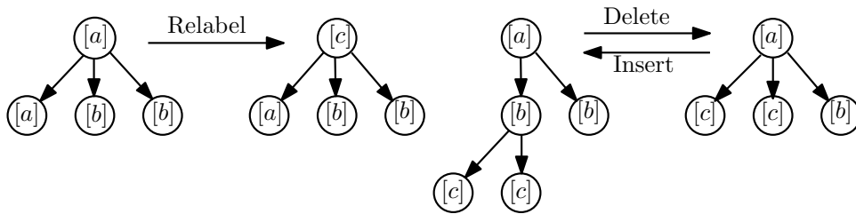
FIGURE 8.1: Examples of edit operations for labeled rooted trees.
