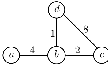
FIGURE 7.8: Example of weighted graph representation. Each number represent the weight of the closest edge.
