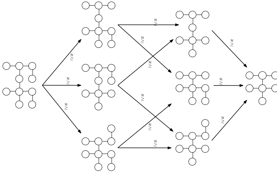
FIGURE 10.1: Example of asymmetric homeomorphic relations on a set of homeomorphic trees.
