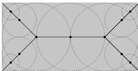
FIGURE 4.1: Example of skeleton in continuous framework. The shape (a rectangle) is represented in grey. The skeleton is represented by bold lines. Some maximal balls are represented by dashed lines, with their center represented by black points.
