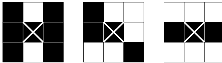
FIGURE 4.7: Examples of 1D isthmuses.
