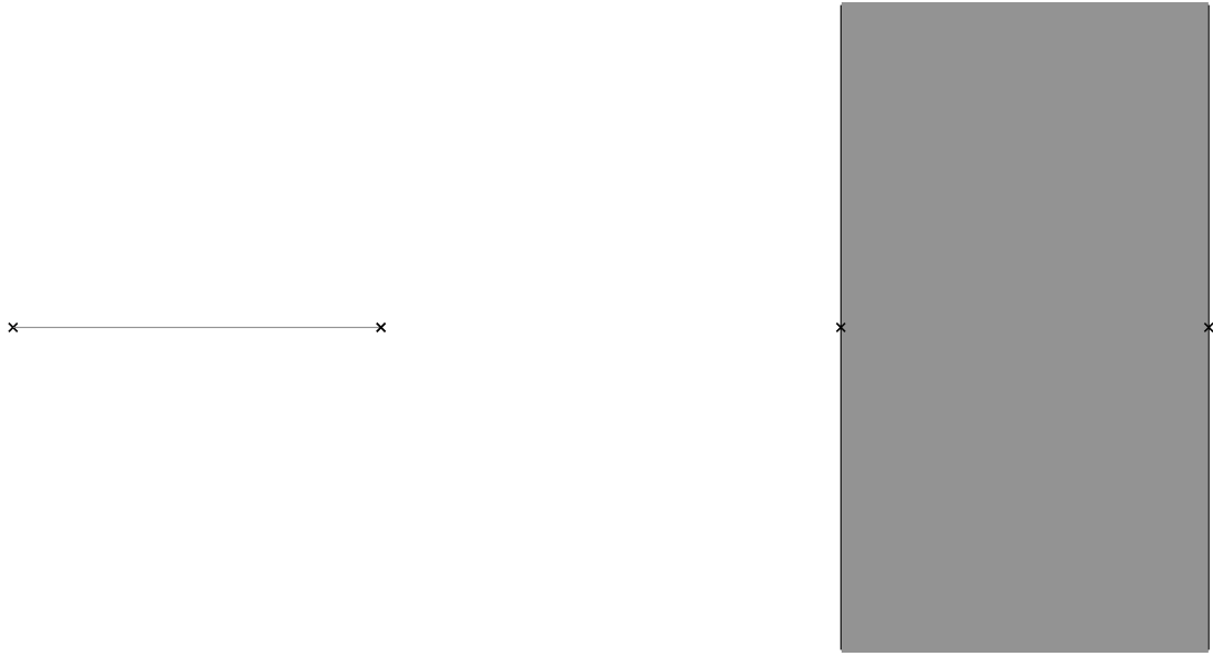
FIGURE 12.4: All points in the grey area are between the two points represented by black crosses: at left, in the sense of R_c , at right, in the sense of R_p .
