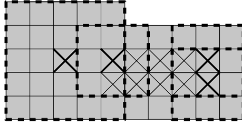
FIGURE 4.2: Example of medial axis in discrete framework. The shape is represented in grey. The medial axis is represented by crosses. Some maximal balls are represented by dashed lines, with their centers represented by bold crosses.
