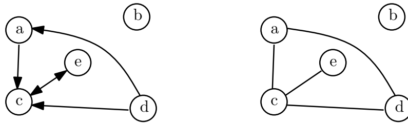
FIGURE 7.4: From the left to the right, a directed graph and its associated undirected graph.
