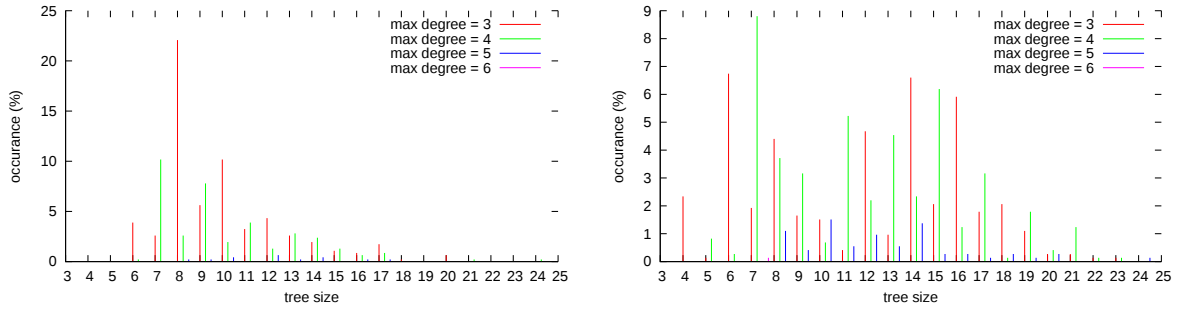
FIGURE 11.11: Average distributions. Left: dancer data set. Right: hand data set.
