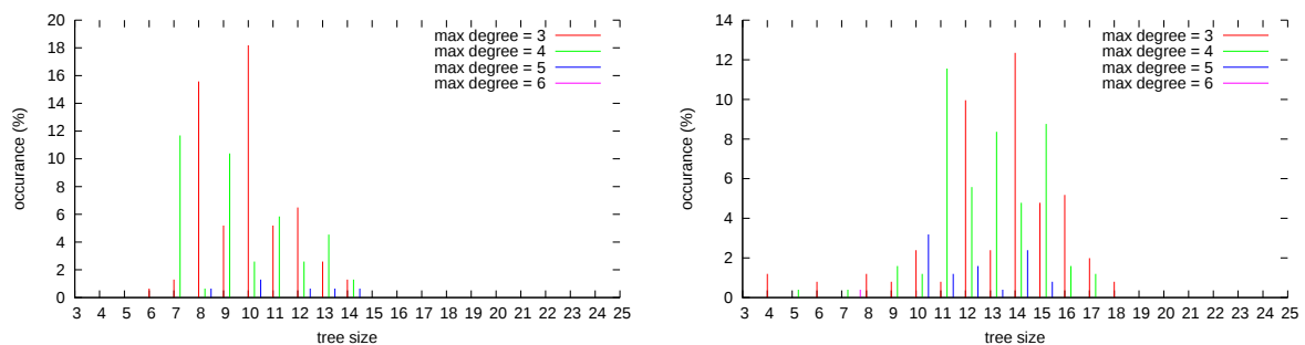
FIGURE 11.9: Distributions for a grid sided by 80. Left: dancer data set. Right: hand data set.
