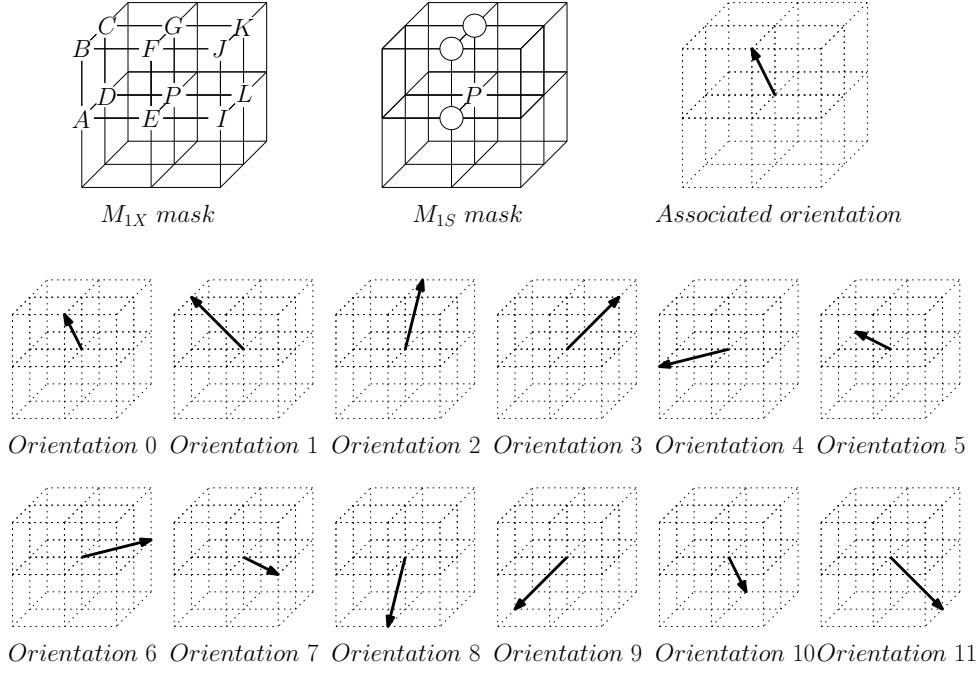
FIGURE 5.6: New masks for 1-crucial points detection, and all possible orientations of these masks.
