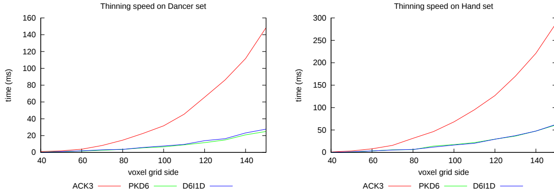
FIGURE 6.4: Thinning speed of fully optimized ACK3, PKD6 and D6I1D on two data sets.
