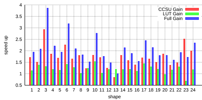
FIGURE 5.12: Speed gain obtained by different optimizations on PKD6.
