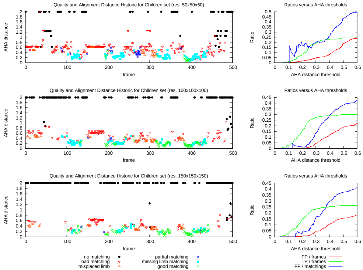
FIGURE 13.5: Study of correlations between AHA distance and matching quality for children data set with different grid resolutions. Left: historic of AHA distances and matching qualities all along the sequence. Right: different ratios in regard of given AHA distance threshold. From top to bottom: for resolutions 50^3 , 100^3 and 150^3 .
