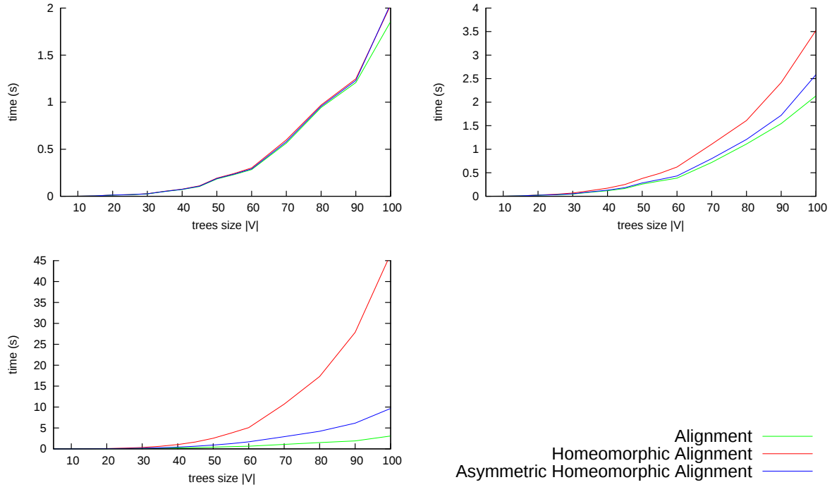
FIGURE 11.7: Computation speed of different alignments for different sizes of trees. Top left: between two rooted trees. Top right: between a rooted tree and an unrooted tree. Bottom left: between two unrooted trees.
