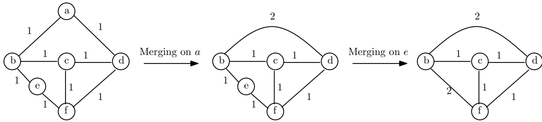
FIGURE 9.2: Examples of merging on undirected graph.
