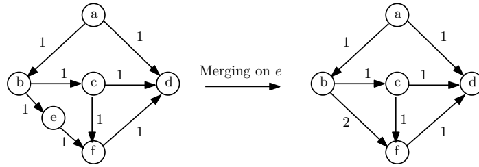
FIGURE 9.1: Example of merging on directed graph.
