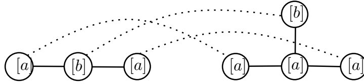
FIGURE 8.8: An invalidate constrained mapping: the center relationship preservation condition is not respected.
