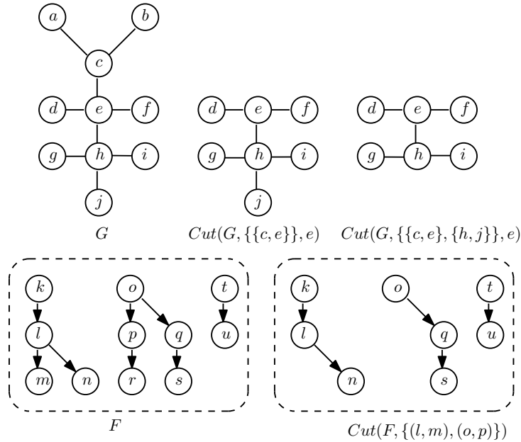
FIGURE 9.9: Examples of cut operations. Top row: on an unrooted tree. Bottom row: on a rooted forest.
