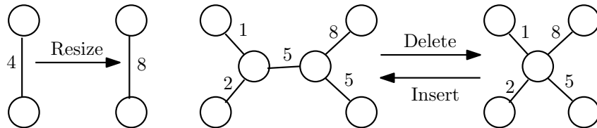
FIGURE 8.2: Examples of edit operations for weighted trees.
