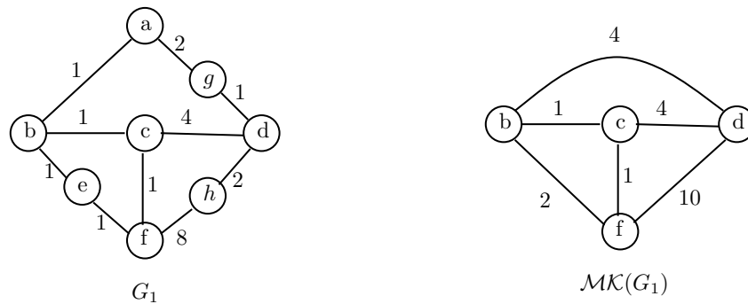
FIGURE 9.4: Example of merging kernel of an undirected graph.
