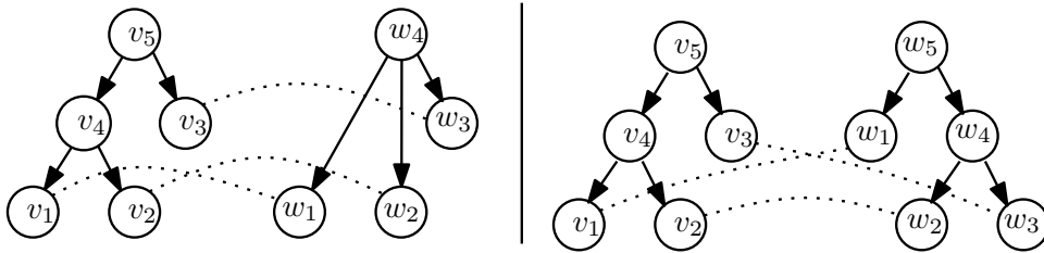
FIGURE 8.9: Left: a mapping which is not constrained but less constrained. Right: a mapping which is not less constrained.
