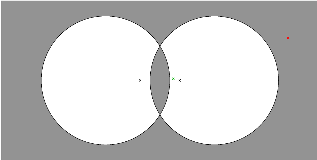
FIGURE 12.6: All points in the grey area are between the two points represented by black crosses (in the sense of R_u ). We can notice that the green cross is between the black ones, in the common conception of betweenness, but is not in the sense of R_u . In the same way, the red cross is not between the black ones, in the common conception of betweenness, but is so in the sense of R_u .
