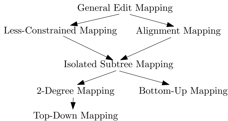
FIGURE 8.12: Hierarchy of mappings.
