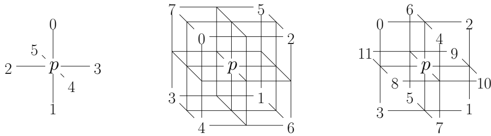
FIGURE 4.9: From the left to the right: Directions used for directional thinning algorithms with 6, 8 and 12 sub-iterations. Each number i represents a voxel which have to be out of the object to allow the deletion of p in the i th sub iteration.
