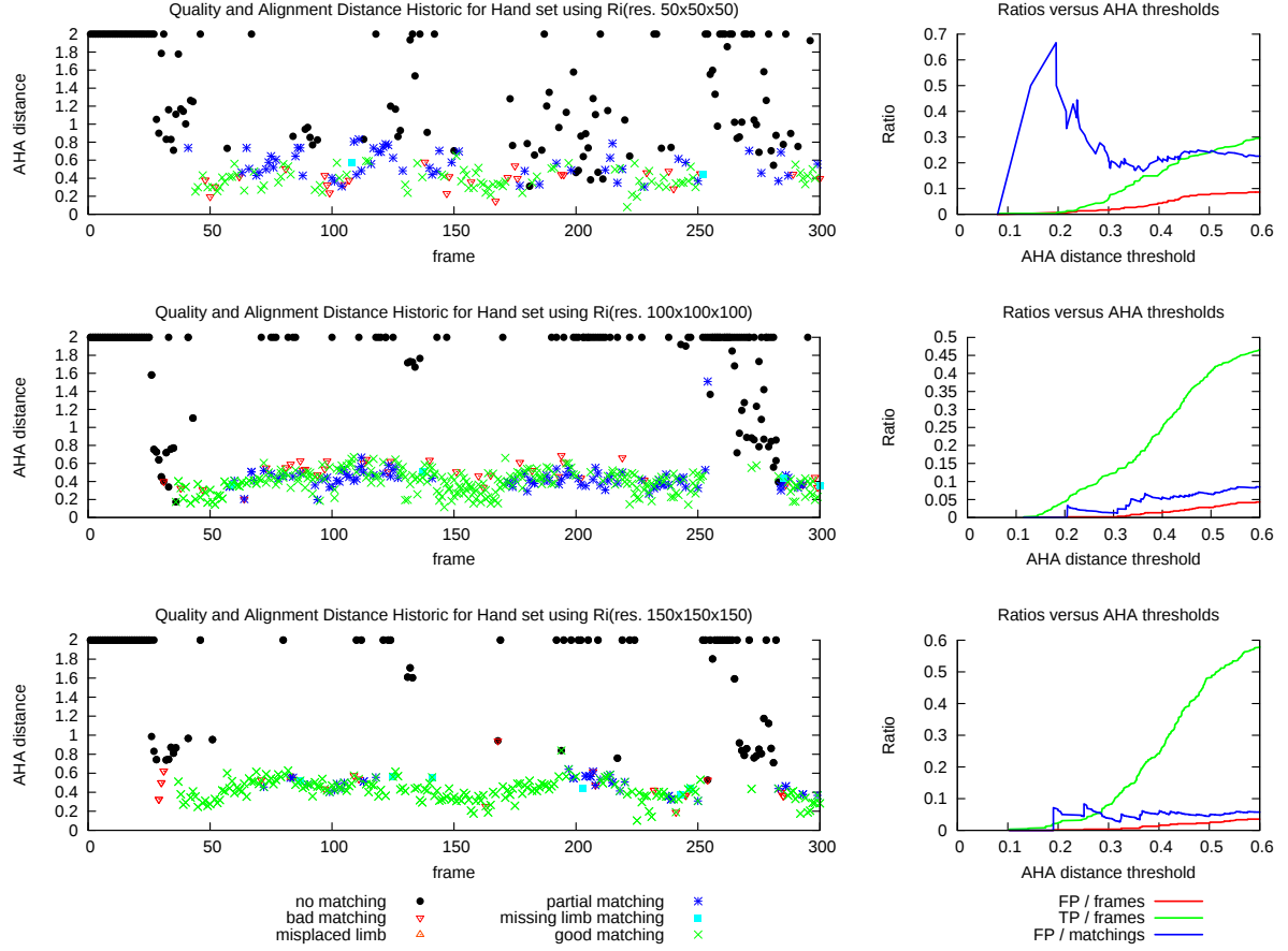
FIGURE 13.7: Study of correlations between AHA distance and matching quality for hand data set with different grid resolutions, using betweenness relation R_i . Left: historic of AHA distances and matching qualities all along the sequence. Right: different ratios in regard of given AHA distance threshold. From top to bottom: for resolutions 50^3 , 100^3 and 150^3 .
