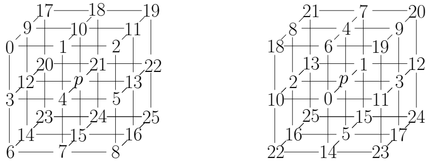
FIGURE 5.1: Left: an order optimized for reducing amount of cache miss. Right: an order useful for algorithms using several look-up tables for different neighborhoods.
