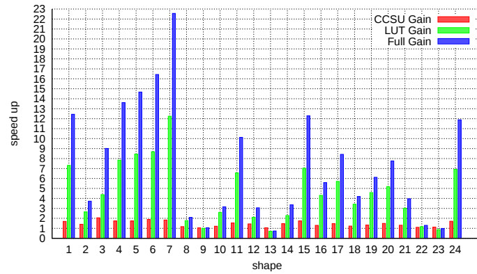
FIGURE 5.11: Speed gain obtained by different optimizations on ACK3.
