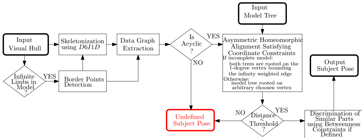
FIGURE 12.8: Complete pipeline of our method. Rounded rectangles represent input and output data. Other rectangles represent steps of the method.
