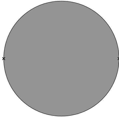
FIGURE 12.5: All points in the grey area are between the two points represented by black crosses, in the sense of R_b .
