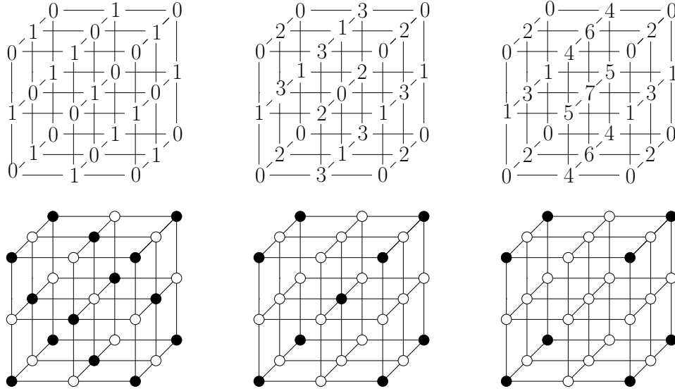
FIGURE 4.10: Top, from the left to the right: Divisions of \mathbb{Z}^3 into 2, 4 and 8 subfields. For an algorithm using k subfields, in a i th sub iteration, only points marked i will be considered. Bottom, from the left to the right: black points represent considered points in the first iteration of a k -subfield based algorithm, for k = 2, 4, 8 .
