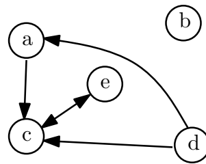
FIGURE 7.3: Example of directed graph representation. The circles represent the vertices, and the arrows represent the arcs. The represented graph is (V = \{a, b, c, d, e\}, E = \{(a, c), (d, a), (d, c), (c, e), (e, c)\}) .
