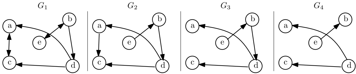
FIGURE 7.5: From the left to the right, four directed graphs: G_1, G_2, G_3 and G_4 . G_1 have two roots ( b and e ), G_2 and G_3 have only one root ( e ) and G_4 have no root. G_2, G_3 and G_4 are antisymmetric, contrary to G_1 . G_3 is a rooted tree, contrary to the three others. G_3 and G_4 are rooted forests, composed respectively by one and two rooted trees.
