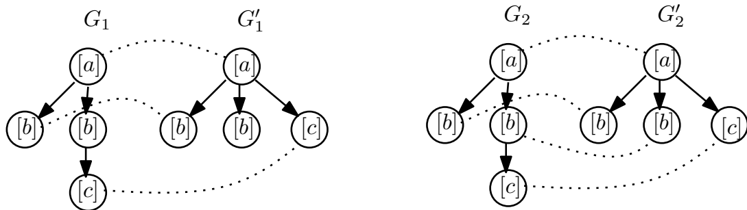
FIGURE 8.3: Left: A mapping from G_1 to G'_1 . The dotted lines represent the mapping. Vertices in G_1 not touched by a mapping line have to be deleted. Vertices in G'_1 not touched by a mapping line have to be inserted. The mapping shows a way to transform G_1 to G'_1 . Right: An invalidate mapping from G_2 to G'_2 : the ancestor condition is not respected.
