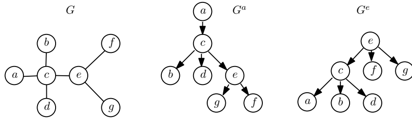
FIGURE 9.8: A tree G and the rooted trees G^a and G^e .
