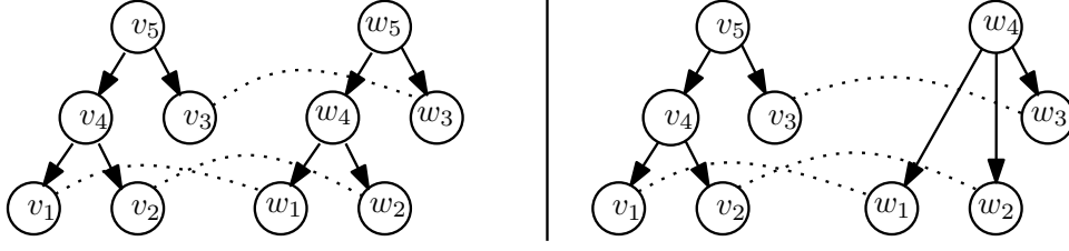
FIGURE 8.6: Left: a mapping which is constrained. Right: a mapping which is not constrained.
