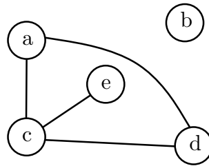
FIGURE 7.1: Example of undirected graph representation. The circles represent the vertices, the letter in each circle is just used in a purpose of easily identify the associated vertex, and the lines represent the edges. The represented graph is (V = \{a, b, c, d, e\}, E = \{\{a, c\}, \{a, d\}, \{c, d\}, \{c, e\}\}) .
