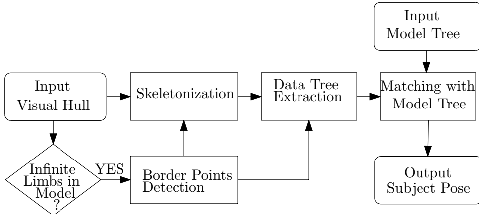
FIGURE 3.4: Pipeline of our method. Rounded rectangles represent input and output data. Other rectangles represent steps of the method.
