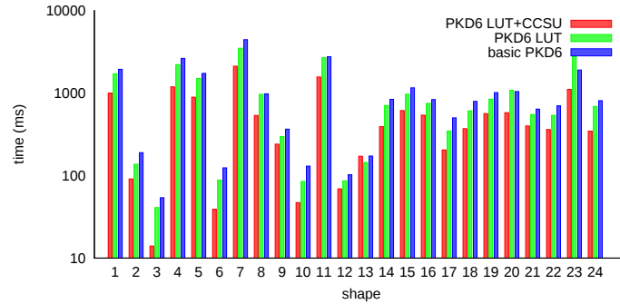
FIGURE 5.10: Computation speed results for PKD6 implemented with different levels of optimization, for each image of our test set.
