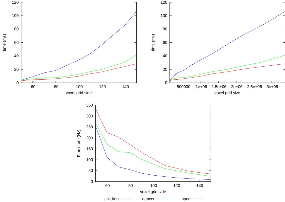
FIGURE 13.2: Speed results for three different data sets: children , dancer and hand . On top, average speed computation for one frame, for different sizes of voxel grid: on the left, in regard of the number of voxels per side of the voxel grid; on the right, in regard of the number of voxels of voxel grid. On bottom: average frame rate in regard of the number of voxels per side of the voxel grid.
