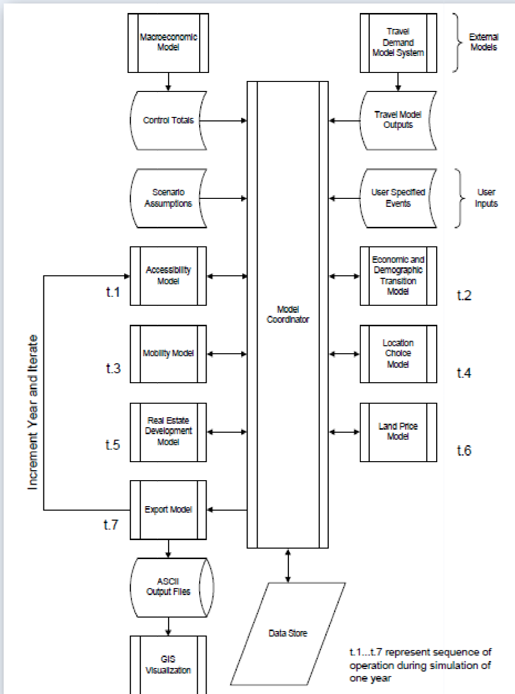
FIGURE 50: MODULAR ARCHITECTURE OF URBANSIM
