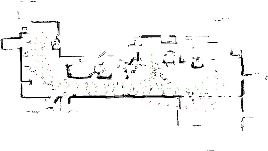
Figure 3.14: Global map obtained by SLAM together with the original and recomputed position of the robot at several key instants.
