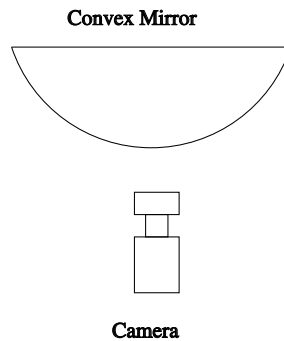
Figure 2.17: Construction of a Catadioptric System
