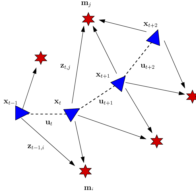
Figure 2.1: Notations for the SLAM problem [ Mei (2007) ]
