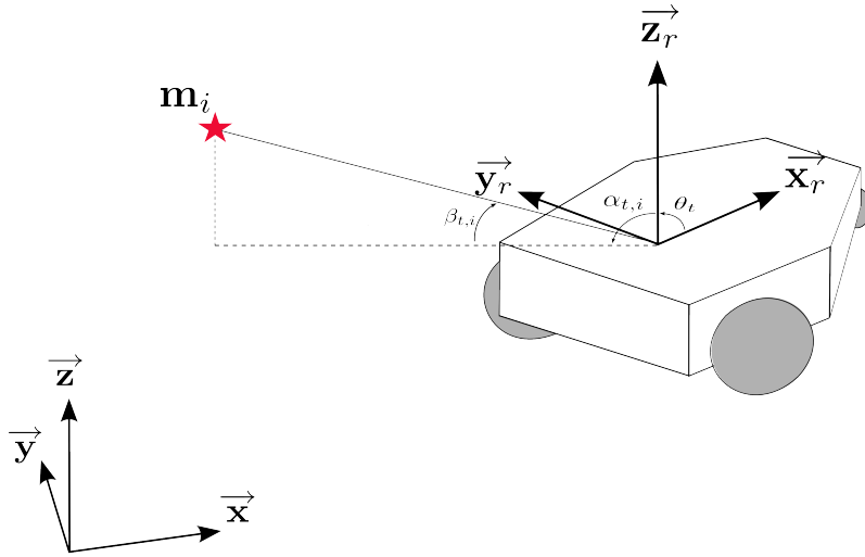
Figure 2.2: Bearing-Only SLAM
