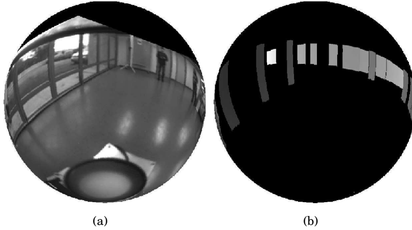
Figure 5.2: Augmented spherical view: at each pixel on the unit sphere is associated with a grey level intensity and the corresponding depth of the 3D point. 5.2(a) Grey levels on the unit sphere. 5.2(b) Depth spherical image.
