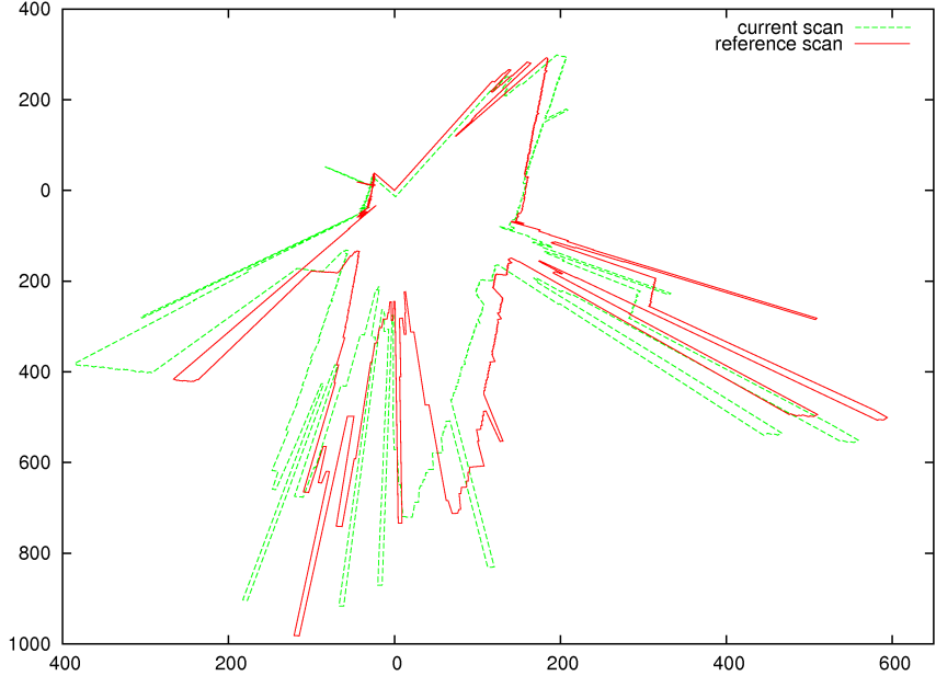
Figure 3.7: Real scans: current scan (green) and reference scan (red) prior to matching
