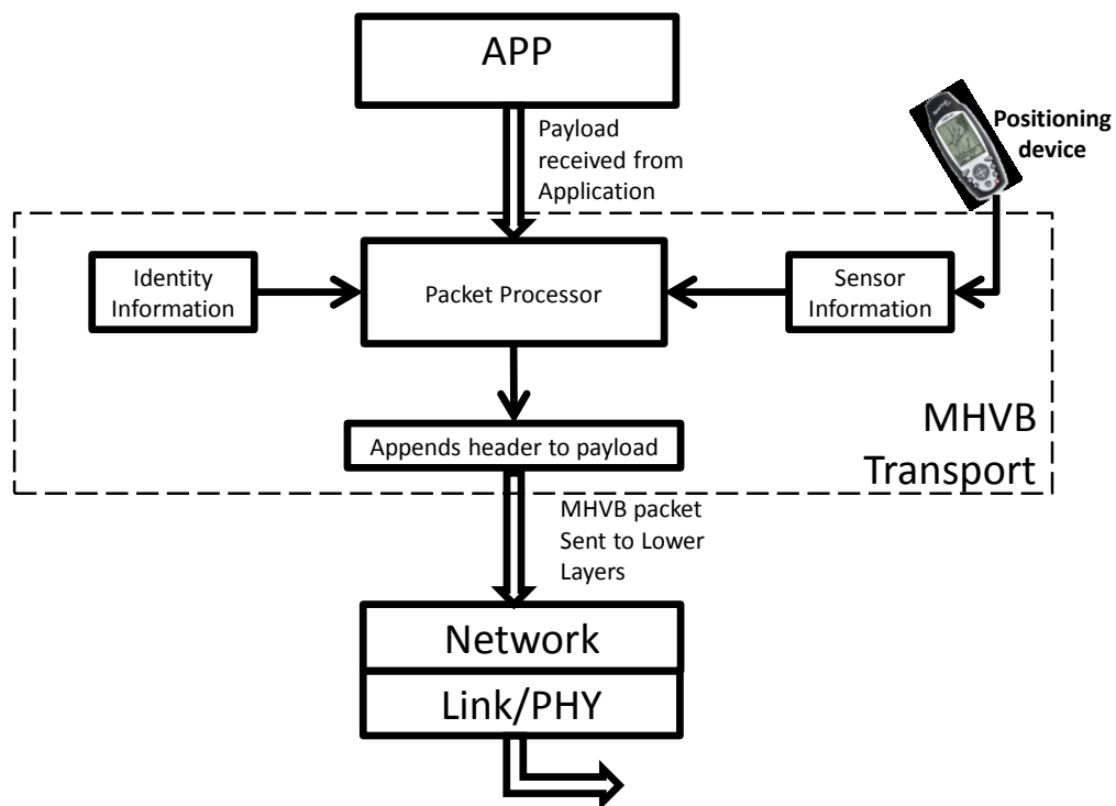
Figure 4.2: Packet Transmission
