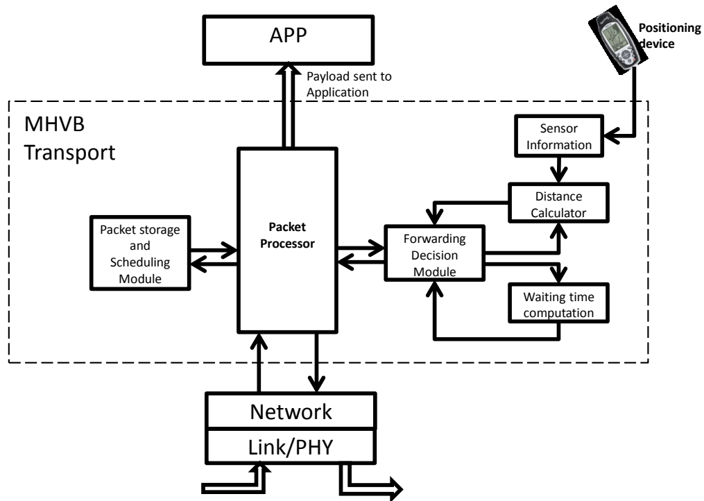
Figure 4.3: Packet Processing and forwarding
