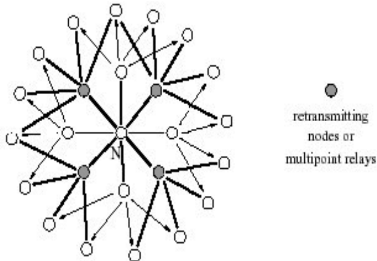
Figure 1.1: Multi-point relay
